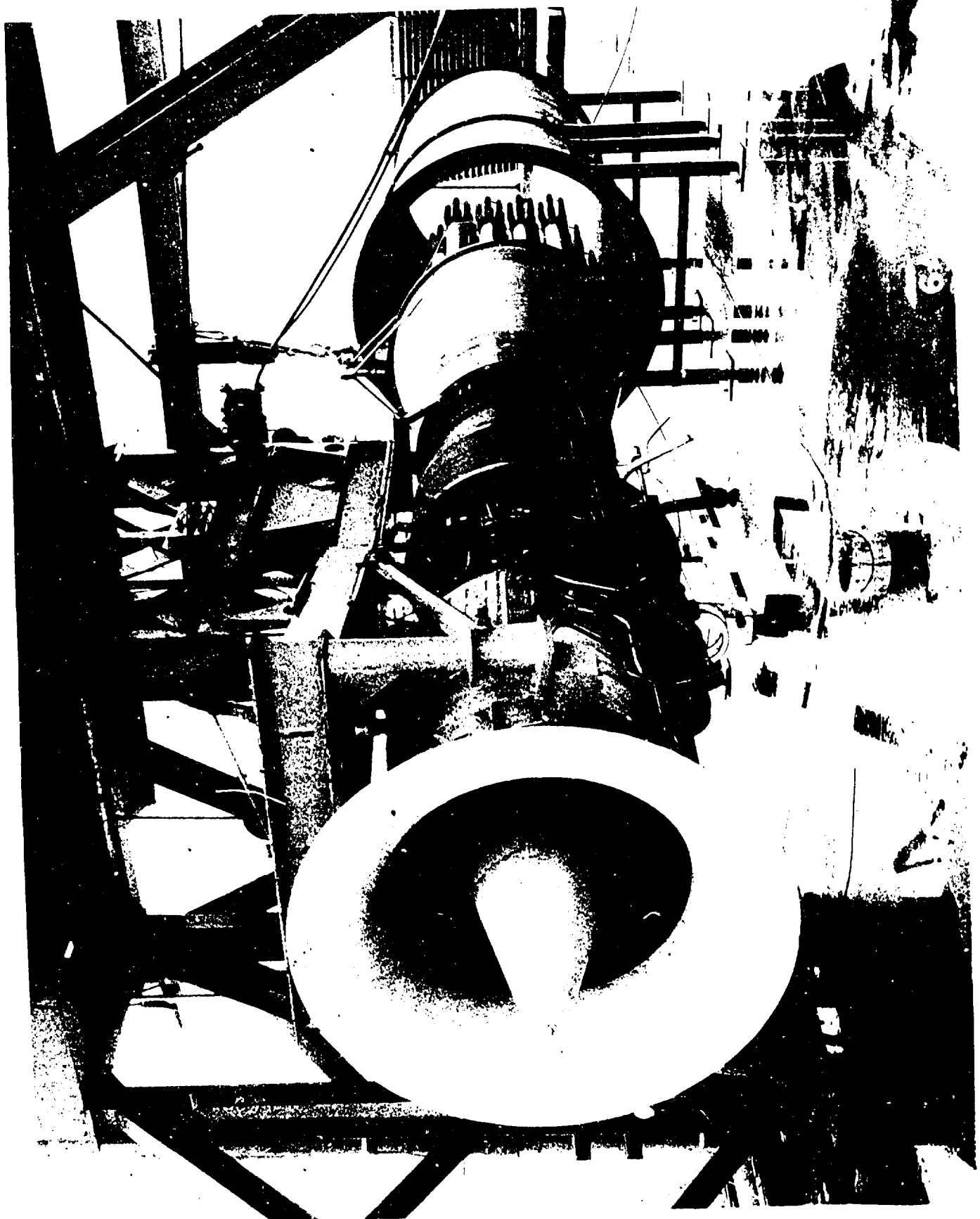
25'-TUBE MIXING NOZZLE - 10" DIA. - 12" THICK WITH 12 FT. ACoustically LINED DUCT
