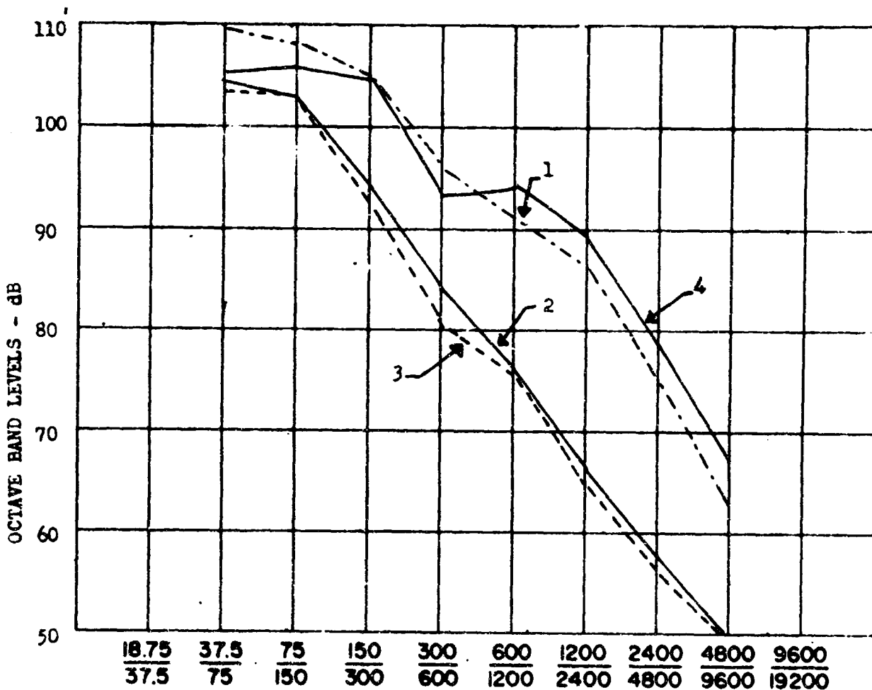
Frequency band in cps UNSUPPRESSED AND SUPPRESSED JET NOISE SPECTRA - 1500 FT. SIDELINE
