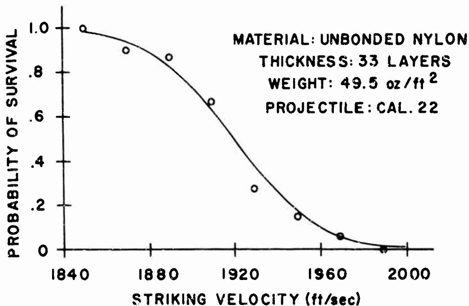
PROBABILITY OF SURVIVAL (NON-PENETRATION) VERSUS STRIKING VELOCITY
