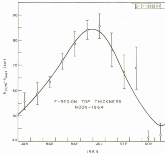
Fig. 14. Seasonal variation of the thickness parameter h_{70\%} - h_{max} .
