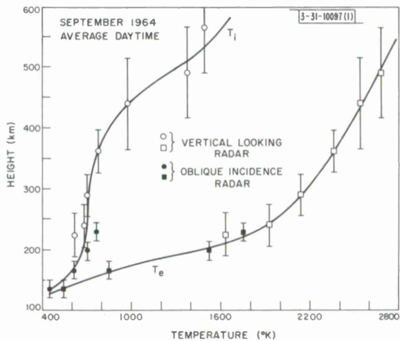
Fig. 26. Average daytime (0900 to 1500 hours) temperature curves obtained with 23- and 68-cm systems.
