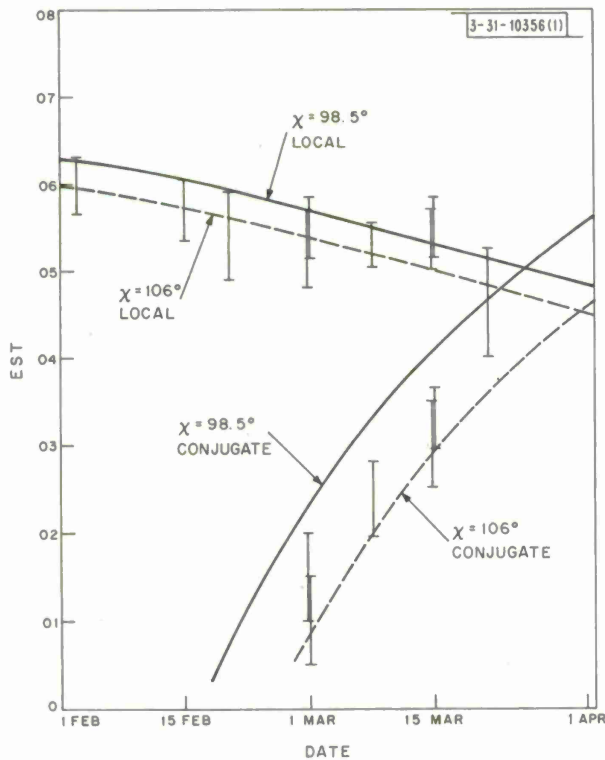
Fig. 19. Times at which local and conjugate sunrise heating appears to commence (Fig. 18). Time at which sun's zenith distance is 106^\circ and 98.5^\circ is also indicated. These two angles correspond to earth's shadow, reaching 200 and 100km, respectively.
