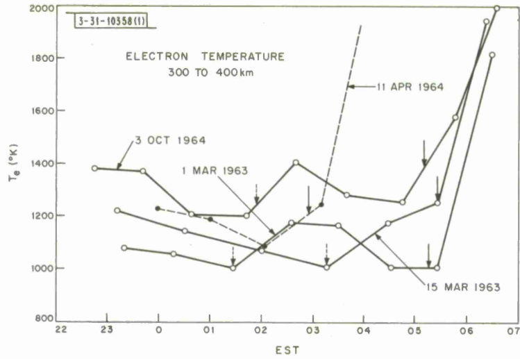
Fig. 18. Variation of T_e showing predawn increases coincident with conjugate sunrise. Solid arrows indicate time of onset of local heating as estimated from \Delta T_e/dt and broken arrows indicate time at which conjugate point heating commences.
