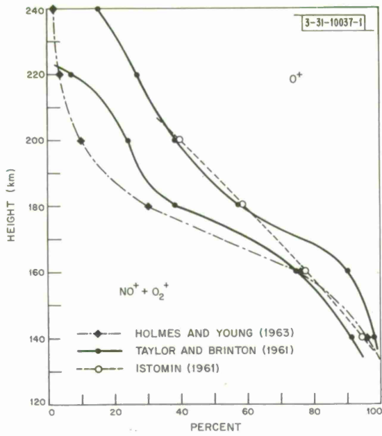
Fig. 20. Rocket profiles of relative abundance of O^+ and sum of O_2^+ and NO^+ ions by three workers.
