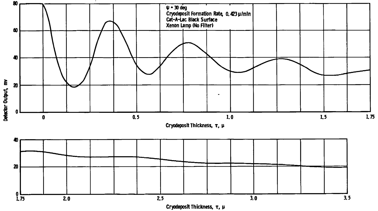
Fig. 13 Bragg Interference Patterns with a White-Light Source
