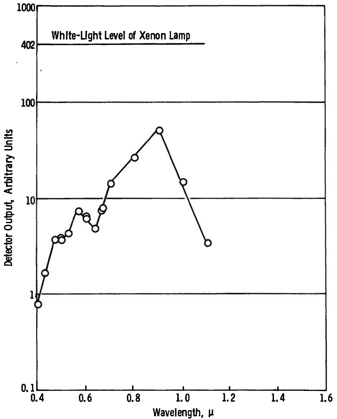
Fig. 3 Composite Spectrum of the Light Source and Detector Systems
