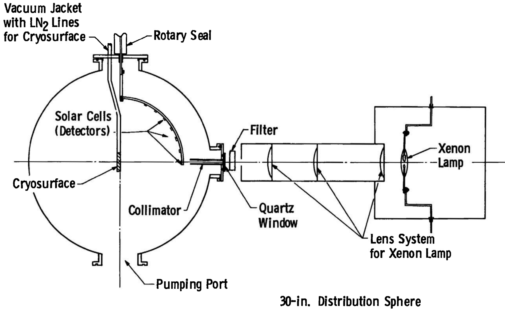
Fig. 2 Schematic of Optical System
