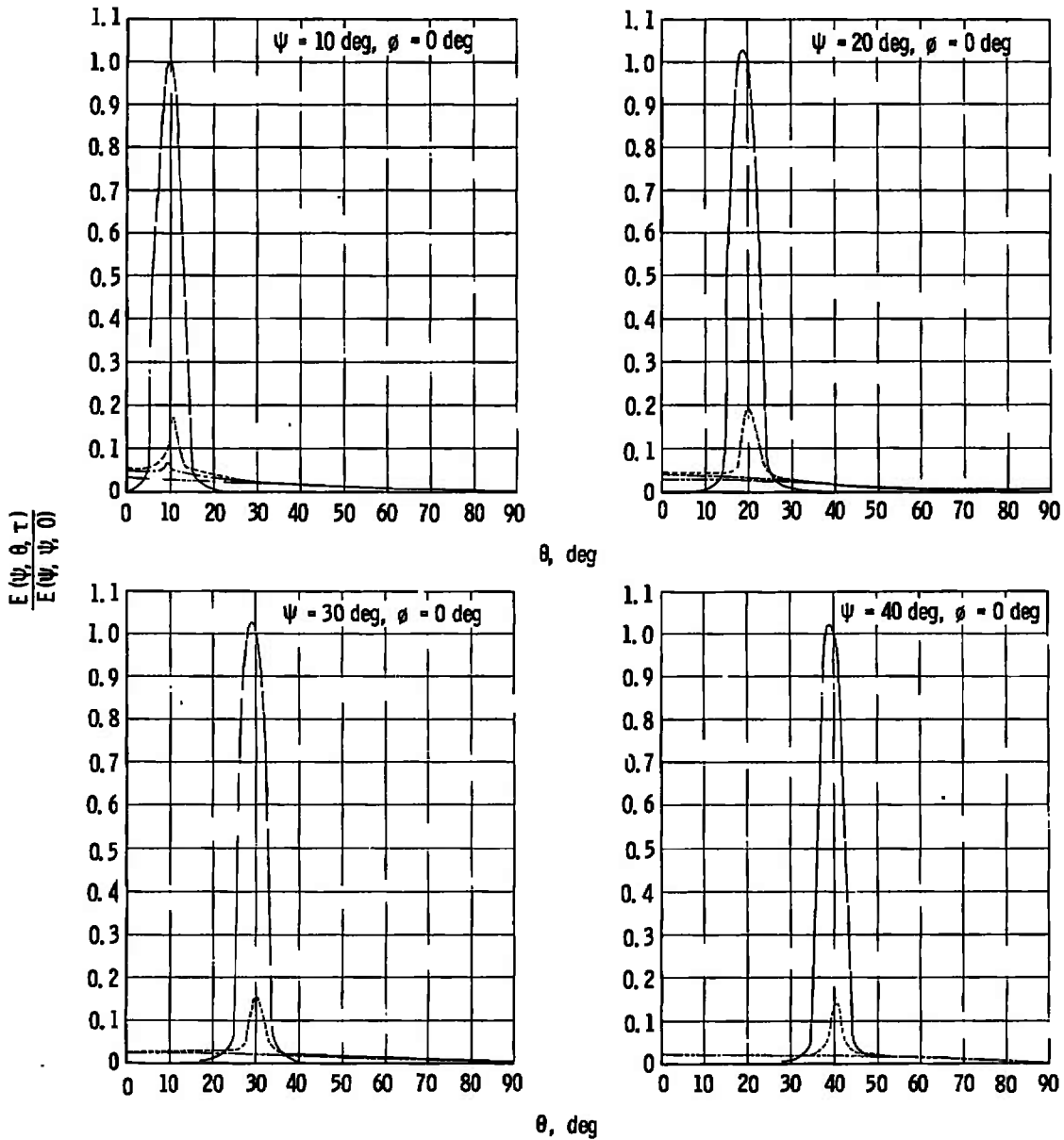
Fig. 7 Normalized Distribution of Light Reflected from CO 2 Cryodeposits Formed at Various Thicknesses on a Polished Copper Substrate at a Rate of 0.423 \mu/\text{min}
