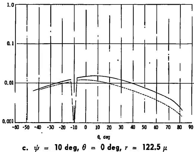
Fig. 19 Comparison of the Distribution of Light Reflected by CO 2 Cryodeposits Formed on a Polished Copper Surface with and without an Oil Frost Sublayer
