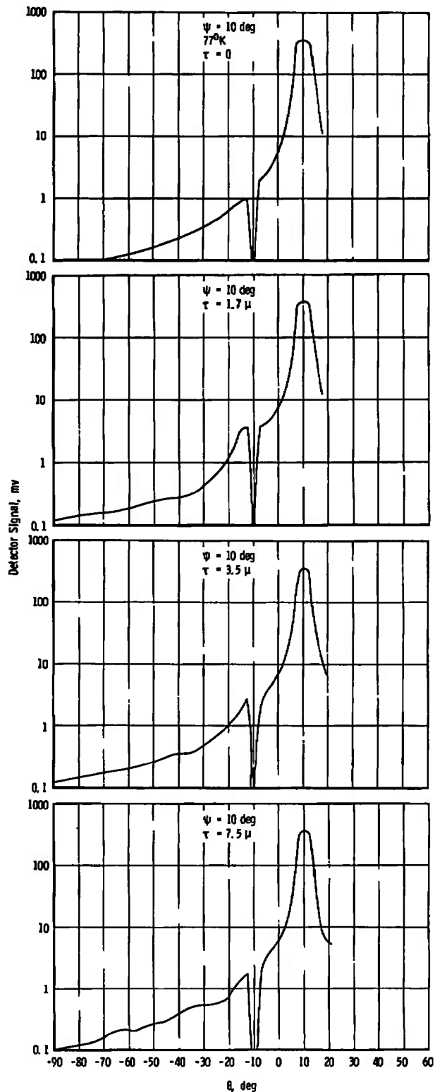
Fig. 8 Distribution of Light Reflected from CO 2 Cryodeposits Formed at Various Thicknesses on a Polished Copper Substrate at a Rate of 0.0385 \mu /min and with \phi = 0 deg
