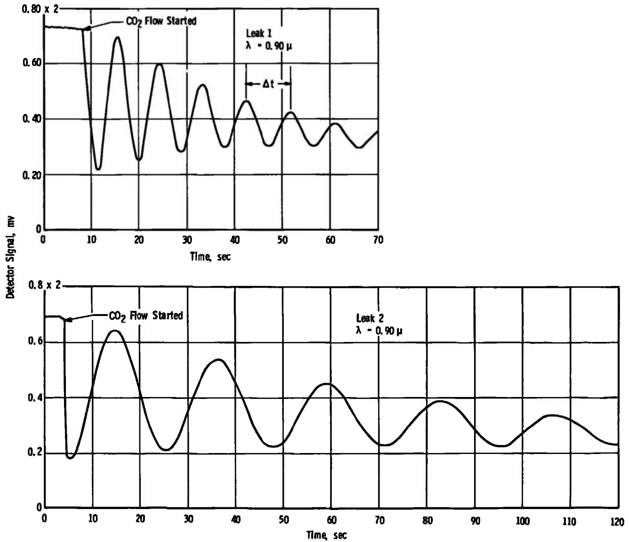
Fig. 5 Typical Bragg Interference Patterns for a Black Substrate
