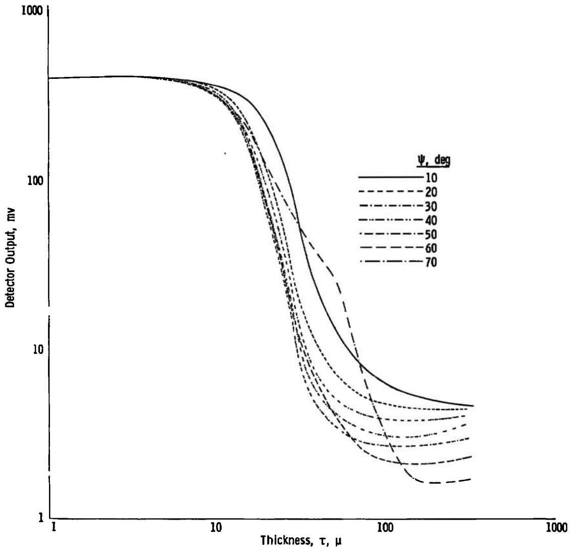
Fig. 15 Variation of Reflected Energy at Specular Angle from CO 2 Cryodeposits Formed at 2.25 \mu /min on a Polished Copper Substrate
