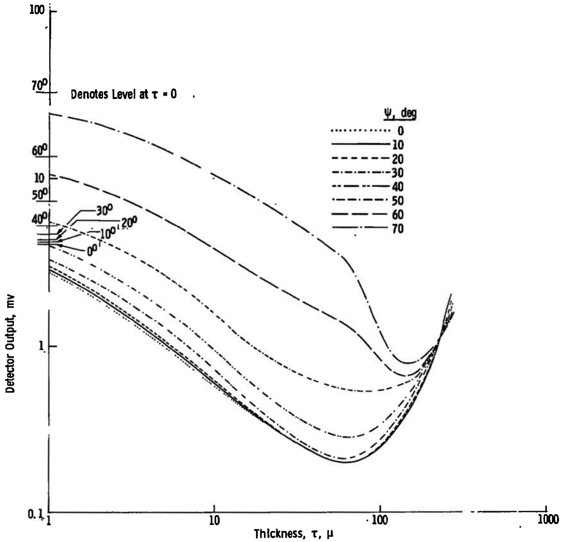
Fig. 16 Variation of Reflected Energy at Specular Angle from CO 2 Cryodeposits Formed at 2.25 \mu /min on a Black Epoxy Painted Substrate
