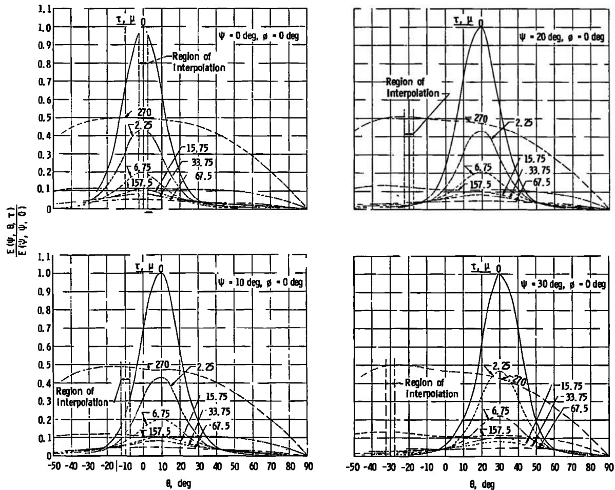
Fig. 9 Normalized Distribution of Light Reflected from CO 2 Cryodeposits Formed at Various Thicknesses on a Black Epoxy Painted Substrate at a Rate of 2.25 \mu /min and with \phi = 0 deg
