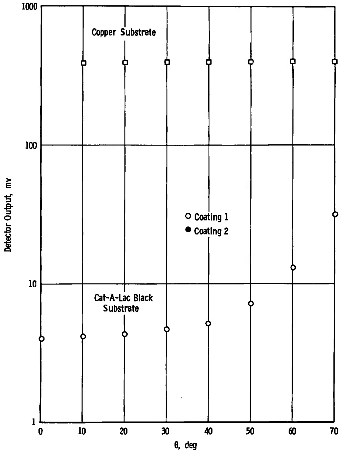
Fig. 12 Detector Output at \theta = \psi for a 300°K Surface without Cryodeposit Used to Normalize Data
