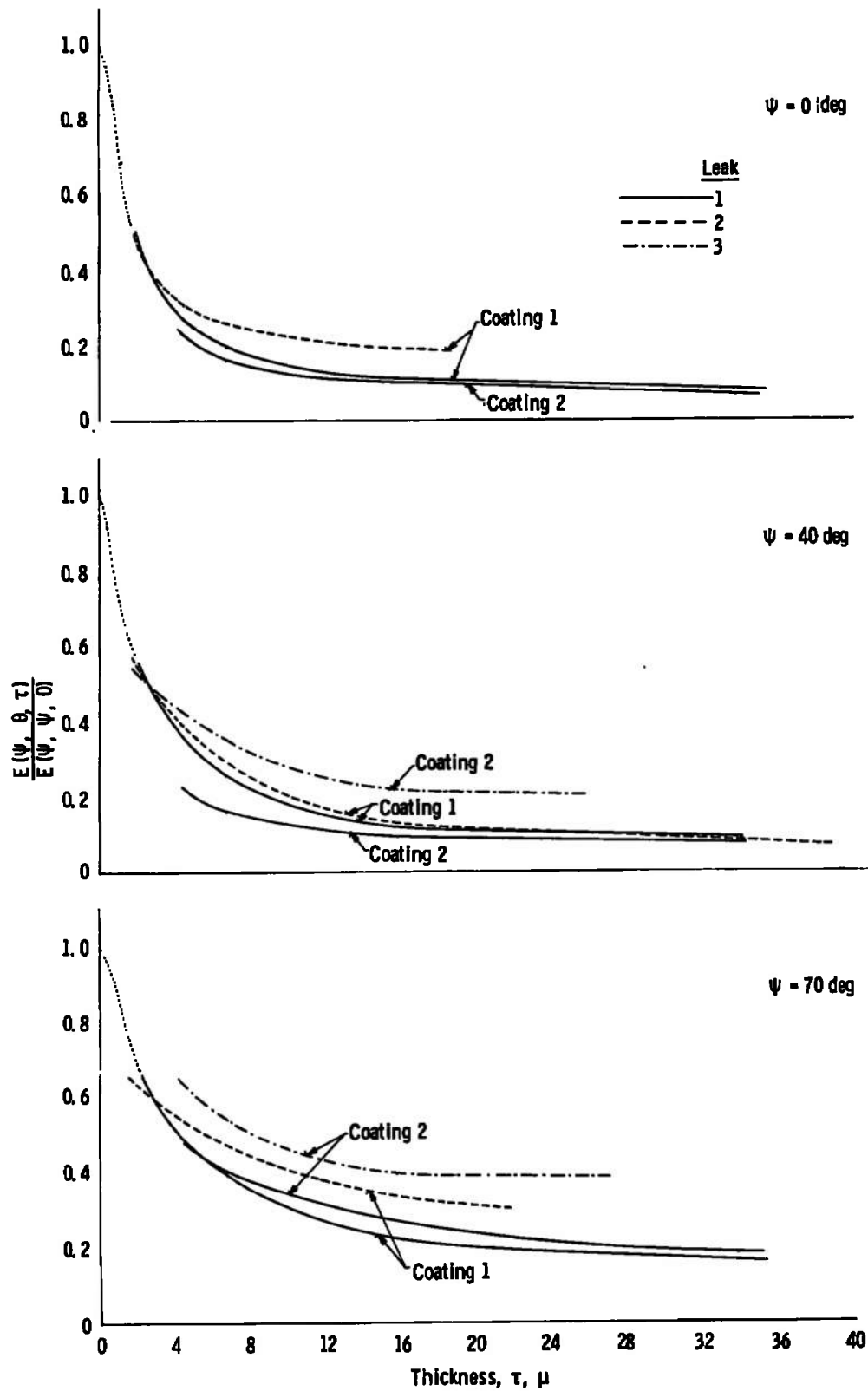
Fig. 14 Variation of Normalized Reflected Energy Output at Specular Angle for Various \text{CO}_2 Cryodeposits Formed on Two Different Cat-A-Lac Black Surfaces
