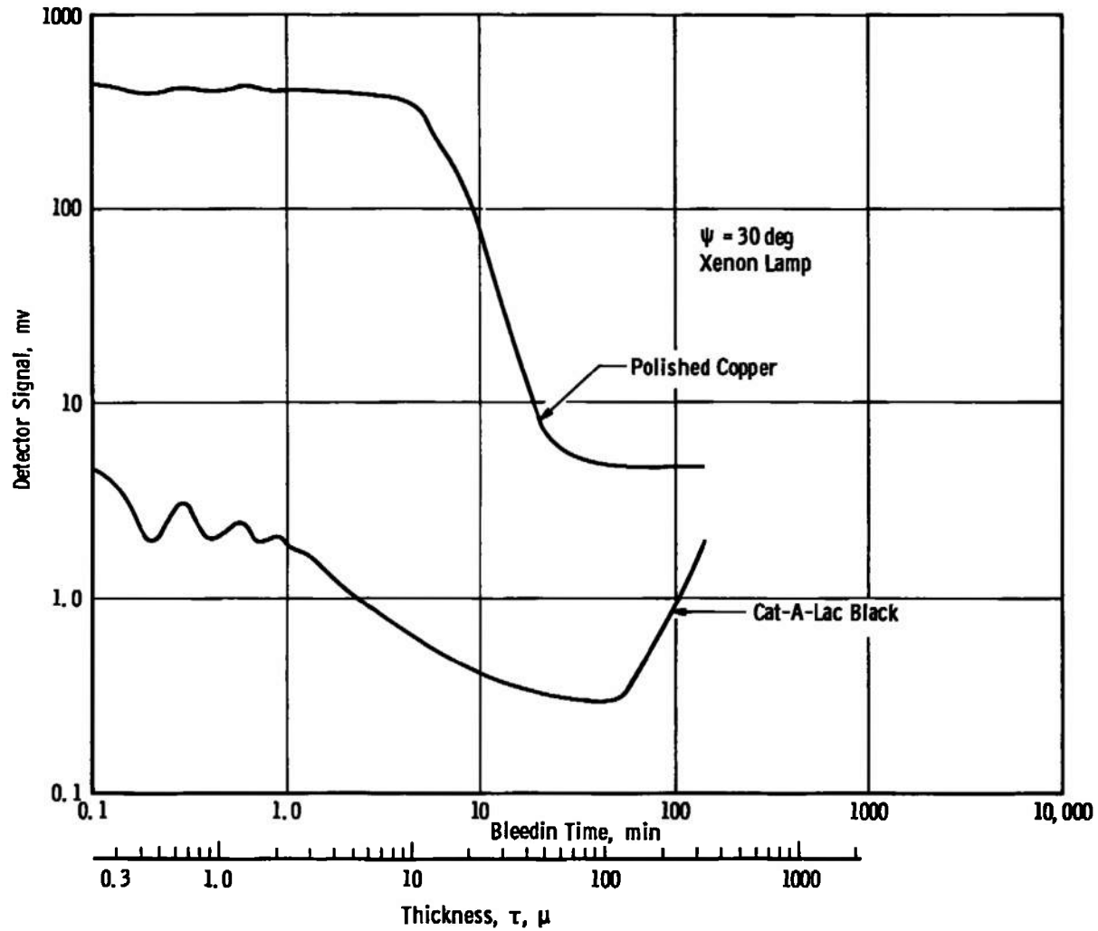
Fig. 17 Comparison of Light Reflected from \text{CO}_2 Cryodeposits on Polished Copper and Black Epoxy Painted Substrates at the Specular Angle of Reflection
