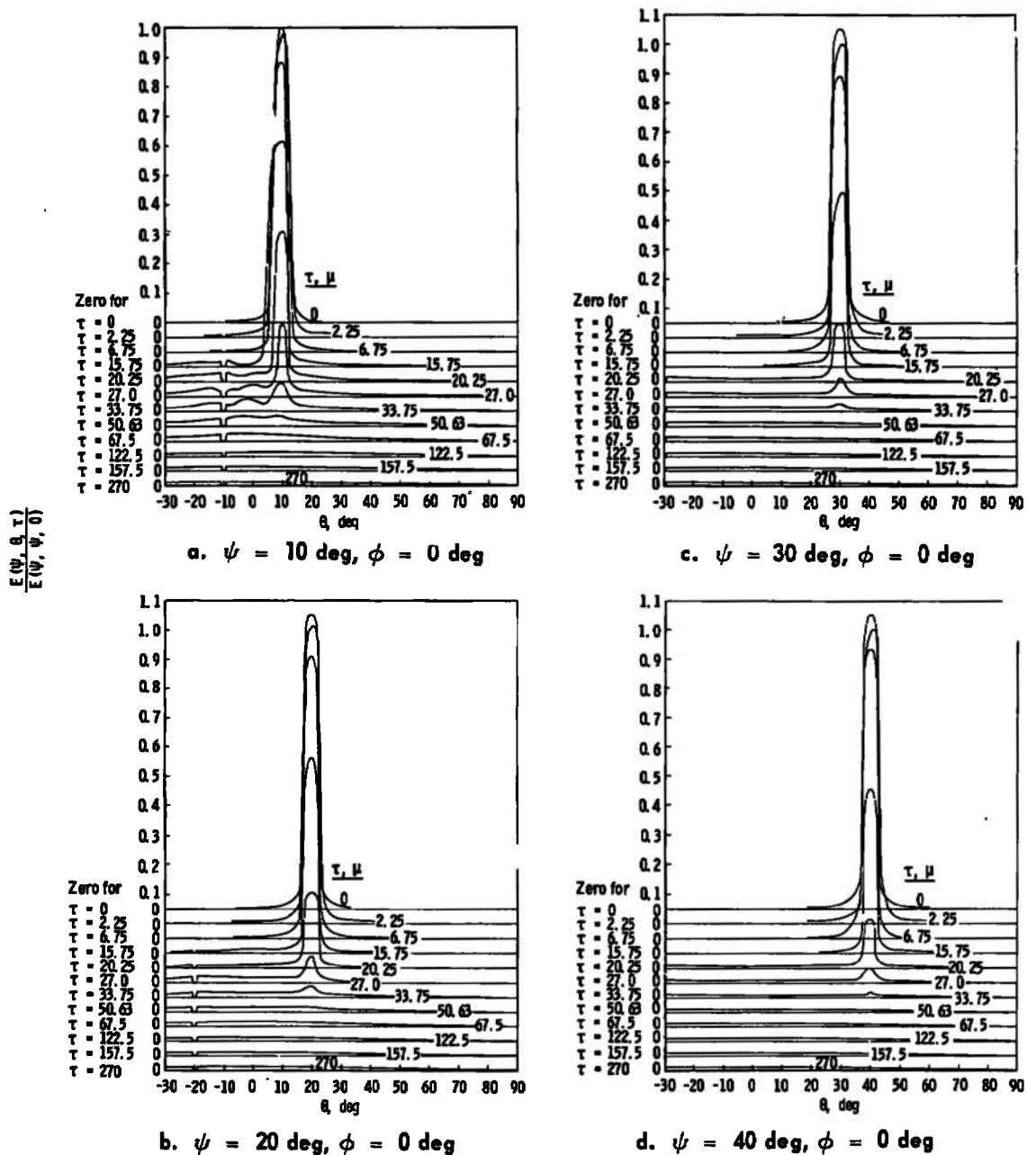
Fig. 6 Normalized Distribution of Light Reflected from CO 2 Cryodeposits Formed at Various Thicknesses on a Polished Copper Substrate at a Rate of 2.25 μ/min
