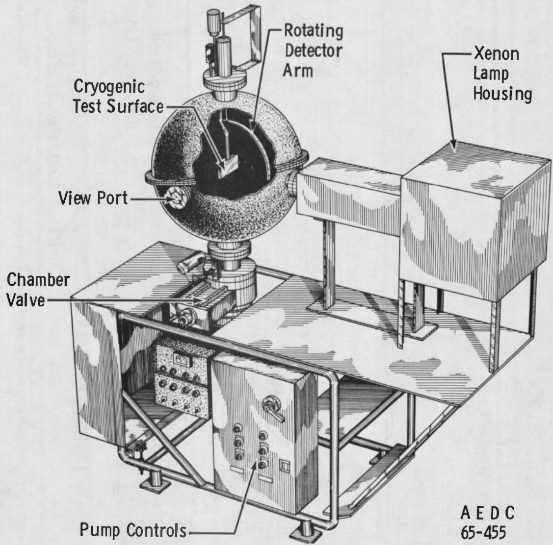
Fig. 1 Schematic of Test Apparatus
