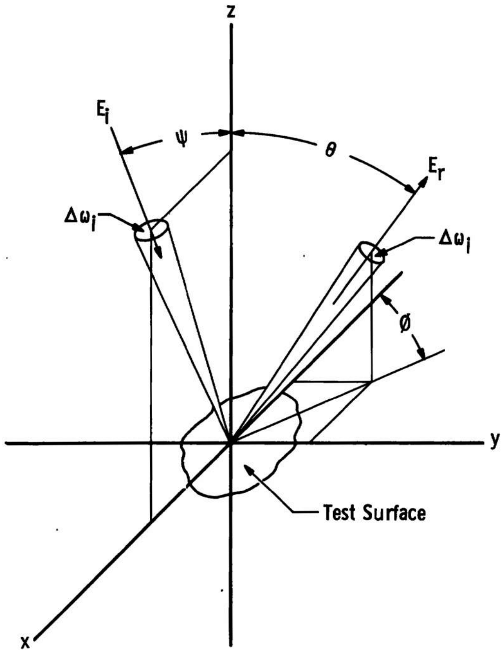
Fig. 4 Notation Pertinent to Biangular Distribution Measurements
