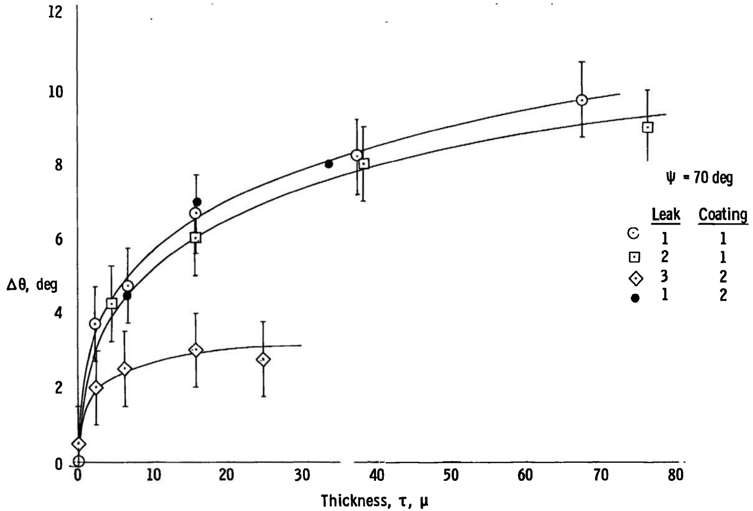
Fig. 18 Angular Shift of the Specular Component of Light Reflected from \text{CO}_2 Cryodeposits Formed at Various Rates on a Black Epoxy Painted Substrate
