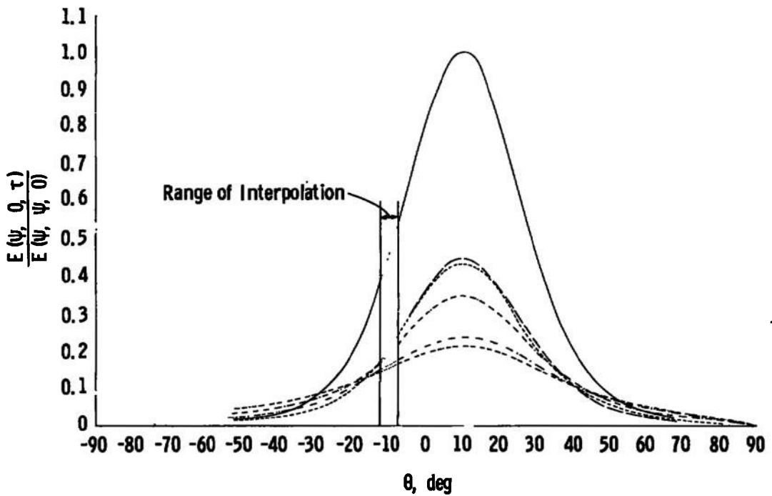
Fig. 11 Normalized Distribution of Light Reflected from CO 2 Cryodeposits Formed at Various Thicknesses on a Block Epoxy Painted Substrate at a Rate of 0.0385 \mu /min and with \phi = 0 deg
