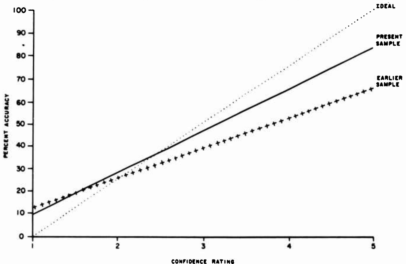
Figure 5. Comparison of the regressions of confidence on accuracy for both samples with the ideal regression
