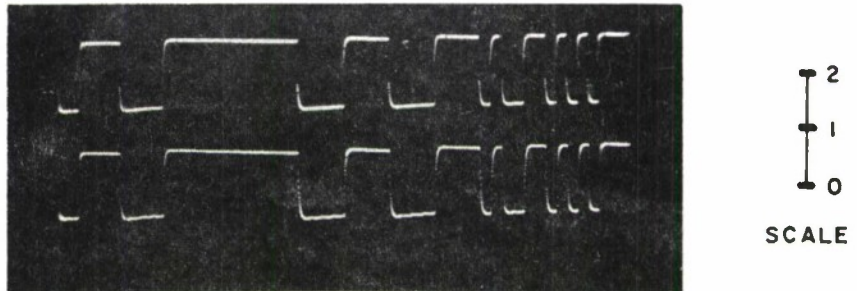
FIGURE 11. - POLAR NRZ SIGNAL TRANSMITTED AT 2400 BITS/SECOND OVER A 1 MILE 22AWG NON-LOADED LINE (VERTICAL SCALE - 2 VOLTS/DIVISION, HORIZONTAL SCALE - 2 MILLISECONDS/DIVISION)
