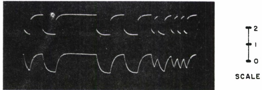
FIGURE 15. - POLAR NRZ SIGNAL TRANSMITTED AT 2400 BITS/SECOND OVER A 5 MILE 19AWG NON-LOADED LINE (VERTICAL SCALE - 2 VOLTS/DIVISION, HORIZONTAL SCALE - 2 MILLISECONDS/DIVISION)
