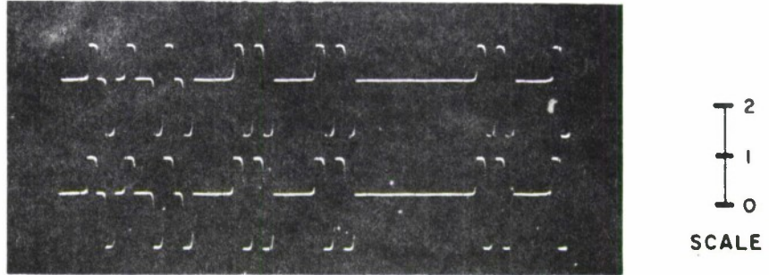
FIGURE 18. - BIPOLAR NRZ SIGNAL TRANSMITTED AT 2400 BITS/SECOND OVER A 1 MILE 22AWG NON-LOADED LINE (VERTICAL SCALE - 2 VOLTS/DIVISION, HORIZONTAL SCALE - 2 MILLISECONDS/DIVISION)
