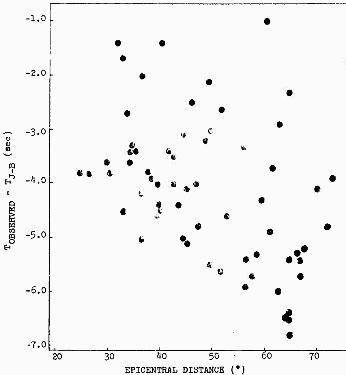
FIG. 14. Long Shot travel time residuals at North American stations as a function of epicentral distances. Values used are listed in Tables 9 and 10.
