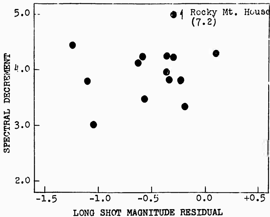
FIGURE 21. Long Shot spectral decrements versus magnitude residuals.
