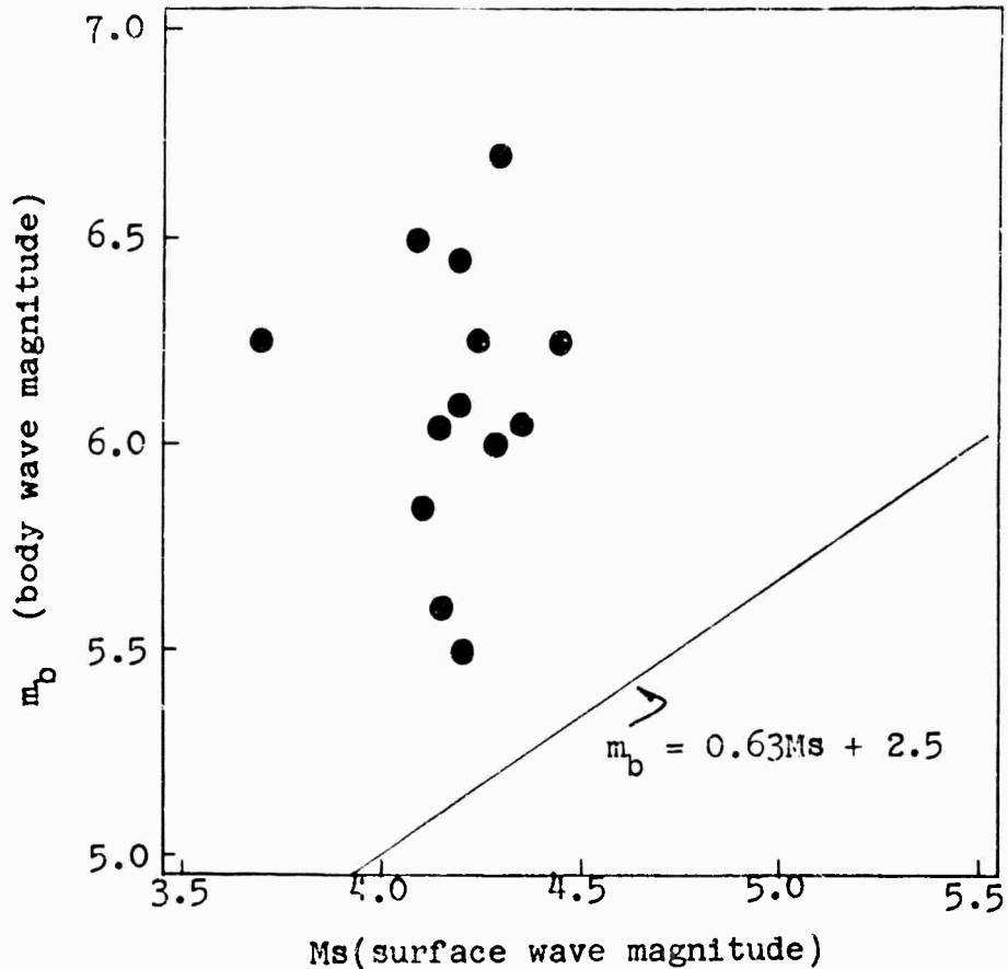
FIG. 13. Long Shot body wave magnitude versus surface wave magnitude at Canadian stations. curve ( m_b = 0.63M_s + 2.5 ) from Gutenberg and Richter (1956). Body wave magnitudes from Jensen et al (1966).
