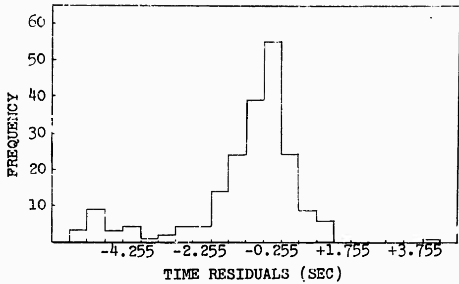
FIG. 16. Histogram of earthquake travel time residuals at Penticton
