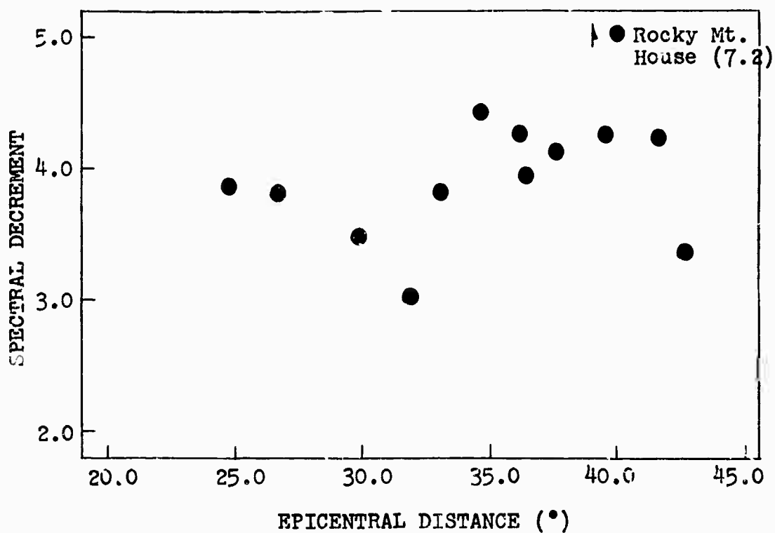
FIGURE 22. Long Shot spectral decrements versus epicentral distance.
