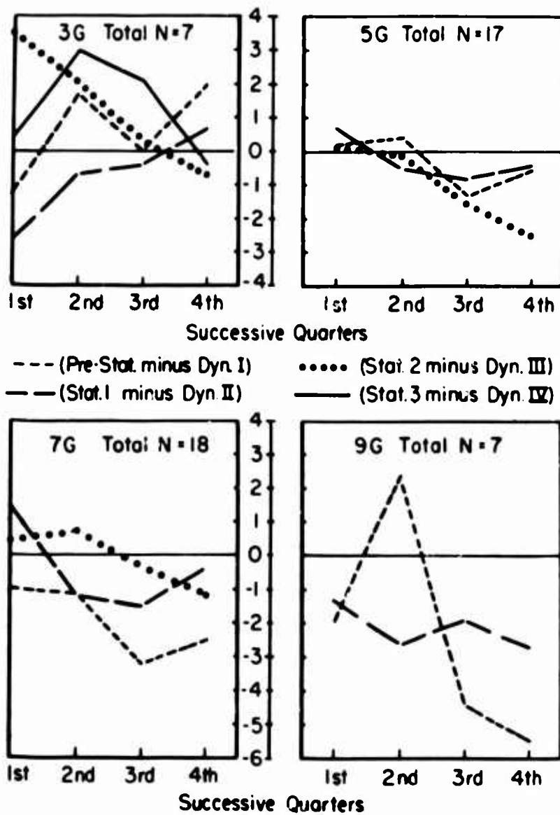
Figure 29. Successive quarters scores for 3, 5, 7, and 9 G x , showing performance on immediate memory task. (Ross, Chambers, and Thompson, 1965)
