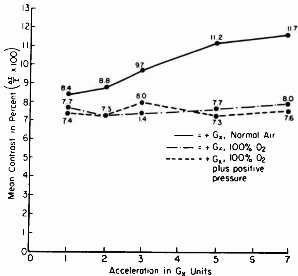
Figure 36. Comparison of effects of breathing normal air, 100% oxygen, and 100% oxygen plus positive pressure, on brightness contrast requirements (As measured on the AMAL Human Centrifuge)
