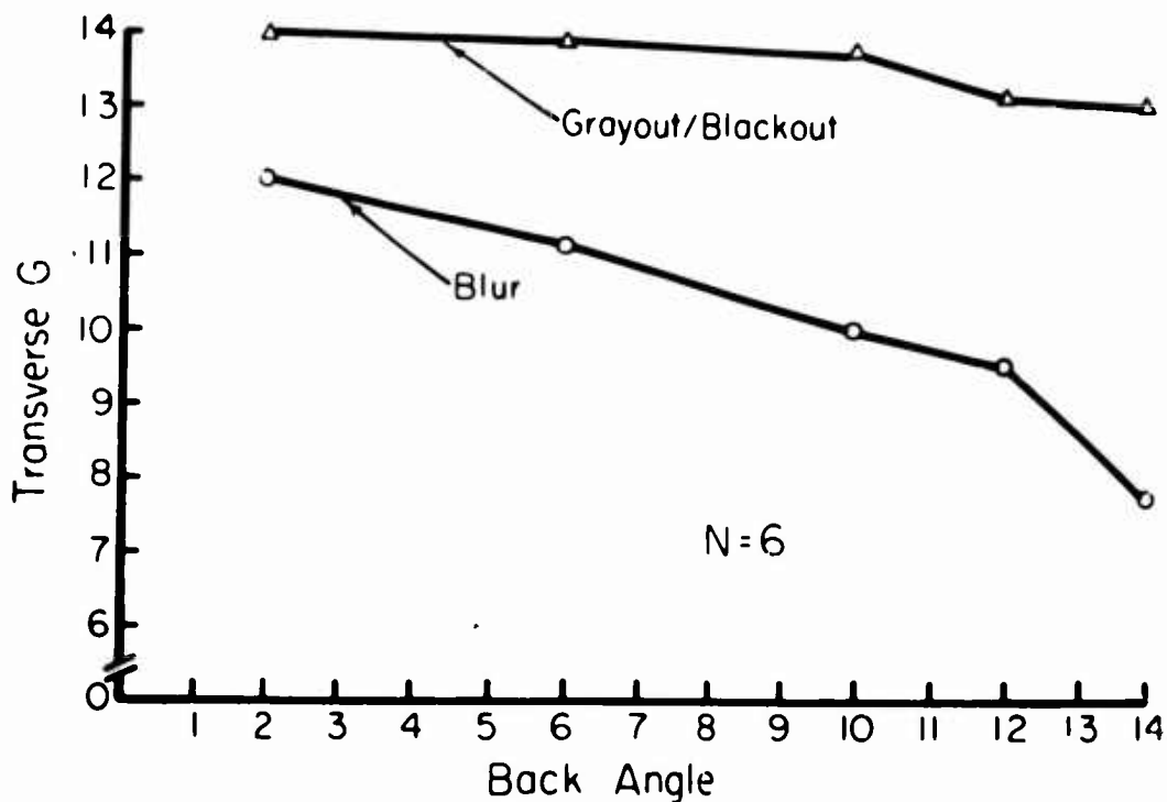
Figure 13. Grayout/blackout, and blur, as a function of back angle during exposure to transverse acceleration. (For this group of subjects, the rate of onset was 1.5 G/sec.)
