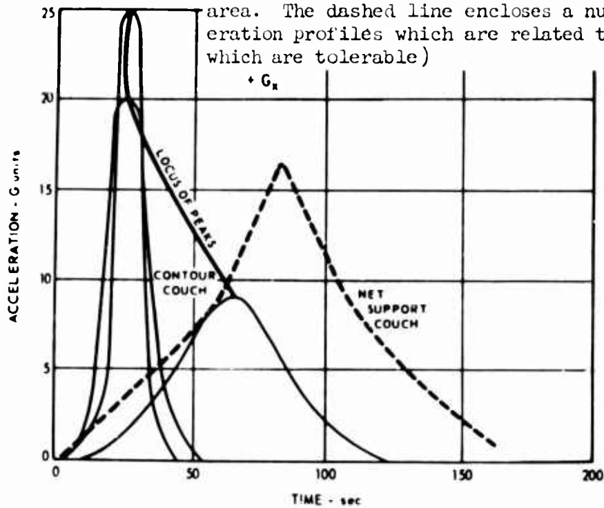
Figure 35. Comparison of maximum protection against the effects of transverse acceleration ( +G_x ), under conditions of optimal positioning in three types of restraint systems: contour couch, net support couch, and water immersion
