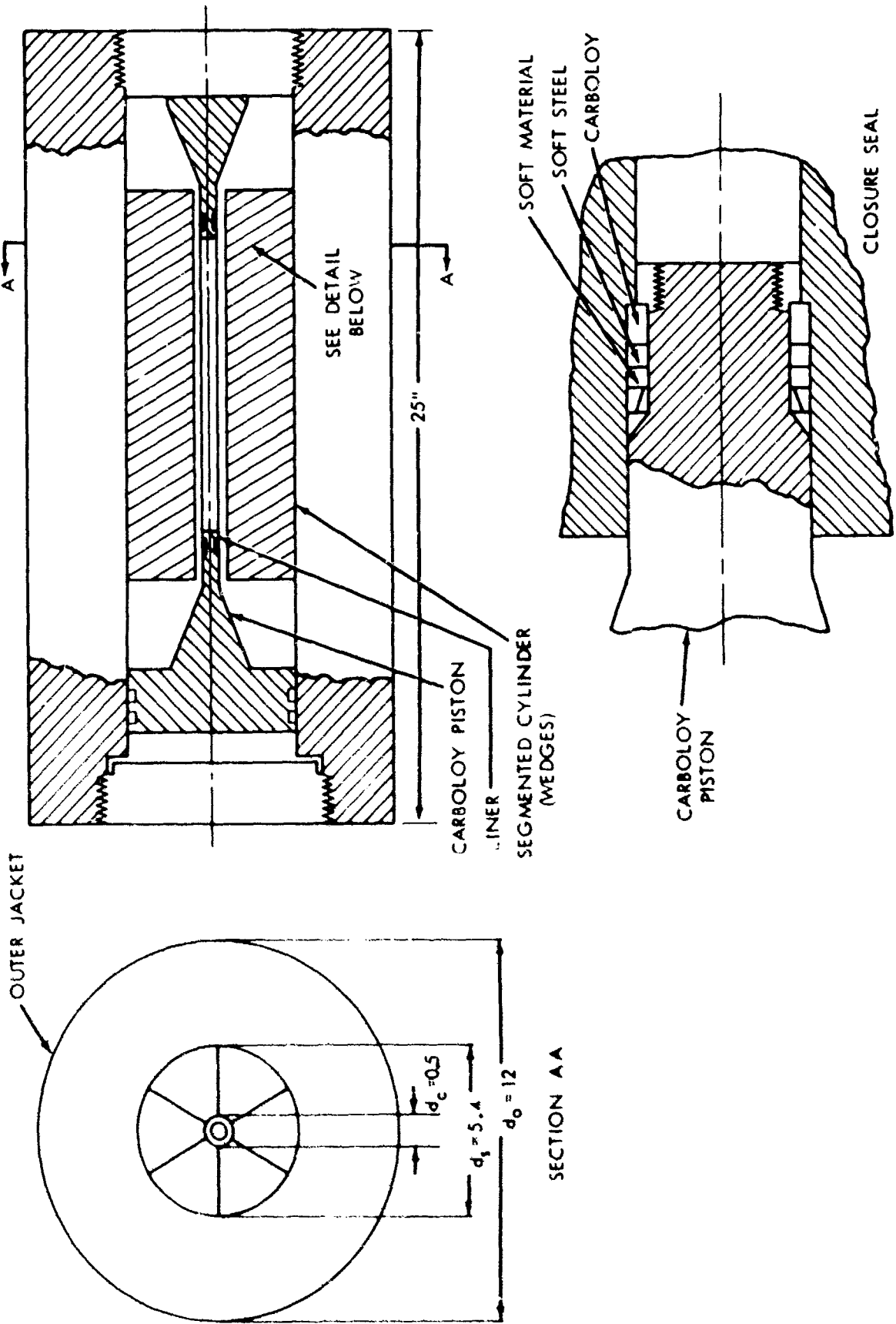
FIG. 7 DESIGN OF HIGH PRESSURE CHAMBER
