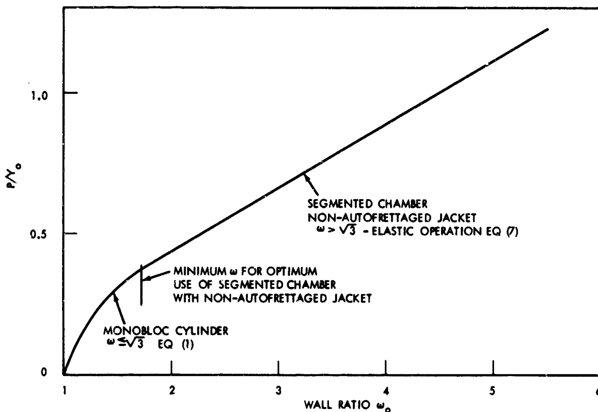
Fig. 4. p/Y_0 vs Wall Ratio (Segmented Chamber Non-autofrettaged Jacket)
