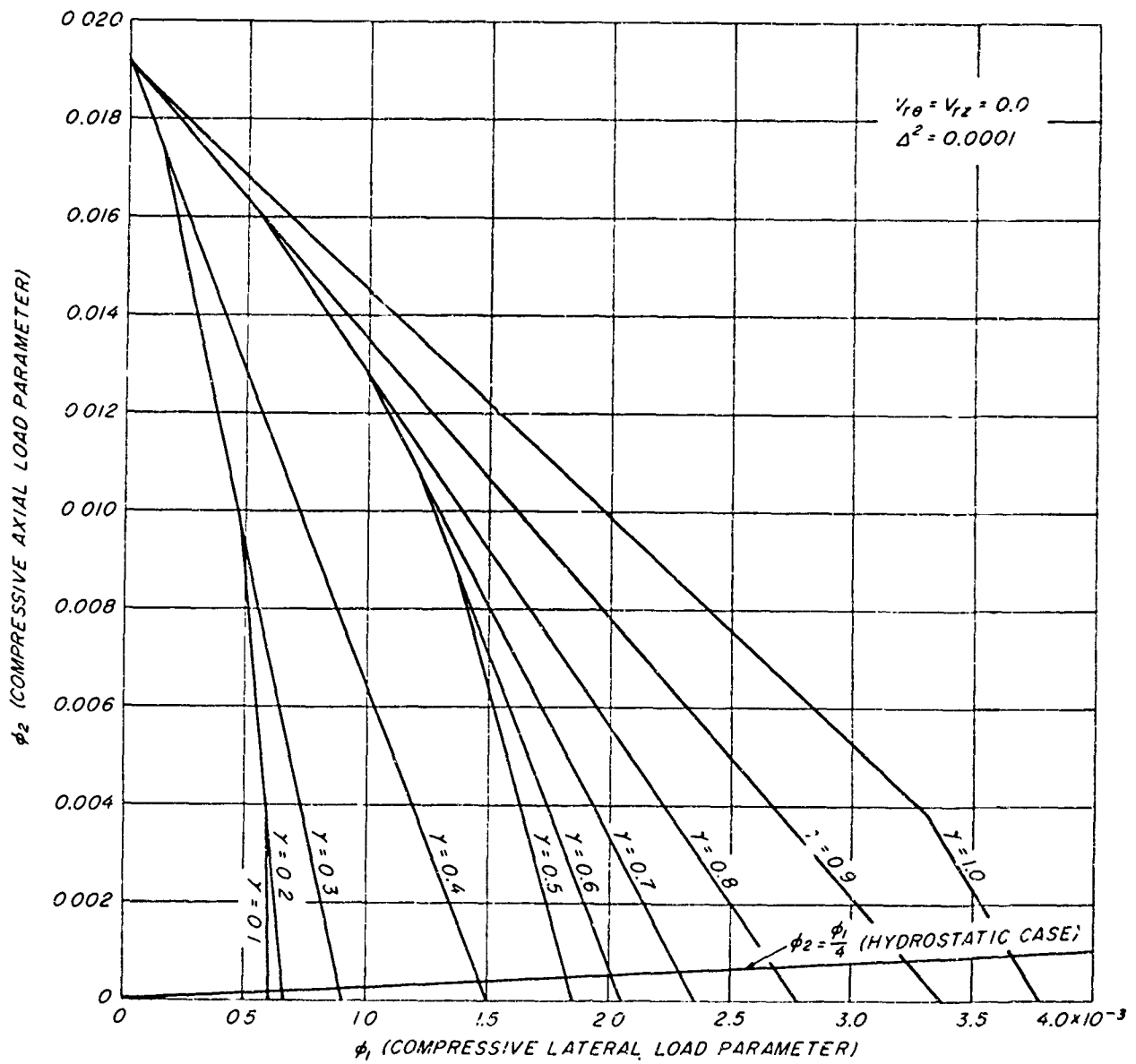
Figure 7.--Effect of combined loading for \Delta^2 = 0.0001 .
