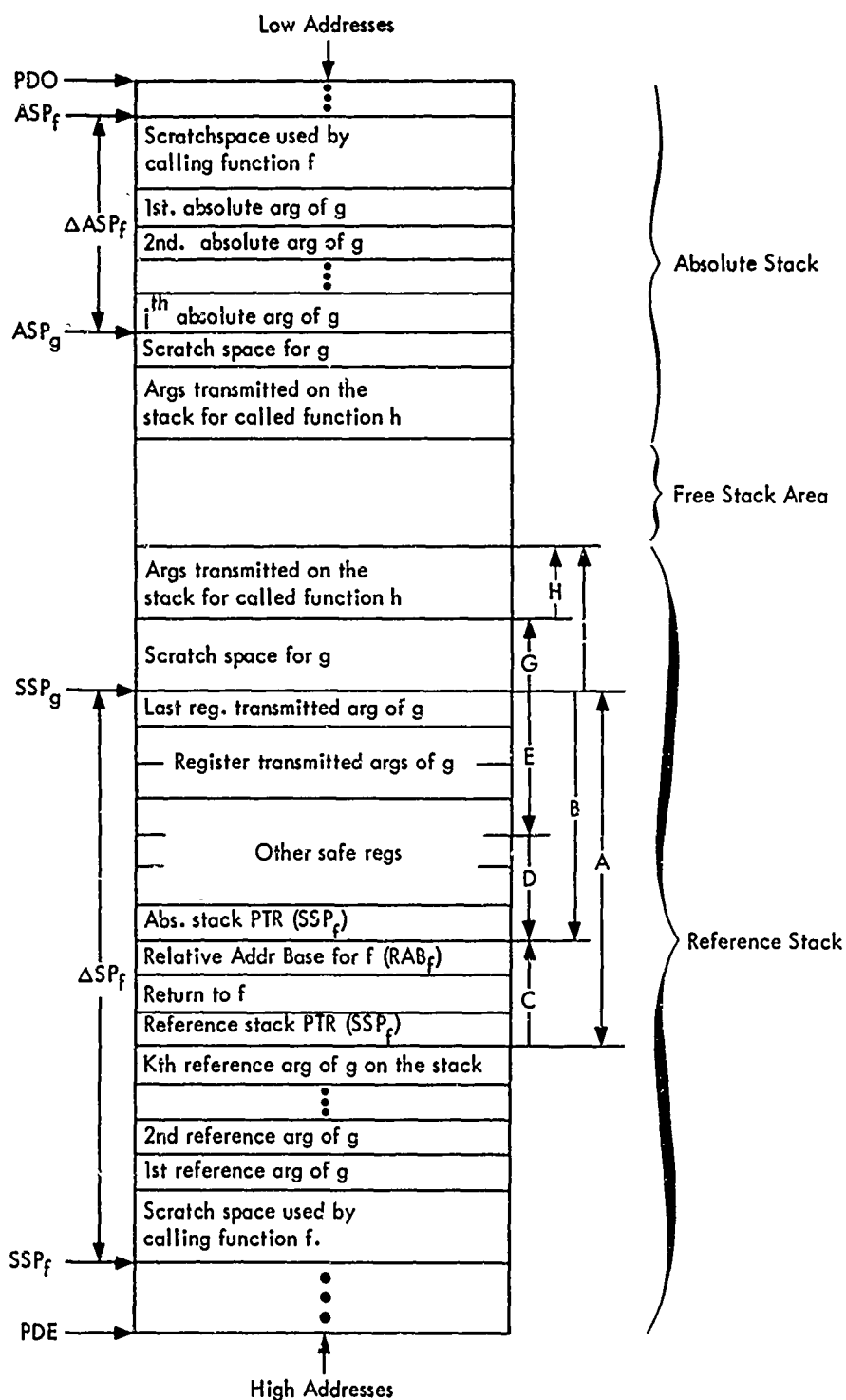
Figure 2. Pushdown Stack Space For The 360
