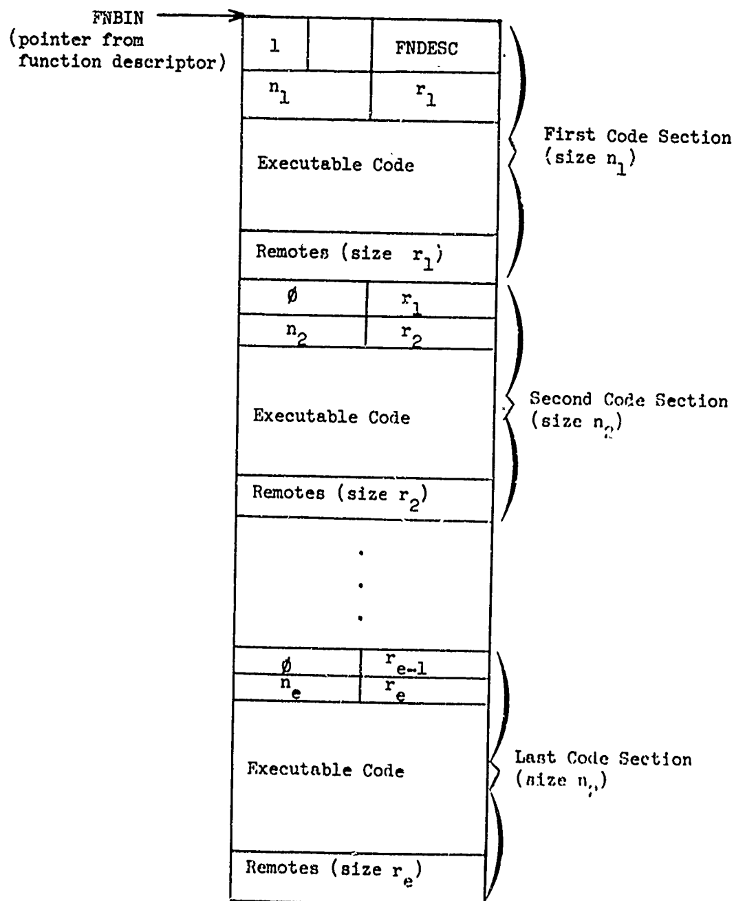
Figure 4. Possible Design of BPI for the 360
