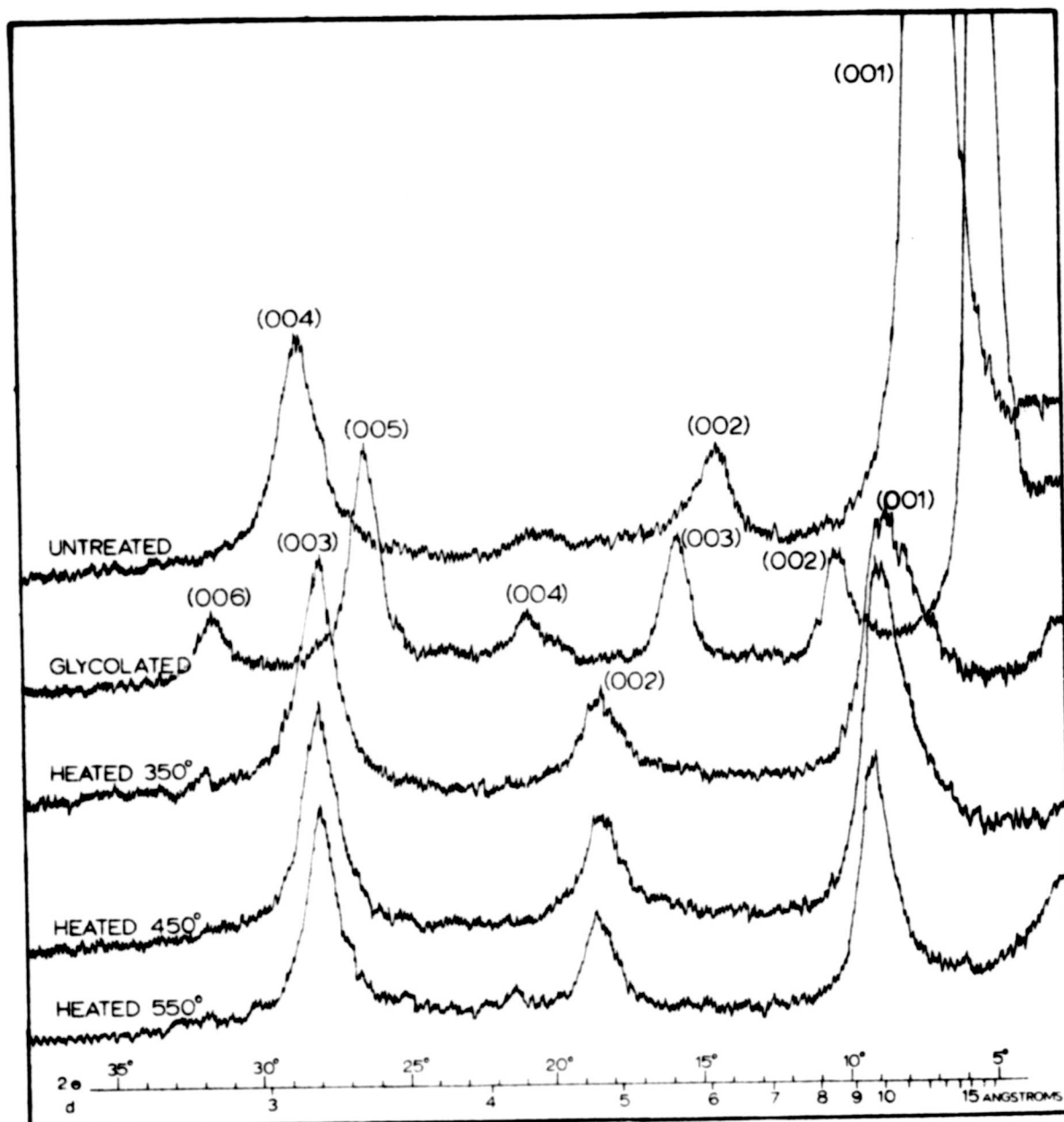
Fig. 4 X-ray diffractometer patterns of montrillonite in 2 \mu fraction of Sample 2. The (001) reflection expands 14 \text{ \AA} to 17 \text{ \AA} on glycolation. The structure collapses reversibly to 10 \text{ \AA} at temperatures as low 350^\circ\text{C} but irreversible collapse is not encountered until 550^\circ\text{C} , when the montmorillonite anhydride or illitic structure is formed.
