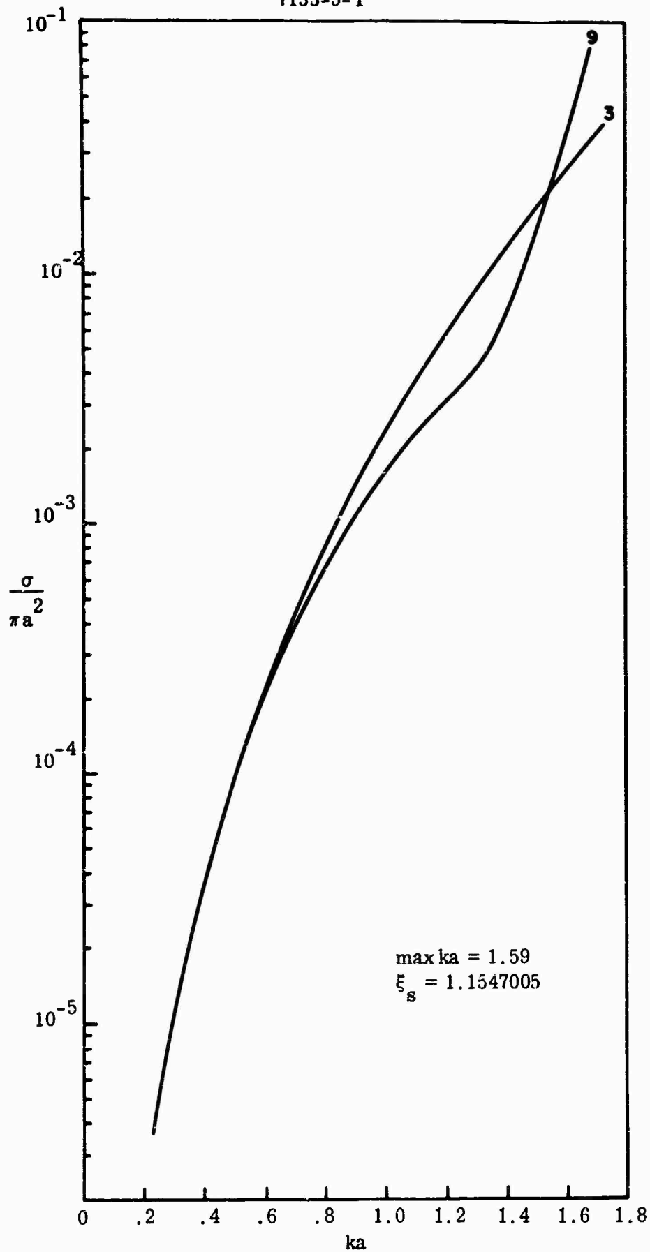
FIG. 6.4a: FORWARD SCATTERING CROSS SECTION OF HARD, 2:1 PROLATE SPHEROID FOR NOSE-ON INCIDENCE.
