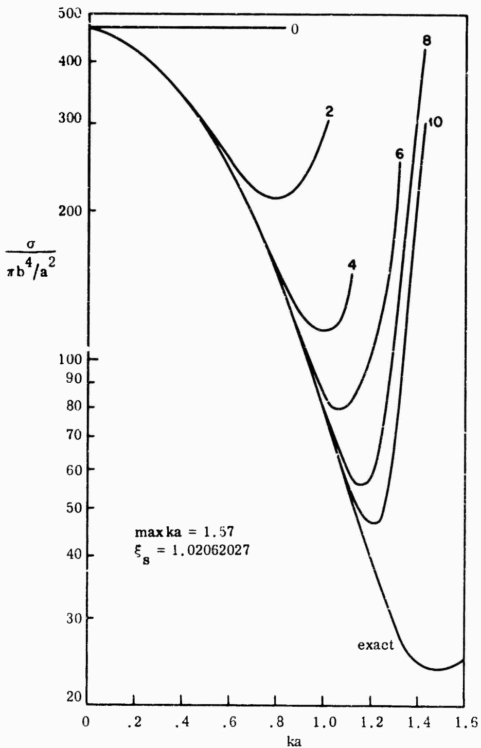
FIG. 6-1b: BACK SCATTERING CROSS SECTION OF SOFT, 5:1 PROLATE SPHEROID FOR NOSE-ON INCIDENCE.
