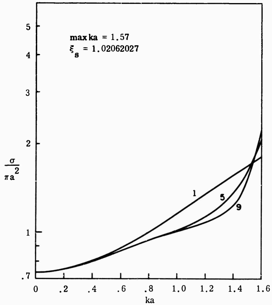
FIG. 6-3b: FORWARD SCATTERING CROSS SECTION OF SOFT, 5:1 PROLATE SPHEROID FOR NOSE-ON INCIDENCE.
