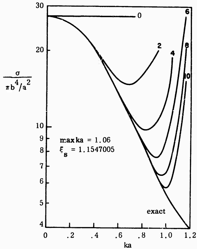
FIG. 6-1a: BACK SCATTERING CROSS SECTION OF SOFT, 2:1 PROLATE SPHEROID FOR NOSE-ON INCIDENCE.
