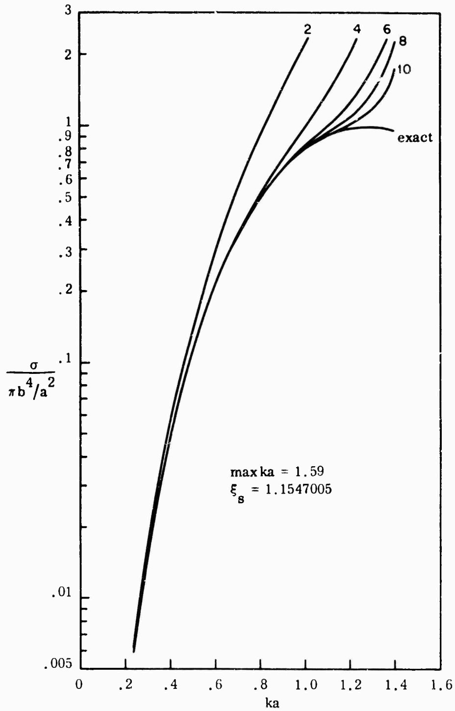
FIG. 6-2a: BACK SCATTERING CROSS SECTION OF HARD, 2:1 PROLATE SPHEROID FOR NOSE-ON INCIDENCE.
