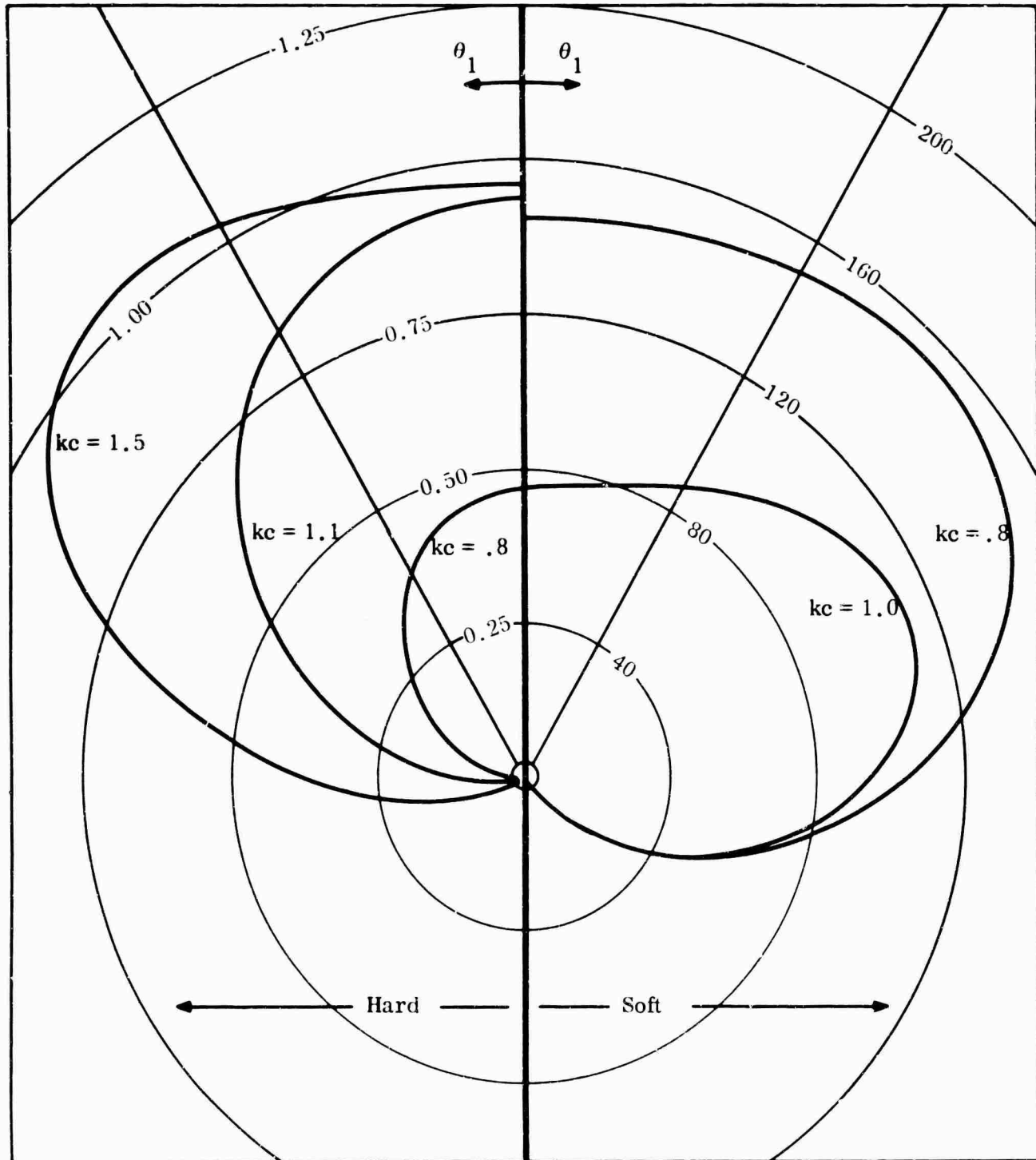
FIG. 6-6: BISTATIC CROSS SECTION OF 5:1 PROLATE SPHEROID FOR NOSE-ON INCIDENCE.
