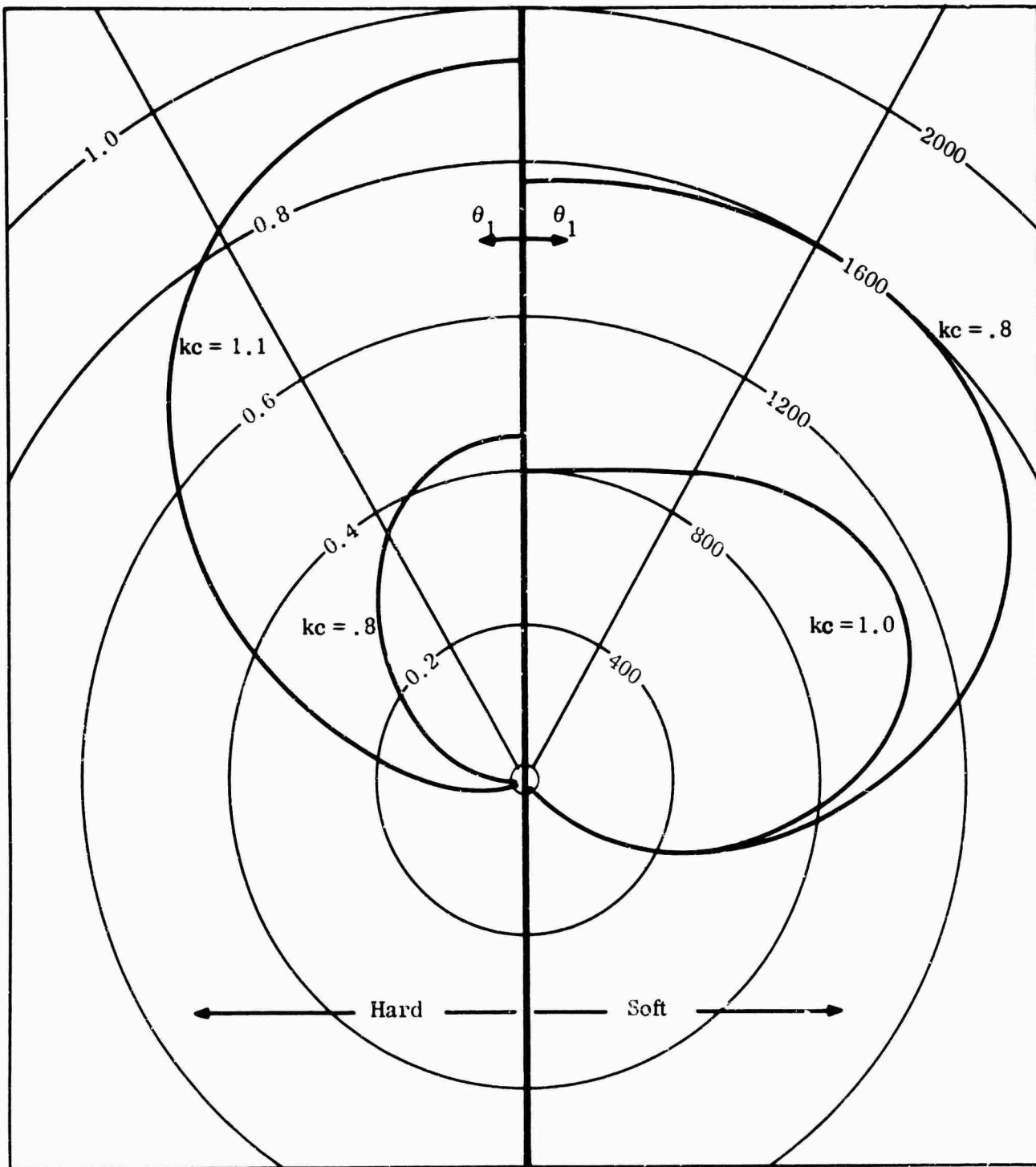
FIG. 6-8: BISTATIC CROSS SECTION OF 10:1 PROLATE SPHEROID FOR NOSE-ON INCIDENCE.
