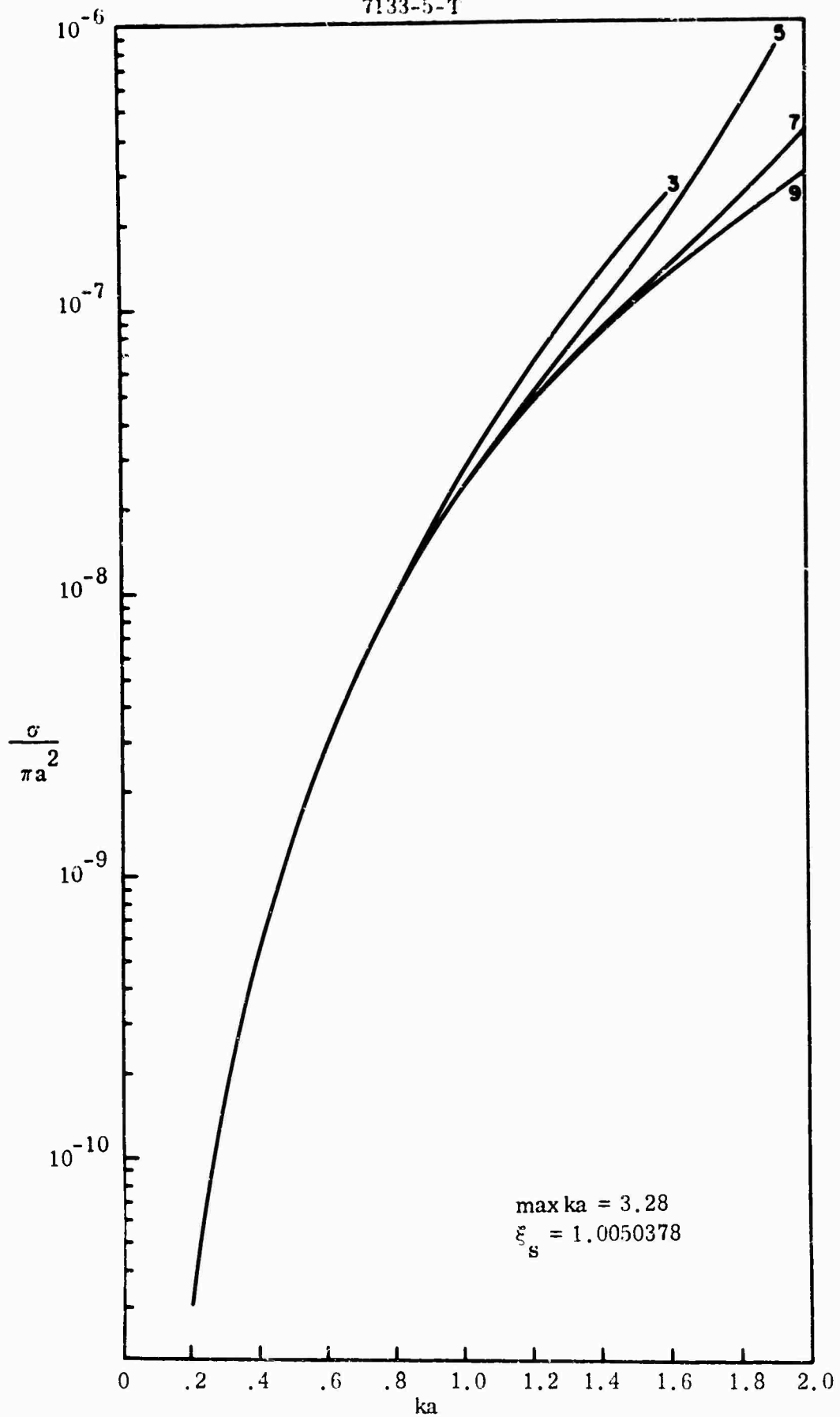
FIG. 6-4c: FORWARD SCATTERING CROSS SECTION OF HARD, 10:1 PROLATE SPHEROID FOR NOSE-ON INCIDENCE.
