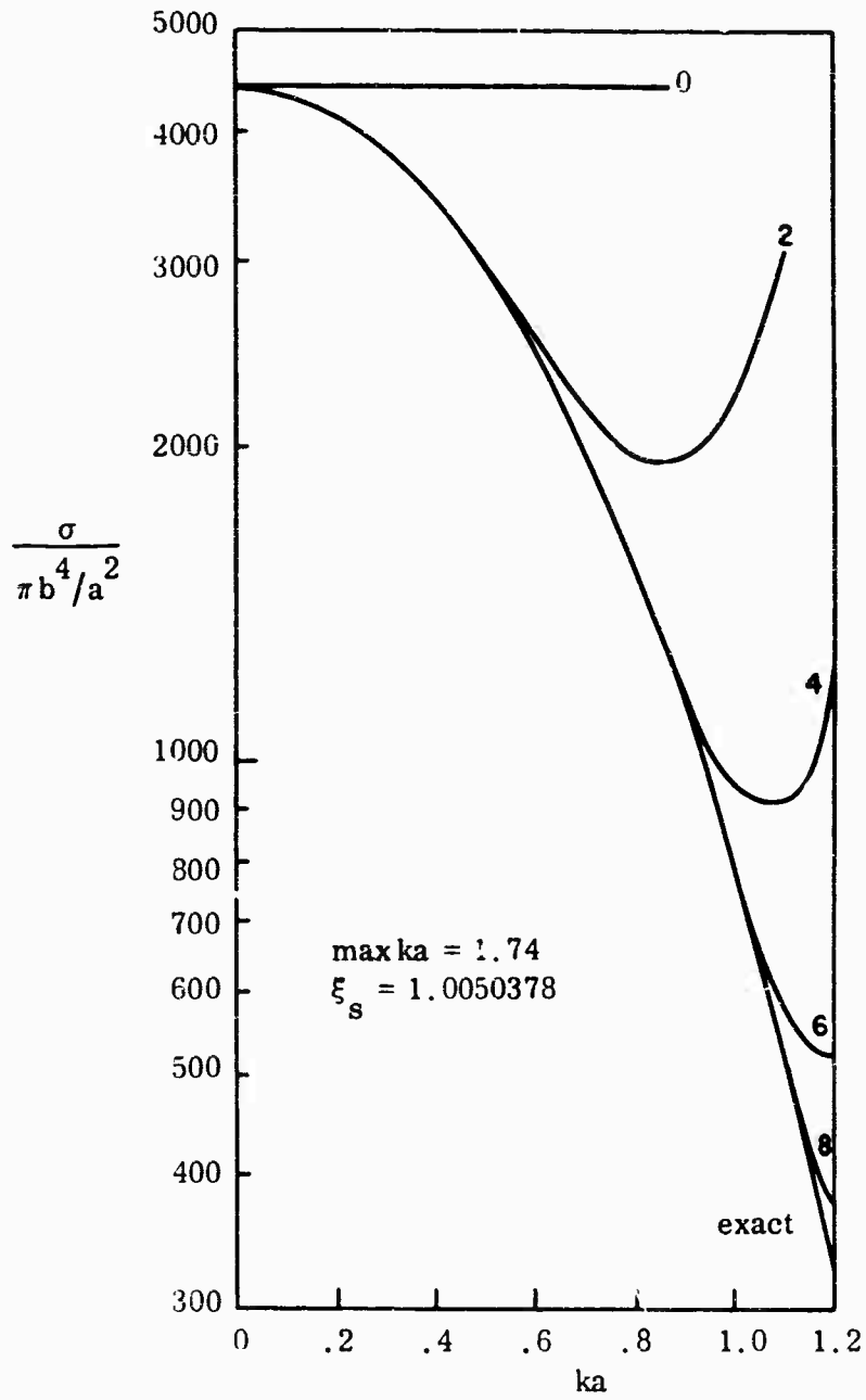
FIG. 6-1c: BACK SCATTERING CROSS SECTION OF SOFT, 10:1 PROLATE SPHEROID FOR NOSE-ON INCIDENCE.
