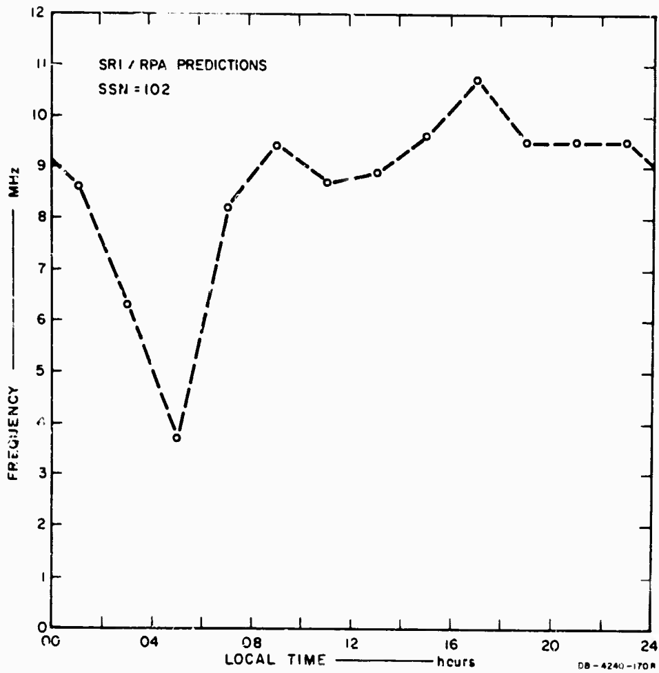
FIG. 13 CORRECTED foF2 PREDICTIONS FOR SEPTEMBER 1967
