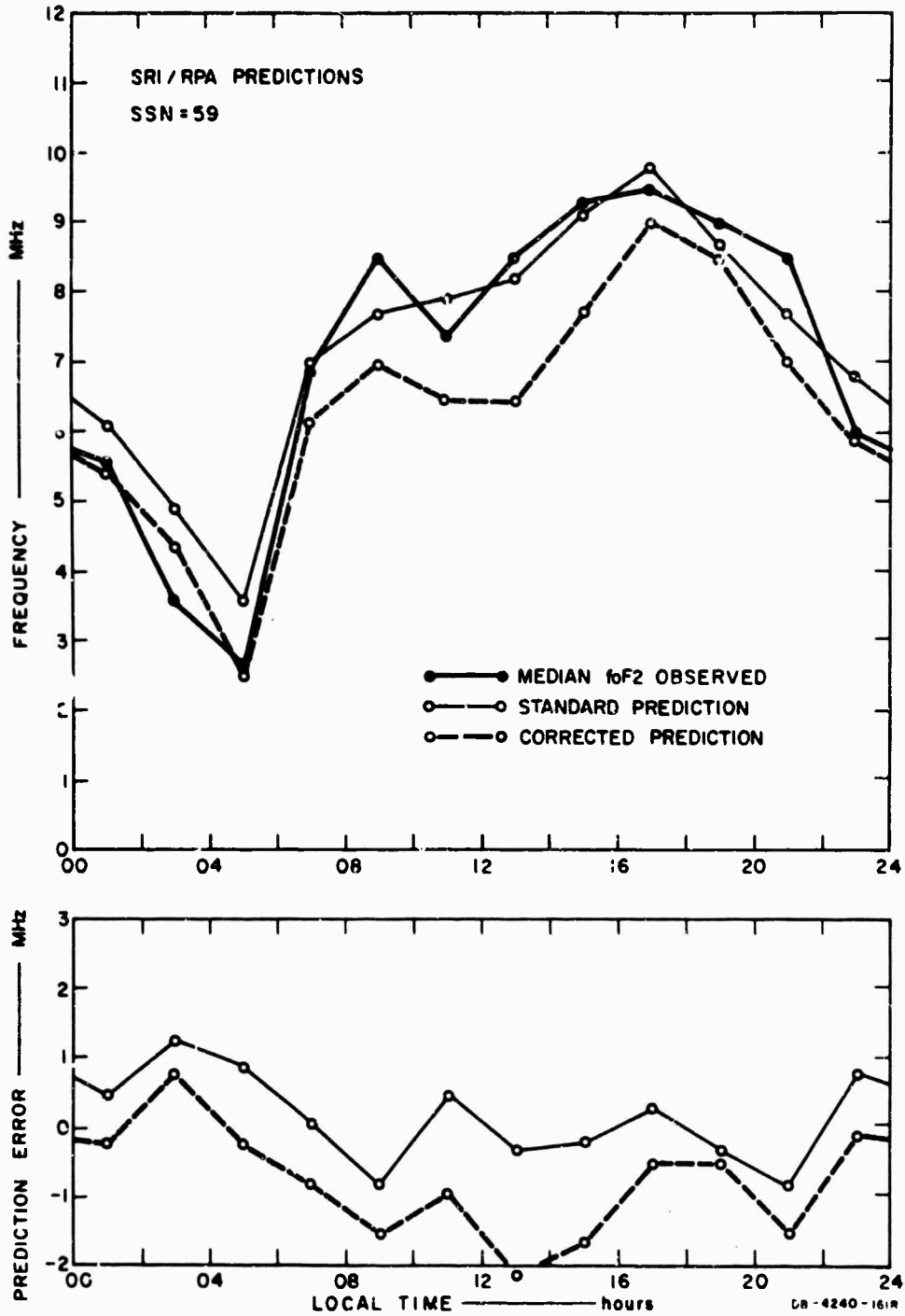
FIG. A-17 COMPARISON OF OBSERVED AND SRI/RPA-PREDICTED MONTHLY MEDIAN foF2 FOR AUGUST 1966
