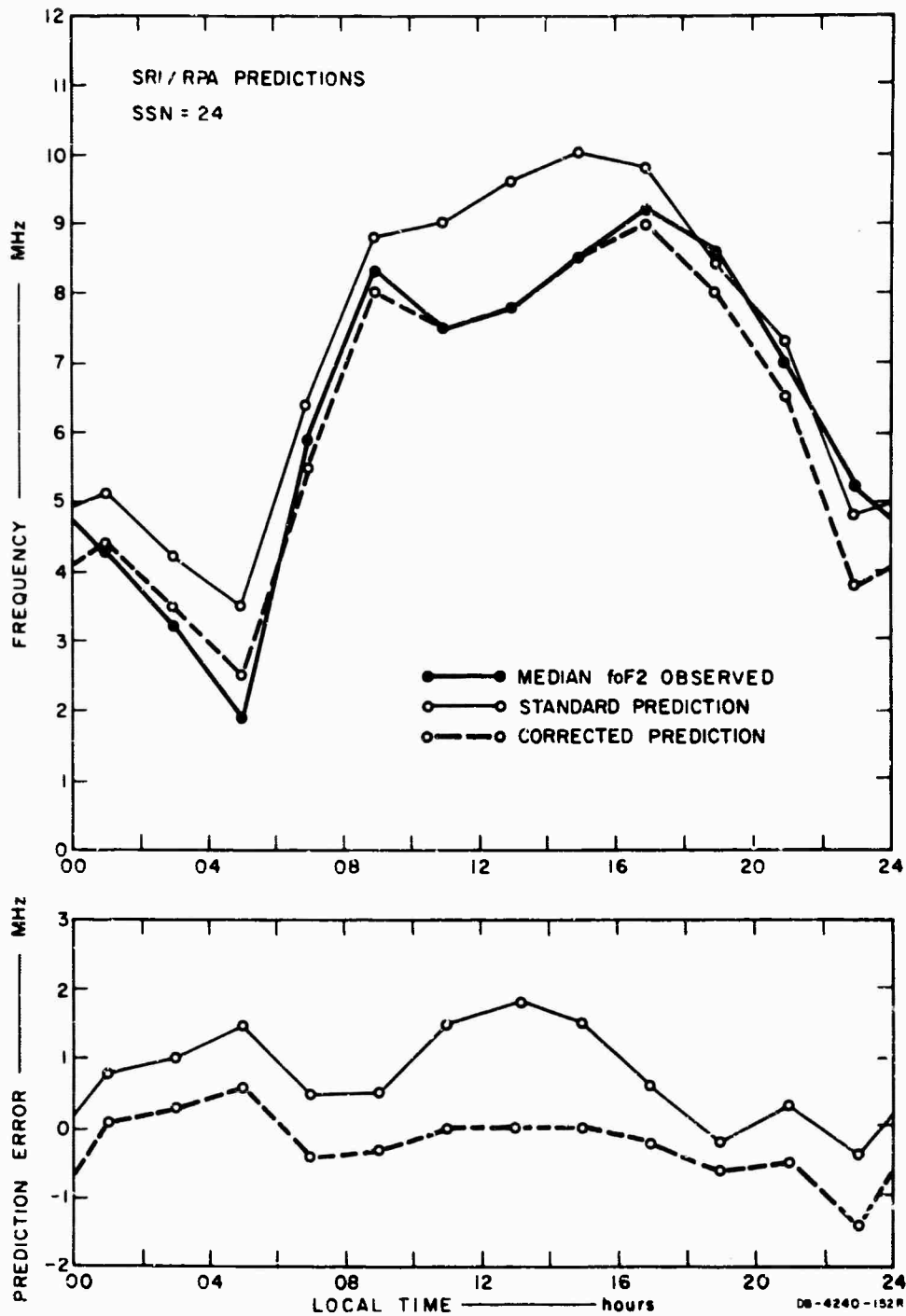
FIG. A-8 COMPARISON OF OBSERVED AND SRI/RPA-PREDICTED MONTHLY MEDIAN foF2 FOR NOVEMBER 1965
