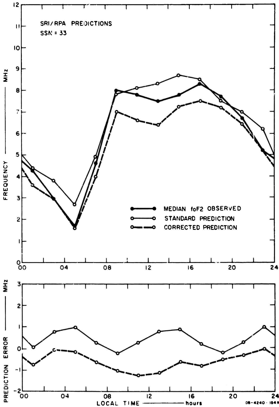
FIG. A-10 COMPARISON OF OBSERVED AND SRI RPA-PREDICTED MONTHLY MEDIAN foF2 FOR JANUARY 1966
