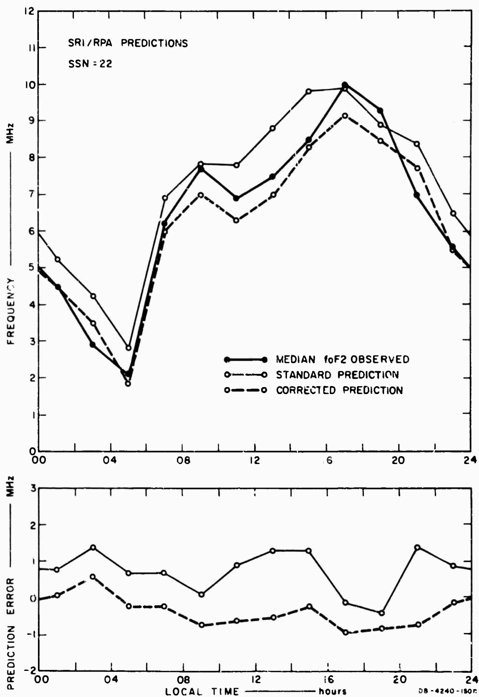
FIG. A-6 COMPARISON OF OBSERVED AND SRI RPA-PREDICTED MONTHLY MEDIAN foF2 FOR SEPTEMBER 1965
