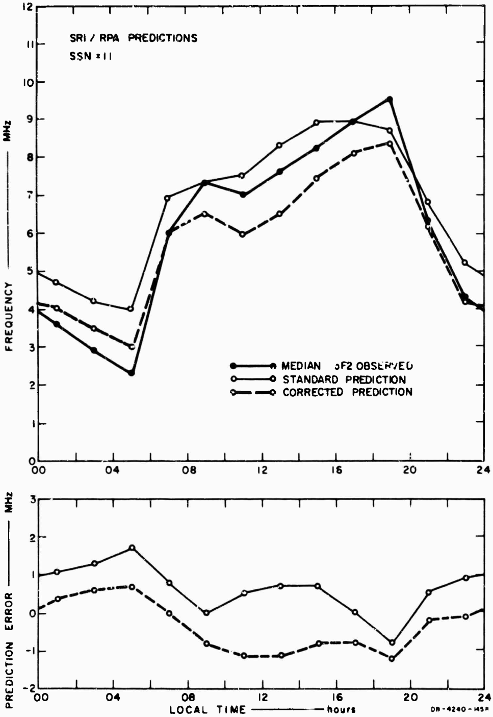
FIG. 1 COMPARISON OF OBSERVED AND PREDICTED MONTHLY MEDIAN f_oF_2 FOR MAY 1965
