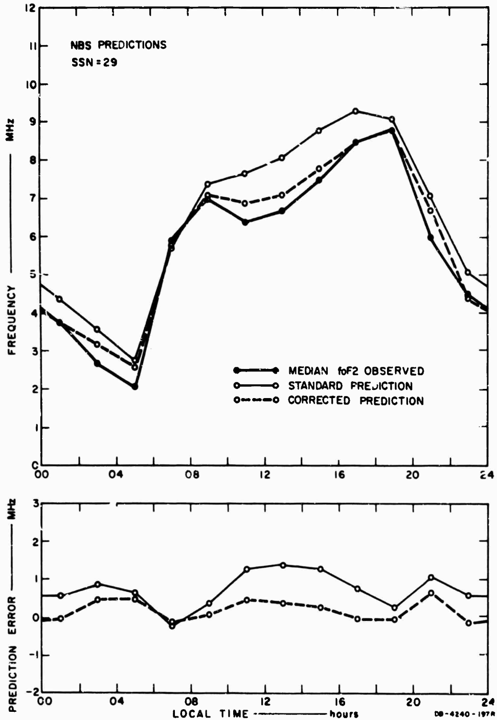
FIG. B-5 COMPARISON OF OBSERVED AND NBS-PREDICTED MONTHLY MEDIAN foF2 FOR AUGUST 1965
