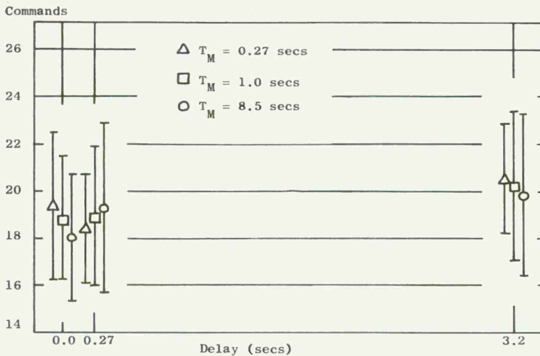
Fig. 16. Effect of Delay and Lag on Number of Commands used (Continuous and Intermittent Vision Combined).
