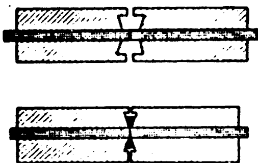
Fig. 129. Scheme of cold butt seam welding.
