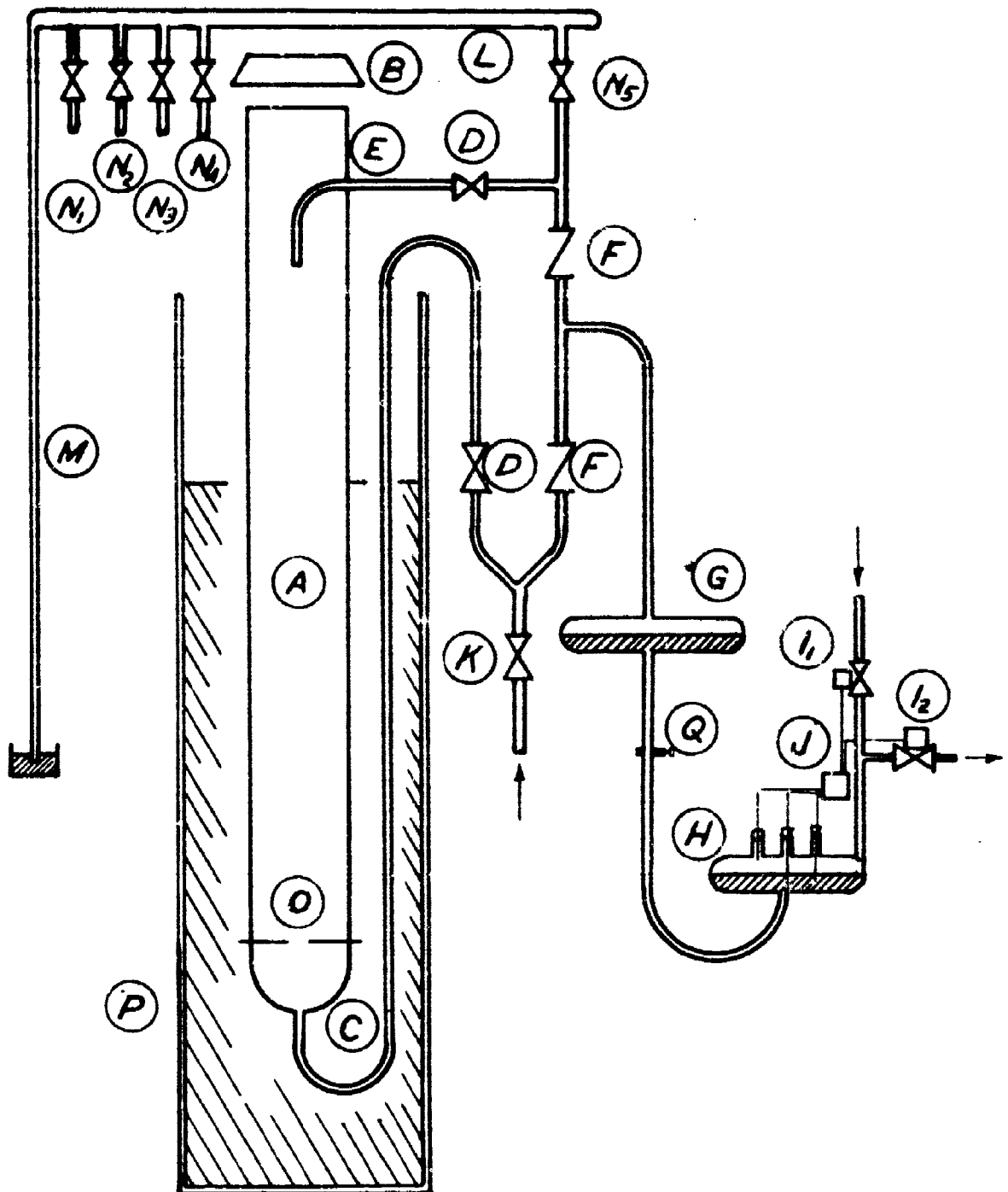
FIG. APPARATUS FOR THE DETERMINATION OF FLAMMABILITY LIMITS AT VARIOUS TEMPERATURES
