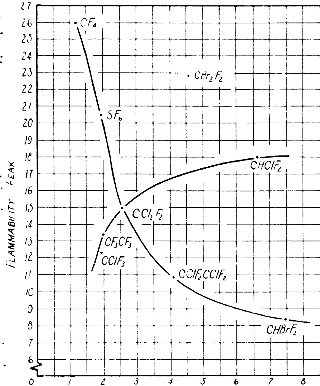
DIELECTRIC CONSTANT \times 10^{-3} Figure 50. Relationship between Dielectric Constant and flammability peak
