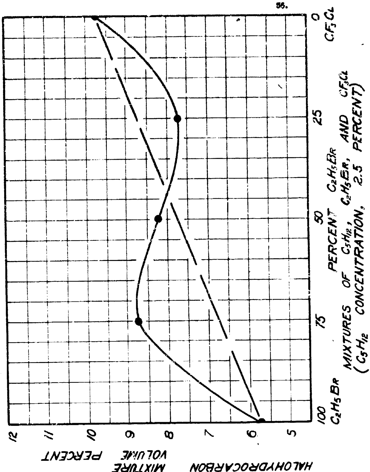
Figure 61 Effect of Binary Mixtures in Decreasing the Flammability of Air and Pentane
