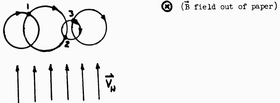
Fig. 1 Ion in a Neutral-Particle Bath
