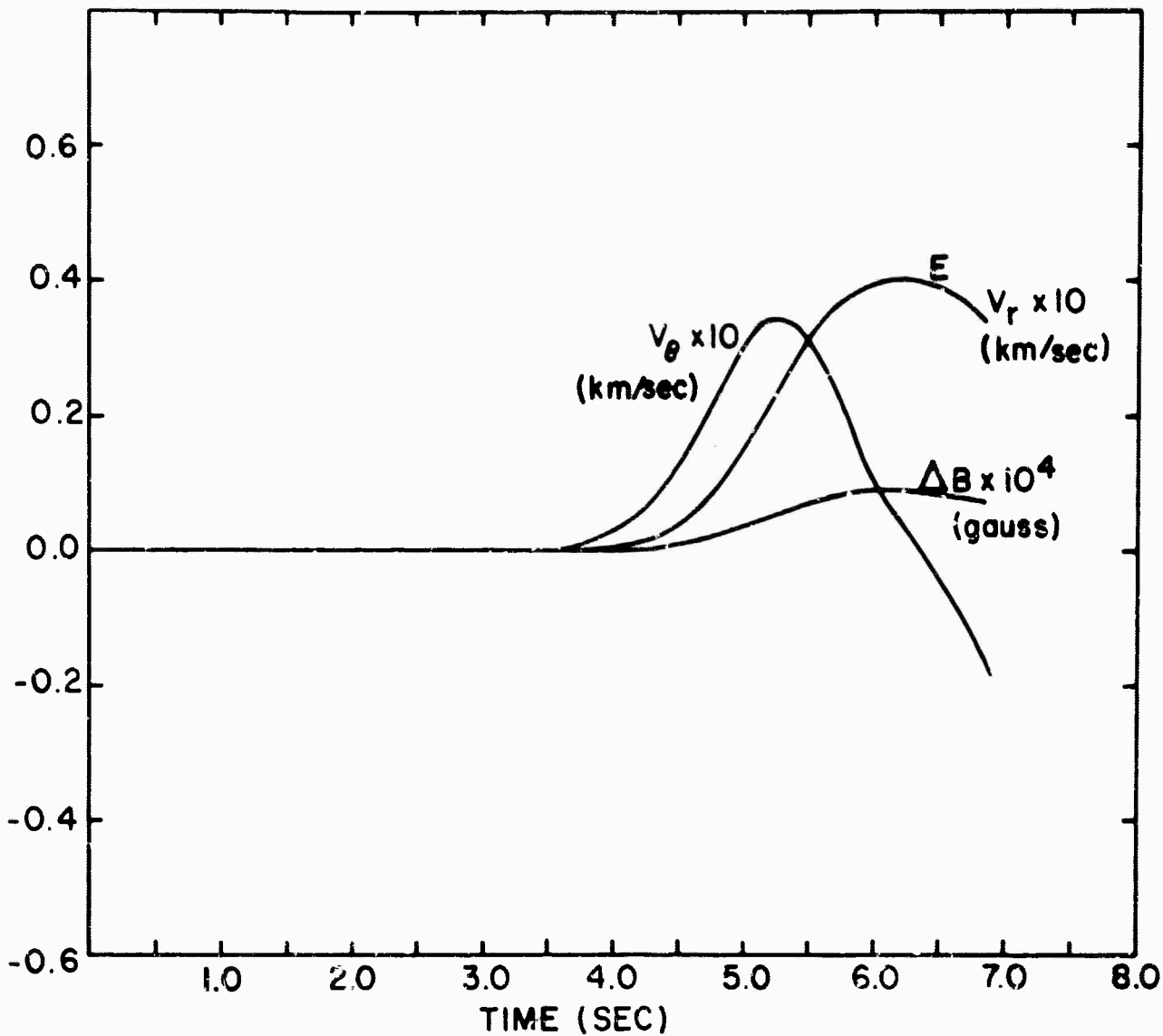
FIG. V-6. TIME HISTORIES AT R = 8 km
