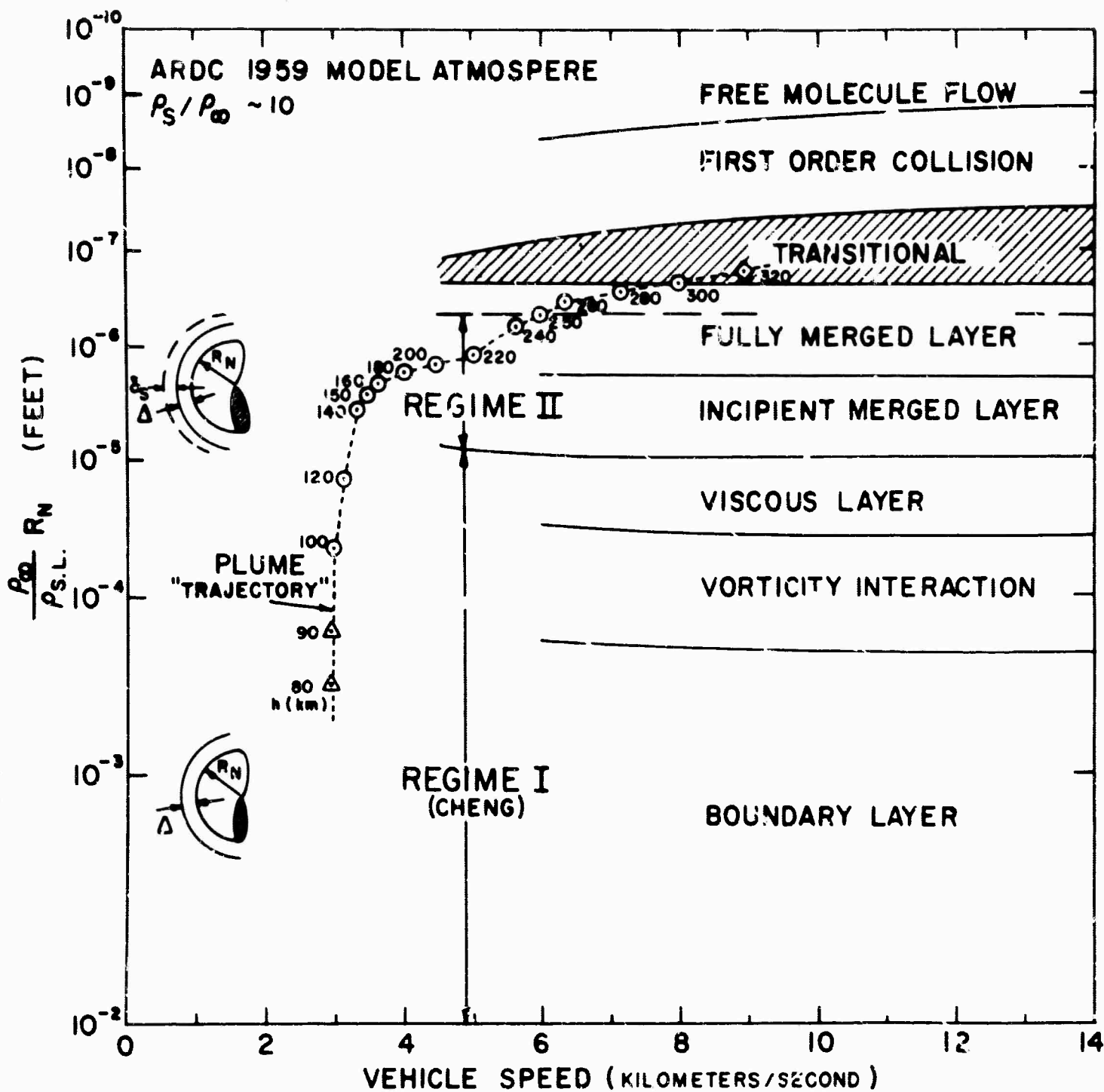
FIG. II-16. PLUME "TRAJECTORY" IN RELATION TO THE LOW DENSITY VISCOUS REGIMES AS DEFINED BY PROBSTEIN AND BY CHENG (REF. 2).
