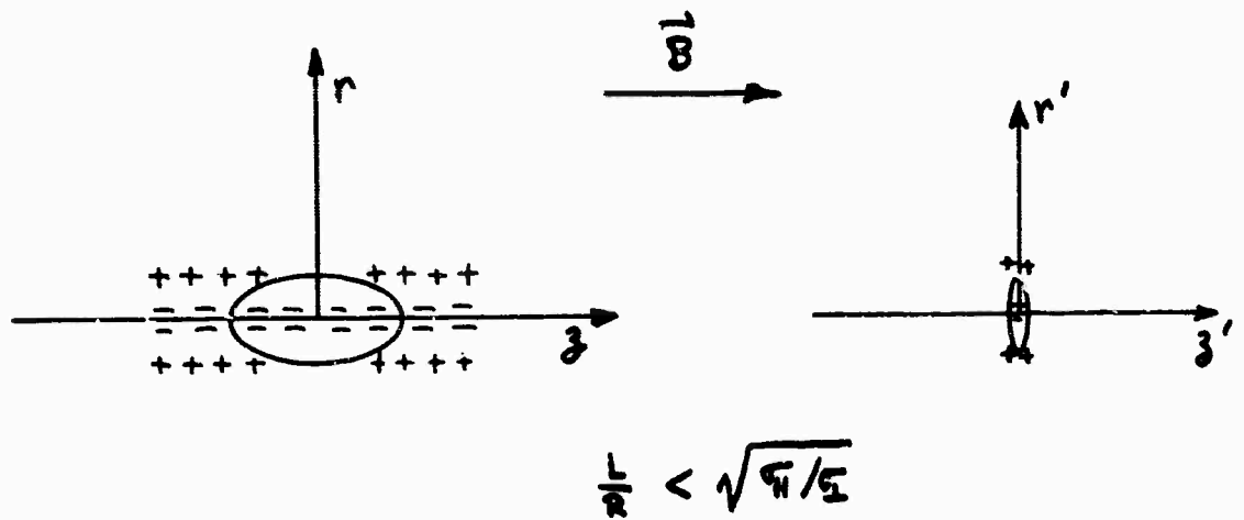
Fig. V-2a Charge distributions in the real and transformed space.
