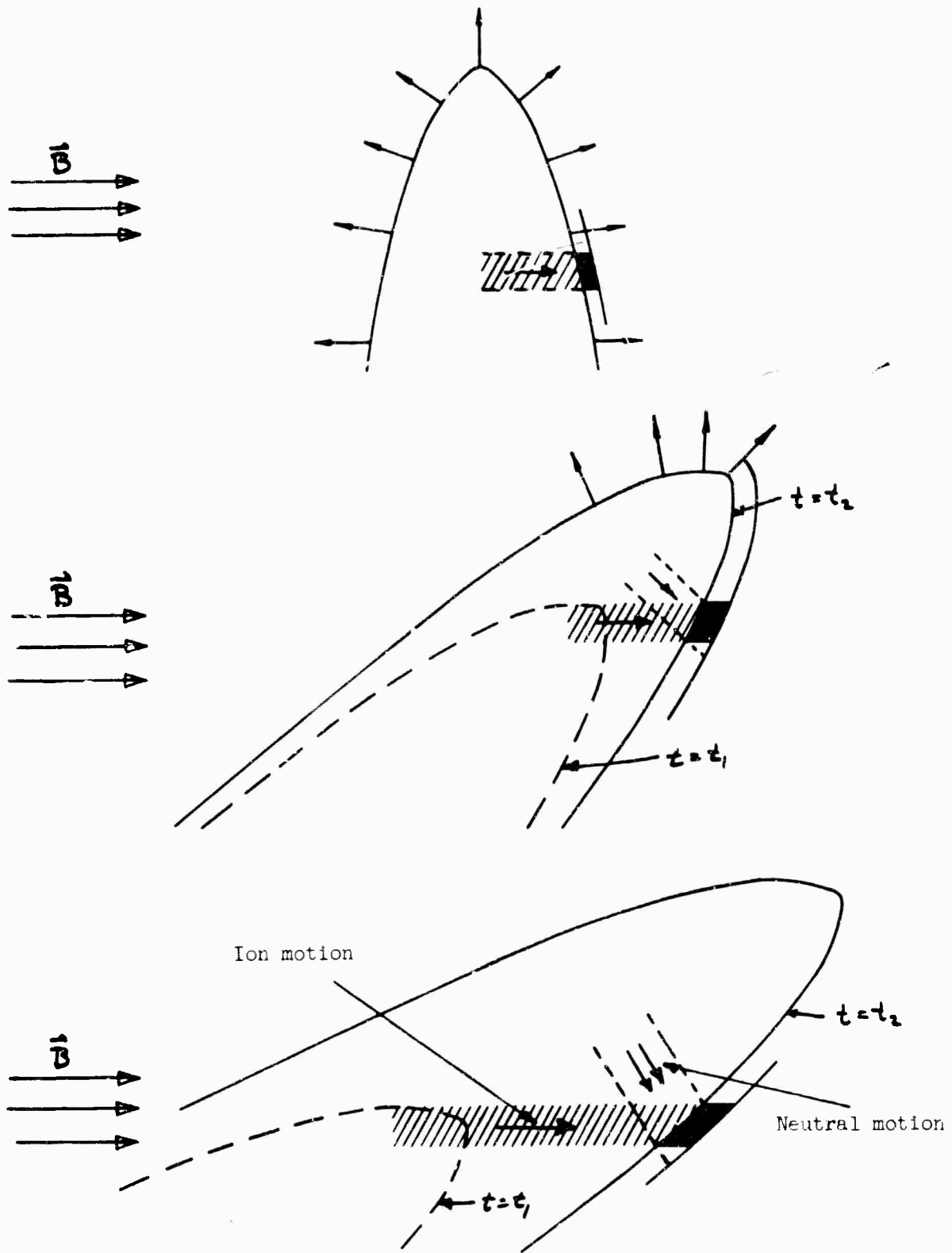
Fig. III-2. Relative motion of ions and neutrals at various inclinations of trajectory to magnetic field.
