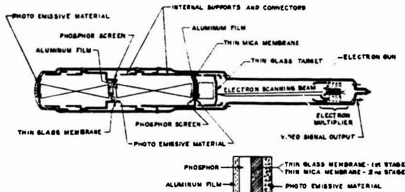
FIGURE 2. RCA two-stage intensifier image orthicon.
