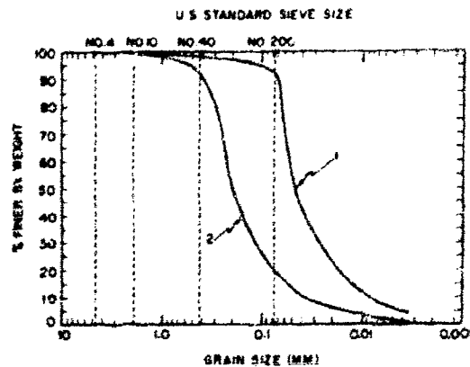
Figure 1. Sieve analyses of typical soils from the test area. Sample 1 - silt (OL) from 0-2 ft depth, nonplastic. Sample 2 - silty sand (SM) from 2-5 ft depth, nonplastic.
