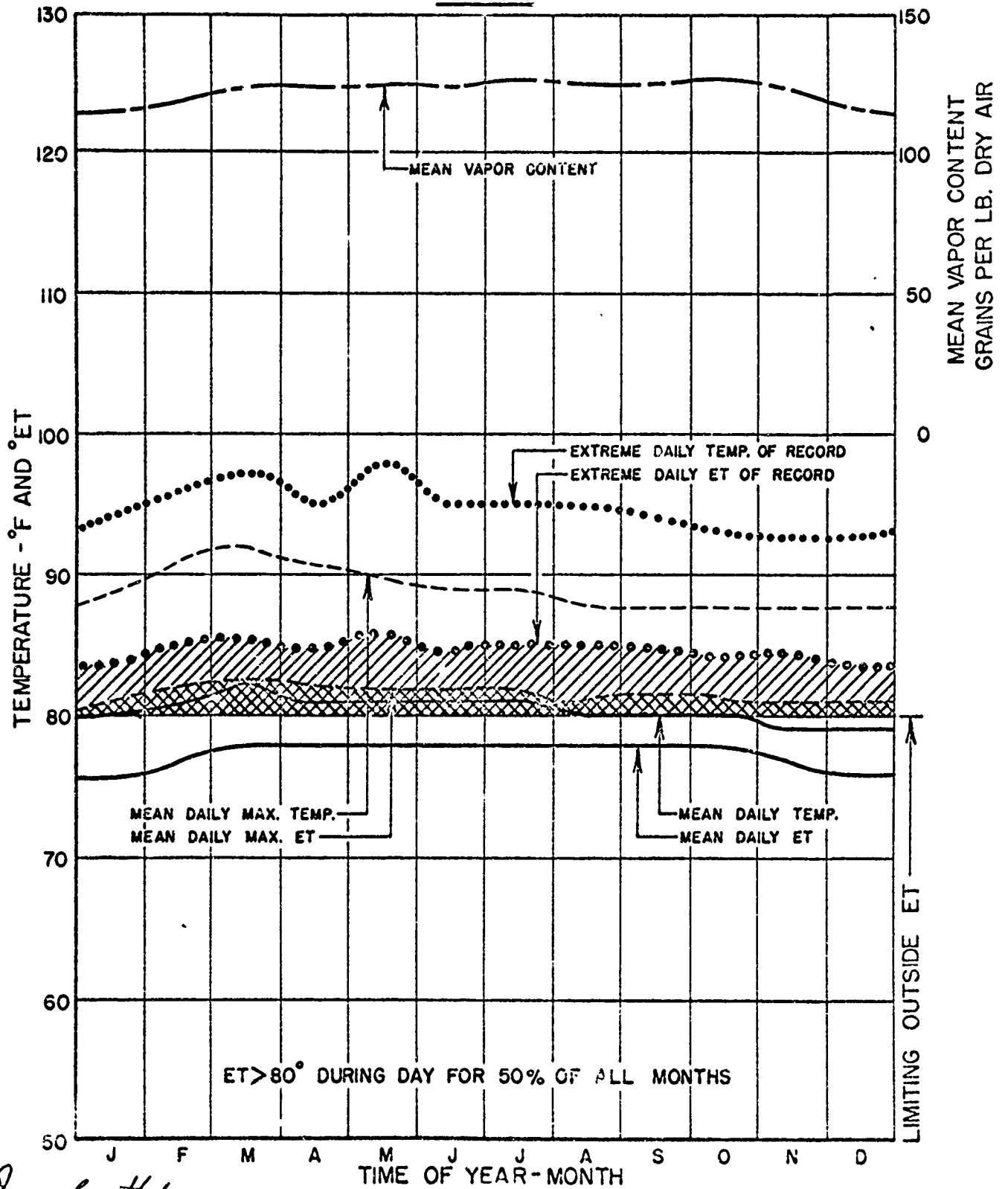
FIG. 6A YEARLY VARIATION IN TEMPERATURE, VAPOR CONTENT AND EFFECTIVE TEMPERATURE PENANG
