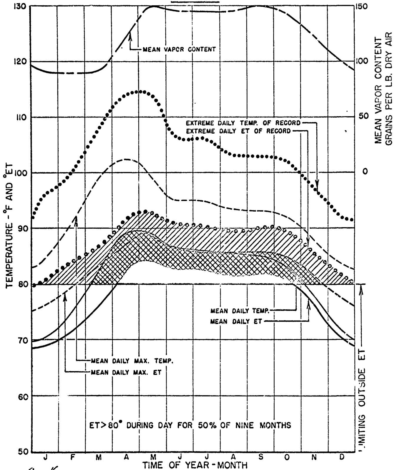
FIG. 7A YEARLY VARIATION IN TEMPERATURE, VAPOR CONTENT AND EFFECTIVE TEMPERATURE MANDALAY
