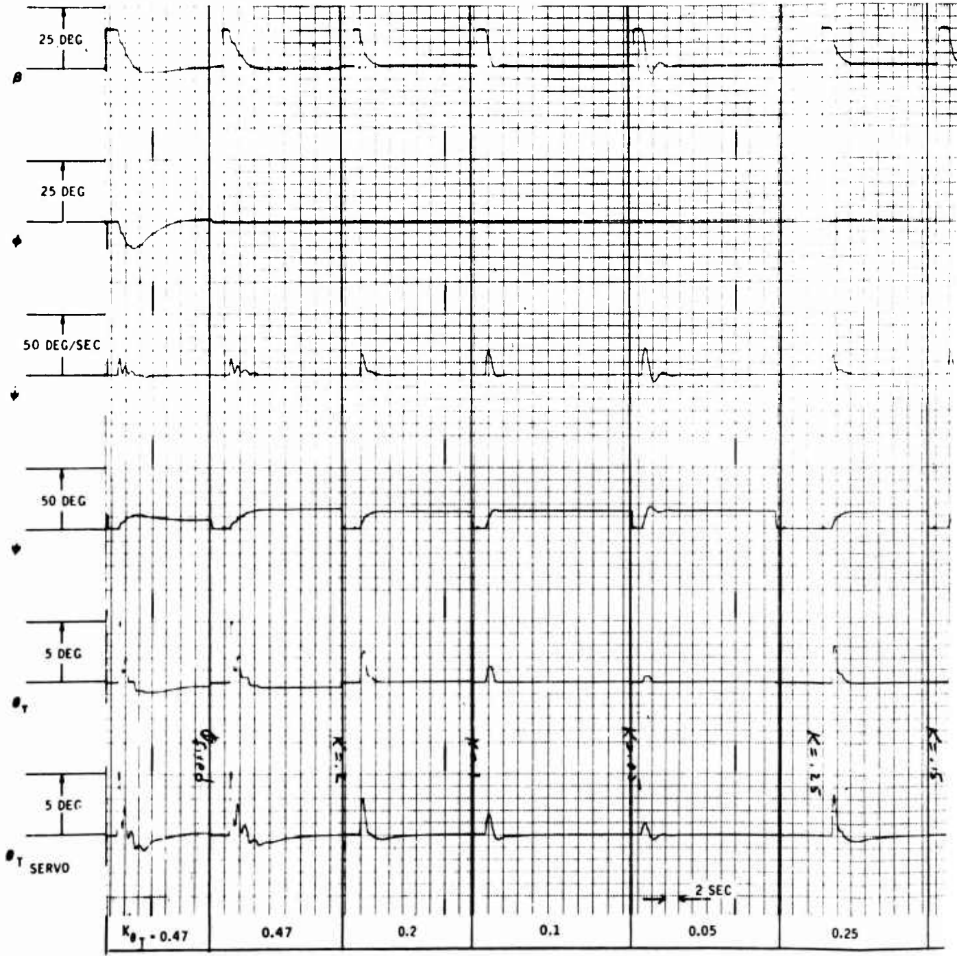
VARATION IN TOTAL LOOP GAIN
