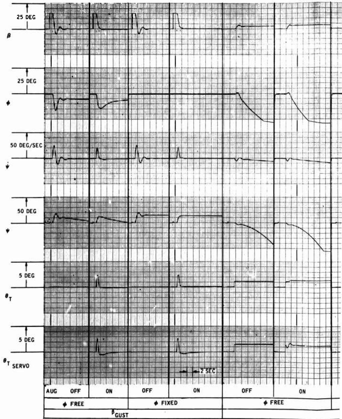
Figure 13. 120 Knots - Nominal Perform
