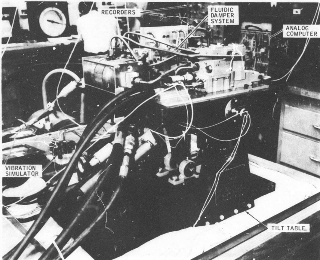
Figure 56. Tilt Table
