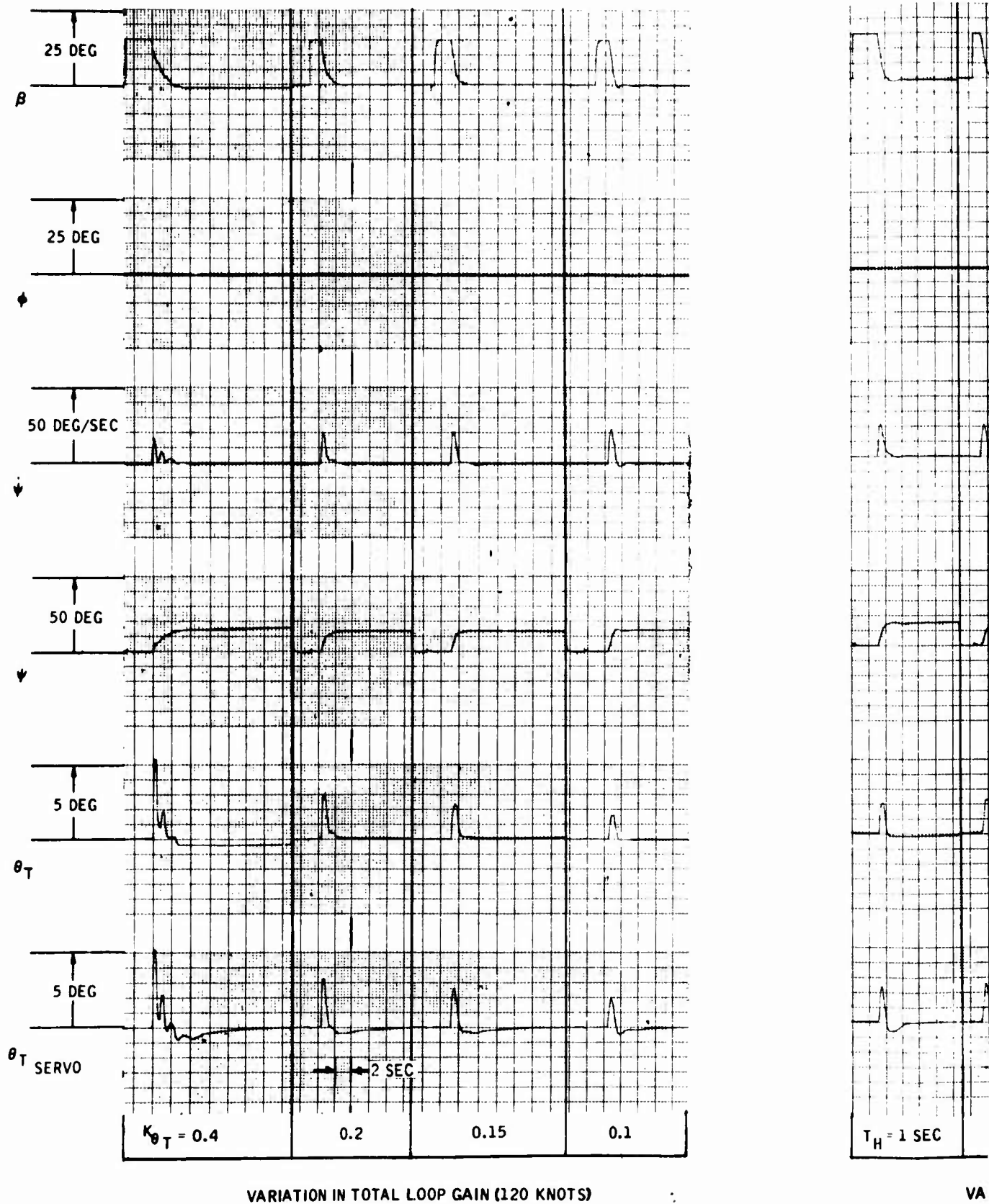
Figure 23. 120 Knots - Parametric Study
