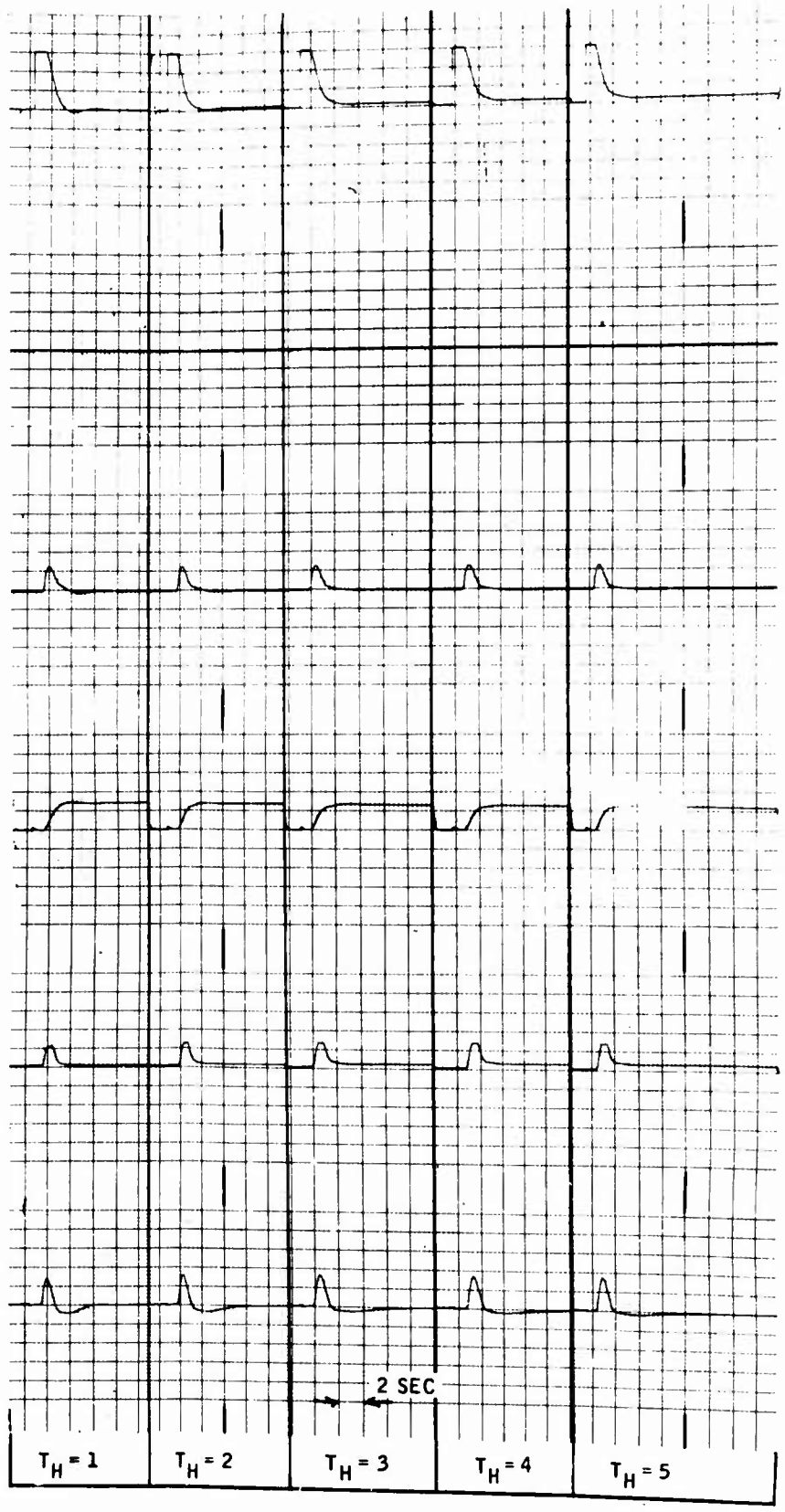
VARIATION IN HI-PASS TIME CONSTANT
