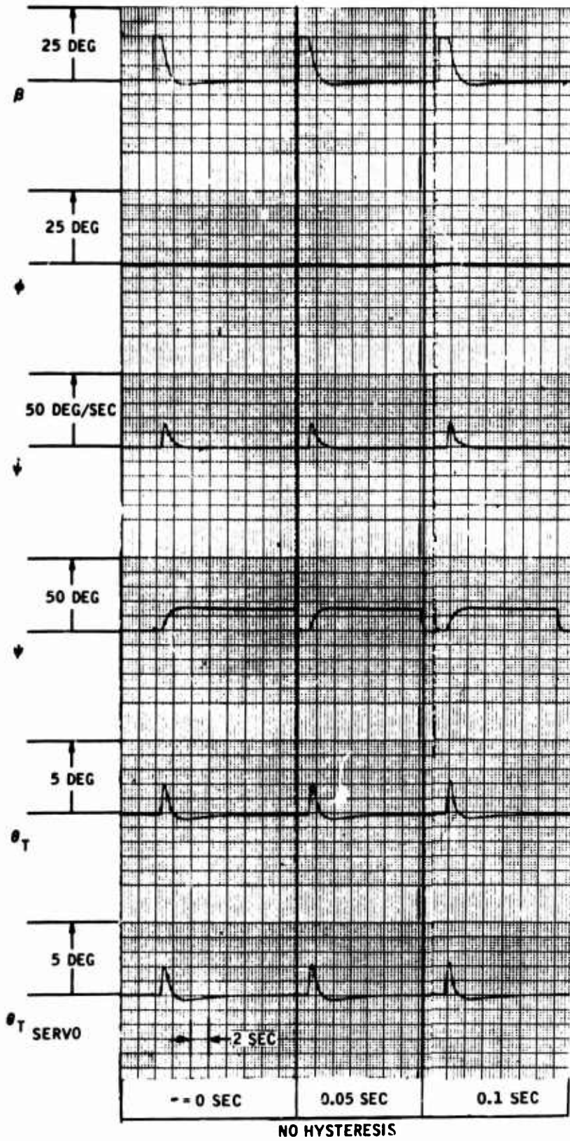
YAW RATE SENSOR TRANSPORT LAG
