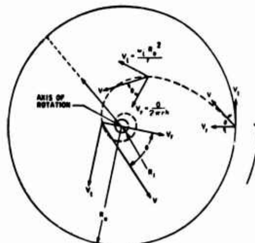
Figure 30. Vortex Rate Sensor Flow Fields
