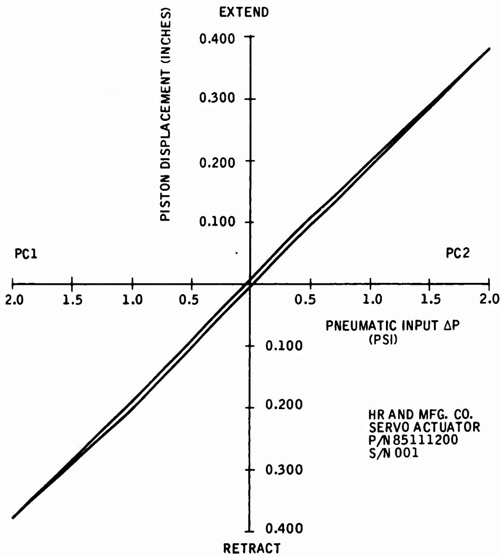
Figure 48. Actuator Displacement Versus Pneumatic Input (S/N 0.001)
