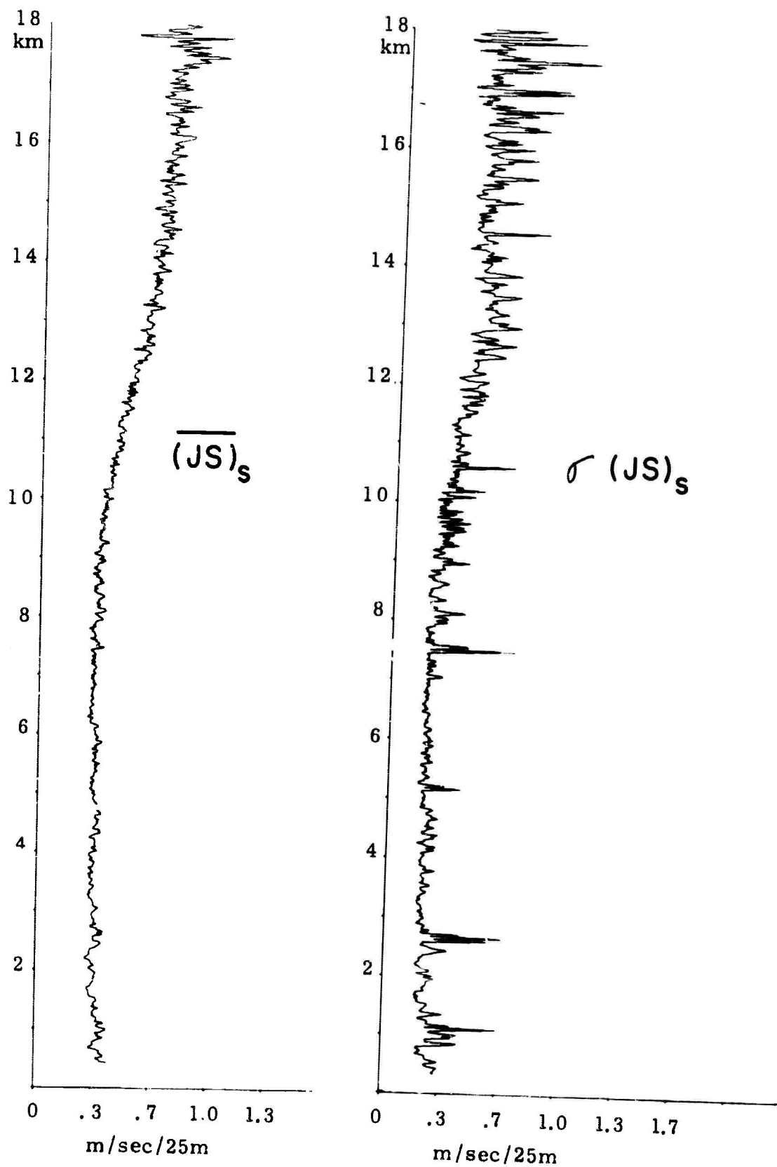
Figs. 21 and 22. Mean and standard deviation of Jimsphere shear.
