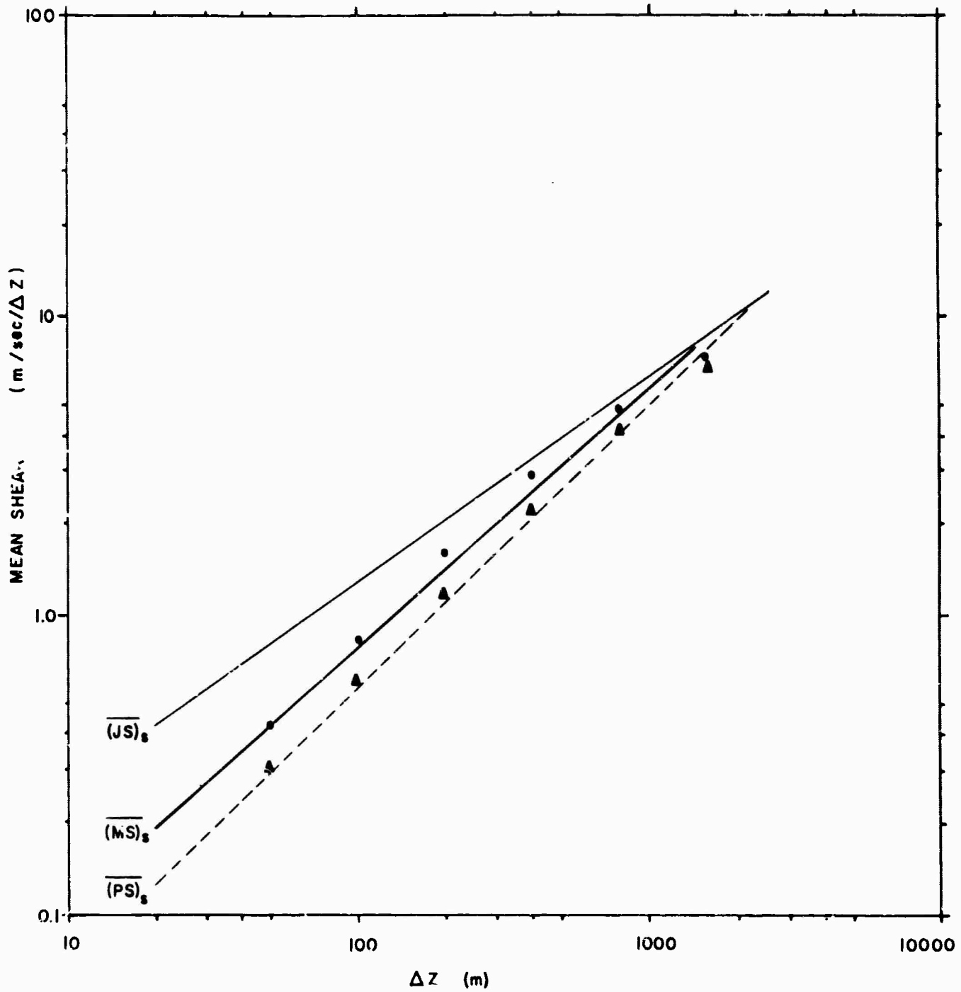
Fig. 16 Comparison of Jinsphere shear, pressure shear and minute shear to layer thickness
