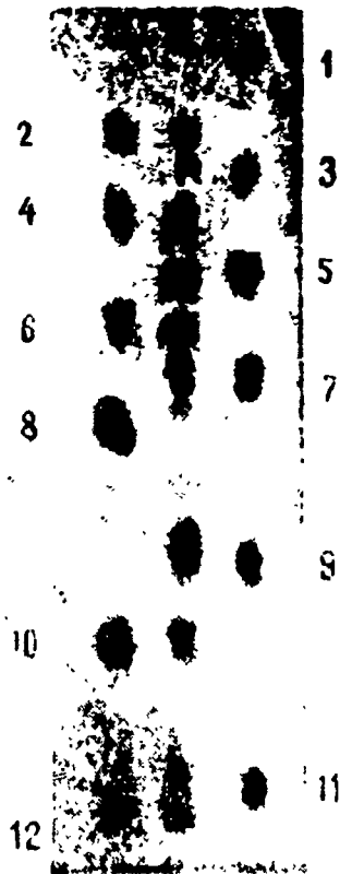
Drawing 2. Chromatogram of the amino-acid composition of chemical anthraxin (in the center). To the left and right evidence of (1) cystine; (2) lysine; (3) arginine; (4) aspariginic acid; (5) glycocoll; (6) glutamic acid; (7) threonine; (8) proline; (9) thyrosine; (10) valine; (11) phenylalanine; (12) leucine.
