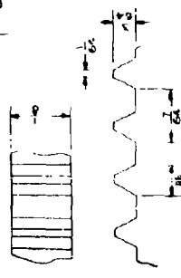
FITTING THE DETAIL PITCH FROM HEEL BREAST TO HEEL BREAST SCALE 2:1
