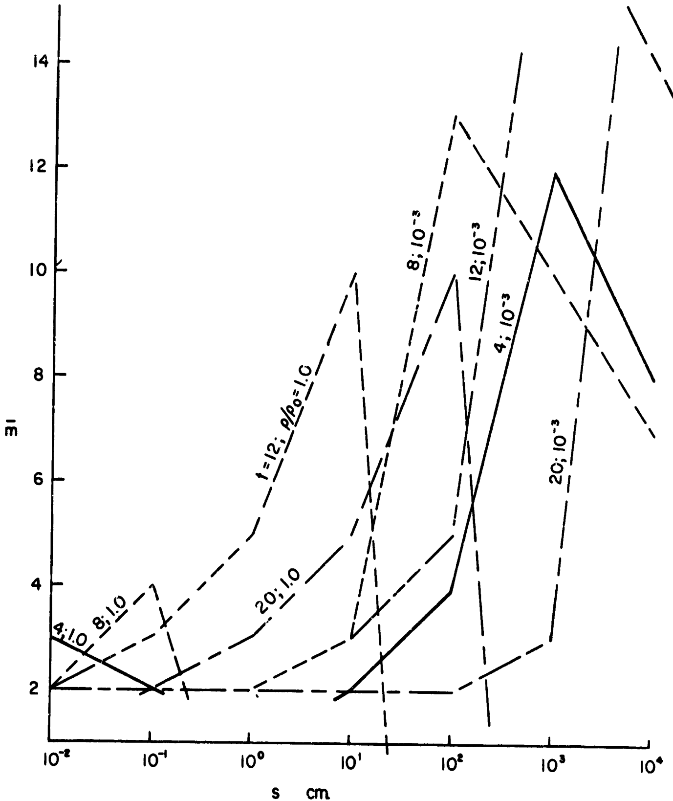
FIG. 10 LOWER STATE QUANTUM NUMBER OF FIRST COMPLETELY MERGED OR THIN SERIES. ONLY VALUE FOR WHICH THE PATH LENGTH IS AN INTEGER POWER OF 10 HAVE MEANING.
