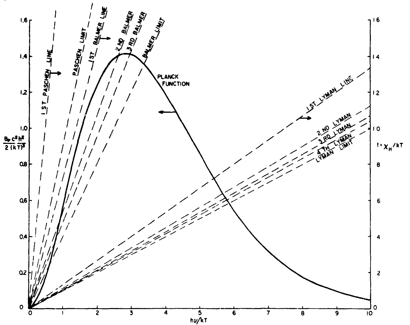
FIG. 2 PLANCK BLACK-BODY FUNCTION AND THE RELATIVE POSITIONS OF SEVERAL STRONG LINES.
