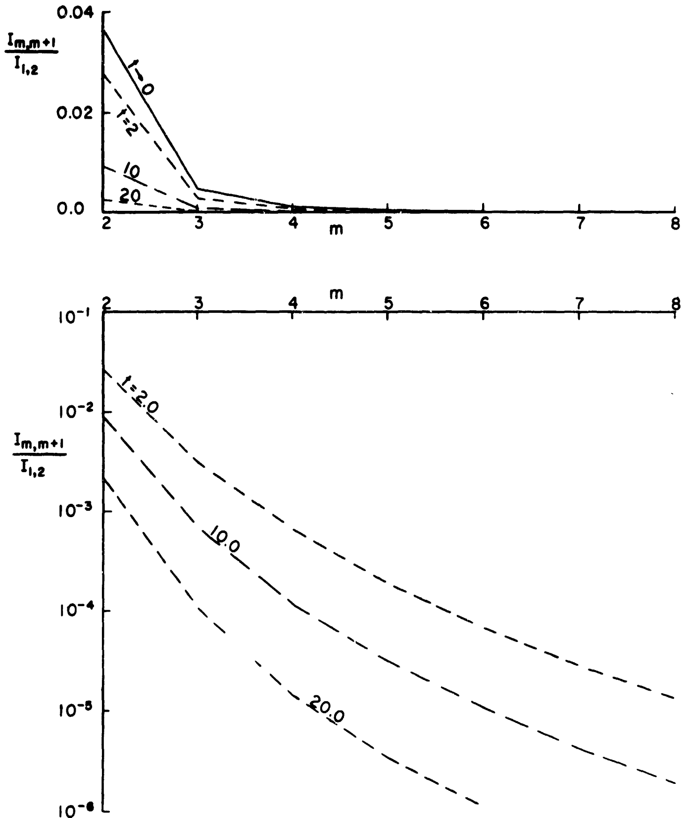
FIG. 4 INTENSITY OF LEADING LINE RELATIVE TO RESONANCE LINE AS A FUNCTION OF LOWER STATE QUANTUM NUMBER AND INVERSE TEMPERATURE PARAMETER FOR NONABSORBED LINES.
