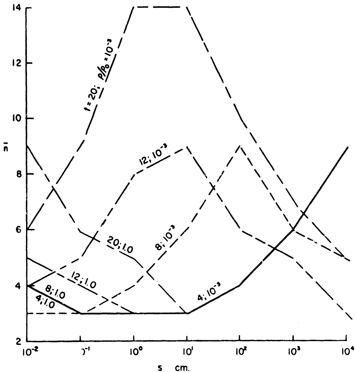
FIG. 80 UPPER STATE QUANTUM NUMBER OF FIRST MERGED OR THIN LINE. ONLY VALUES FOR WHICH THE PATH LENGTH IS AN INTEGER POWER OF 10 HAVE MEANING. m = 1
