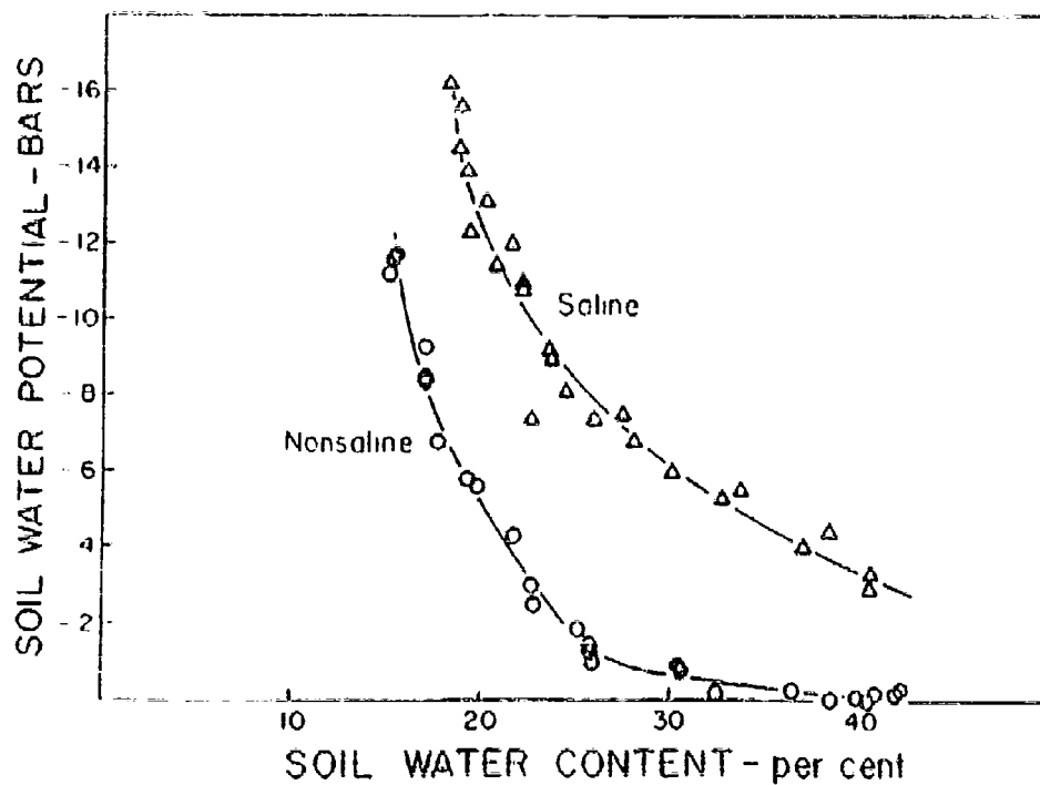
Figure 1.--Soil water potential as a function of soil water content. Deionized water or saline water (with an osmotic potential of -2.0 bars) was applied to Chino clay.
