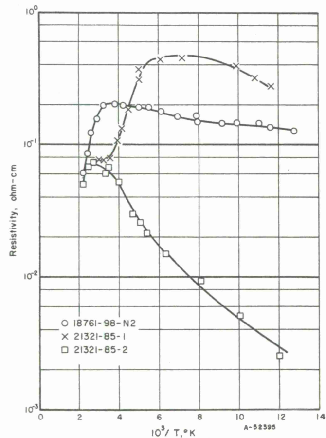
FIGURE 3. RESISTIVITY AS A FUNCTION OF RECIPROCAL TEMPERATURE FOR VARIOUS AS-GROWN PT-DOPED CRYSTALS OF \text{PbTe}
