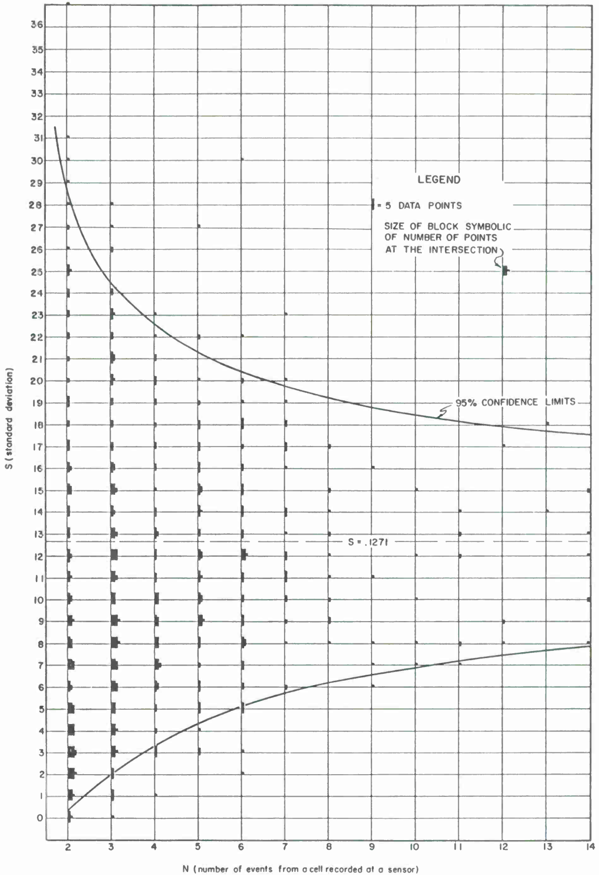
Figure 6. Distribution of Standard Deviation Estimates Computed from N Events
