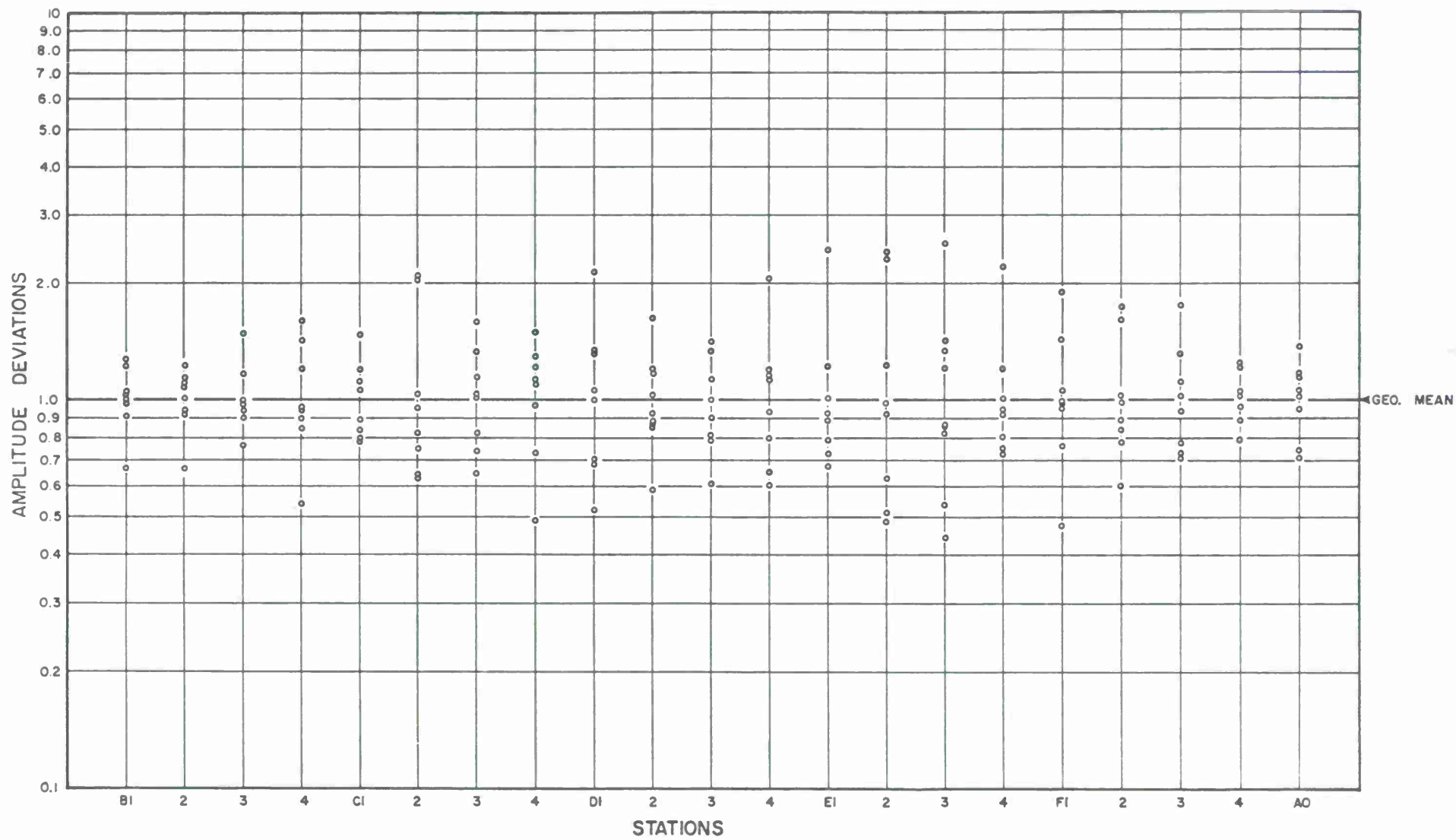
Figure A-2. Eight Fiji Island Events Showing Deviations about the Mean Amplitudes
