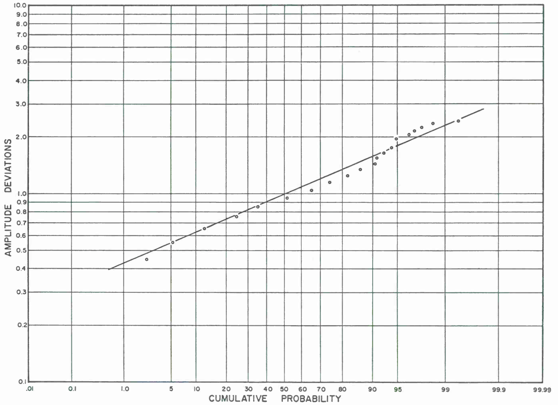
Figure A-3 Distributions of the Amplitude Deviations of Eight Fiji Island Events
