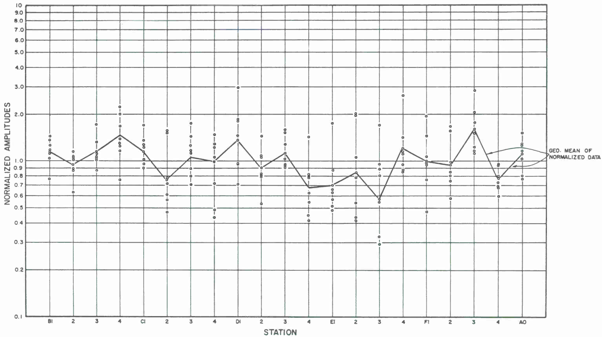
Figure A-1. Eight Fiji Island Events - Normalized and Showing the Means for Each Station
