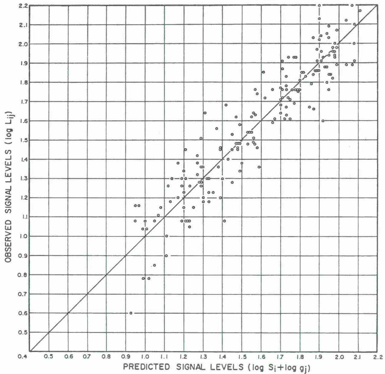
Figure A-4. Observed versus Predicted Signal Levels - 8 Fiji Island Events. Using a Product Error Model with Zero Additive Noise Assumed.
