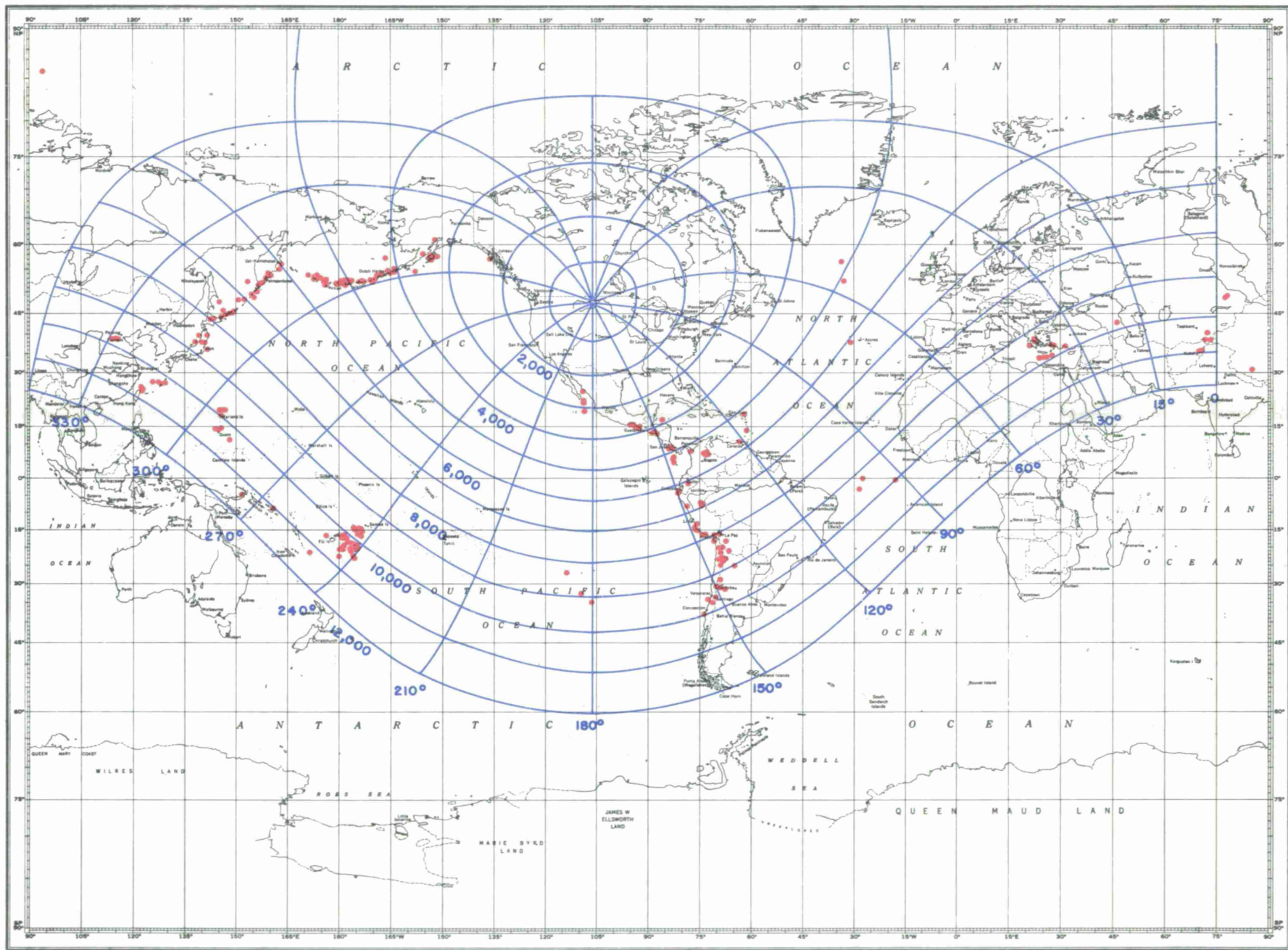
Figure 1. Event Location Chart with Distance-Azimuth Grid (Distance in Kilometers, Azimuth in Degrees)
