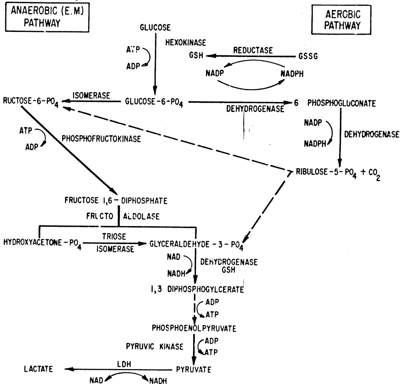
Figure 2. PATHWAYS OF GLUCOSE METABOLISM IN THE ERYTHROCYTE
