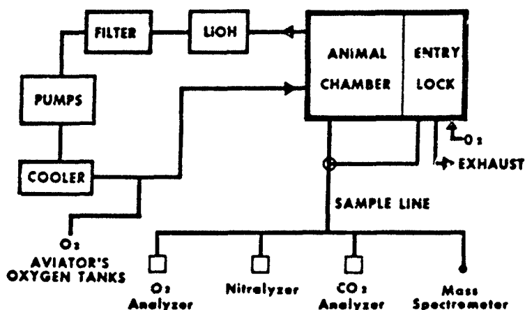
Figure 1. BLOCK DIAGRAM OF CHAMBER FACILITIES. Direction of flow of atmosphere is indicated by arrows.
