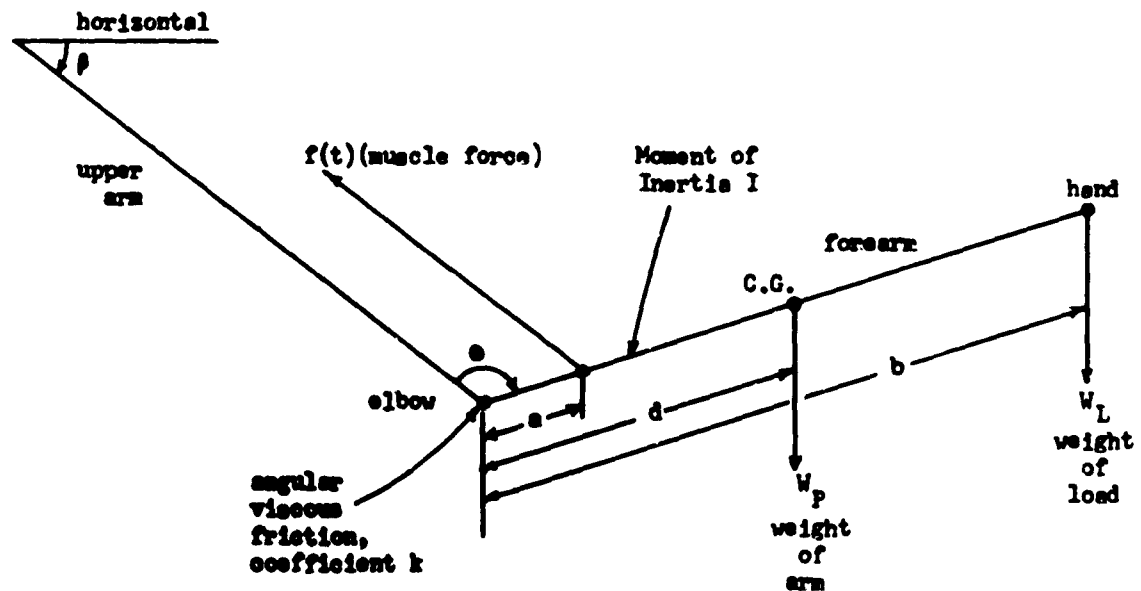
Fig. 14. Idealized arm model used in simulation
