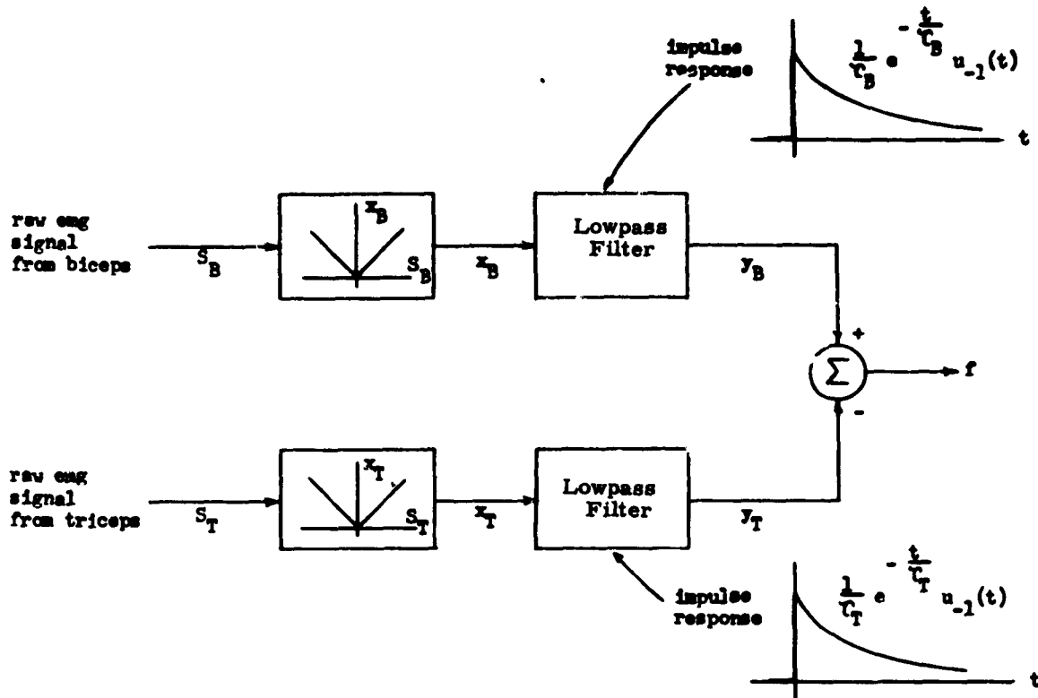
Fig. 15. Block diagram of the emg signal processing
