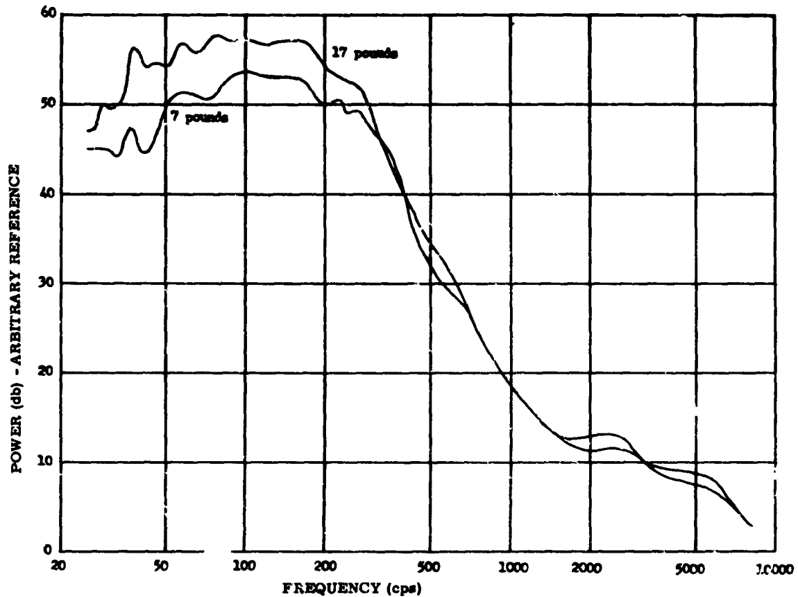
Fig. 12. Power spectra for needle emg signals
