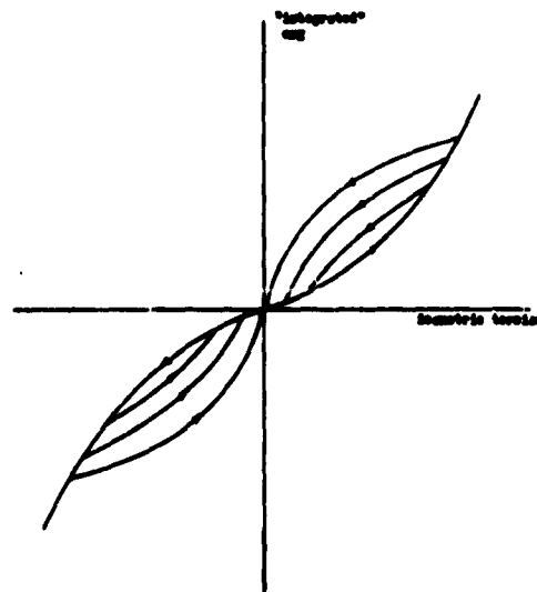
Fig. 13. Multiple-valued nonlinear emg-force relation. Biceps and Triceps surface electrodes. Integrator time constants 300 ms. Relation is qualitative only. Tension measure at hand, elbow angle 90°.
