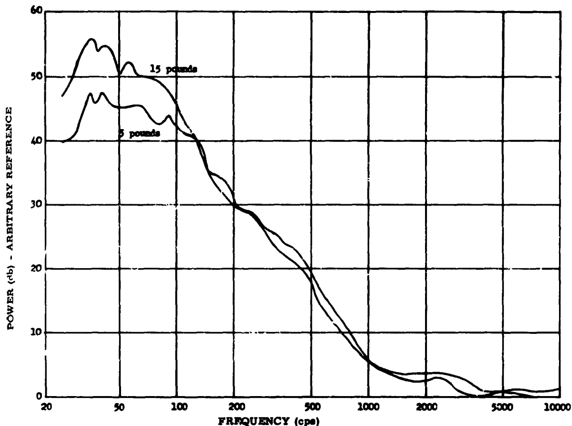
Fig. 11. Power spectra for surface emg signals
