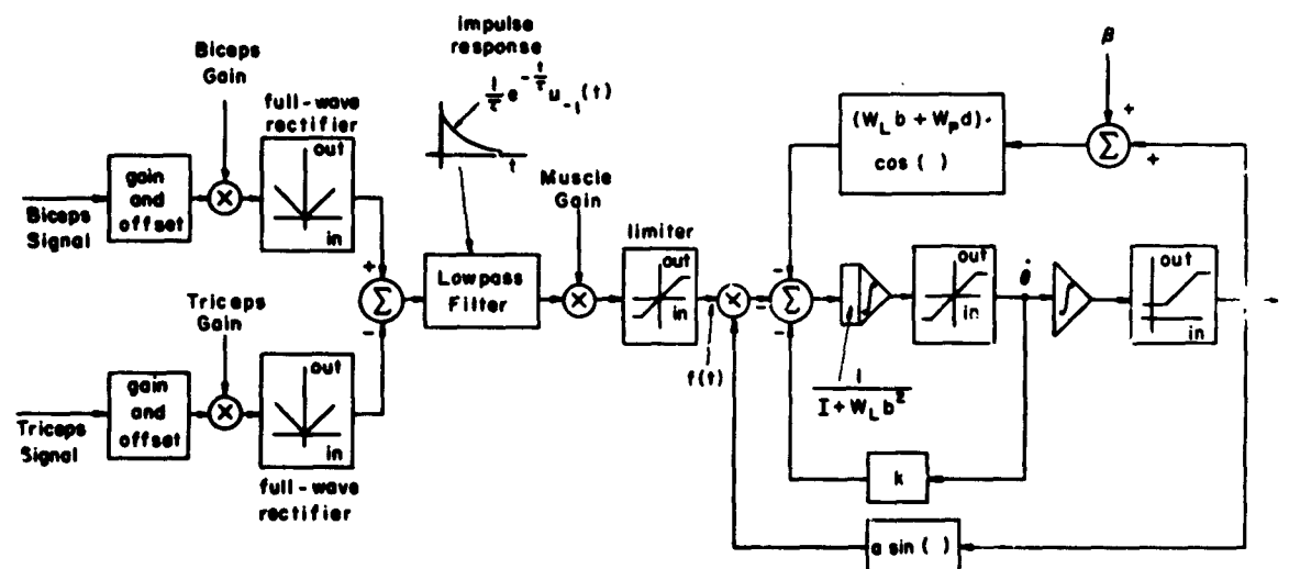
Fig. 16. Block diagram of over-all simulation program
