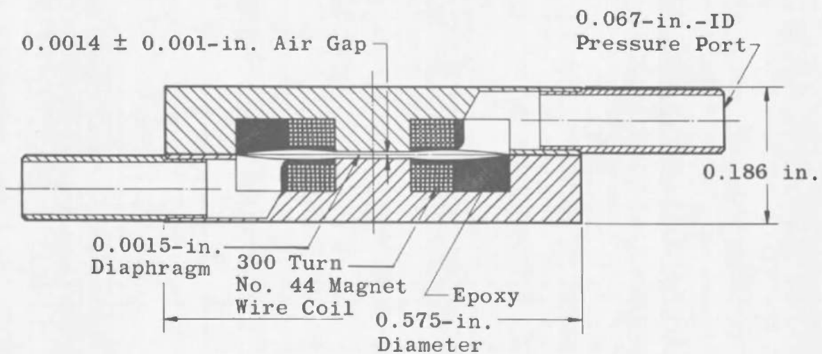
Cross Section
