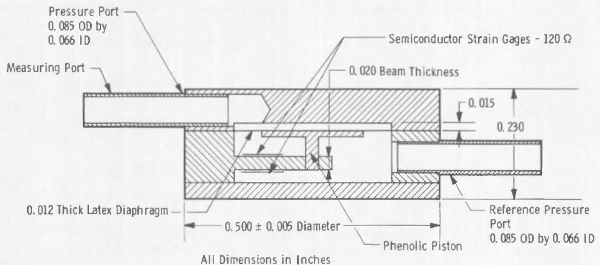
Fig. 6 Semiconductor Wafer Gage Assembly
