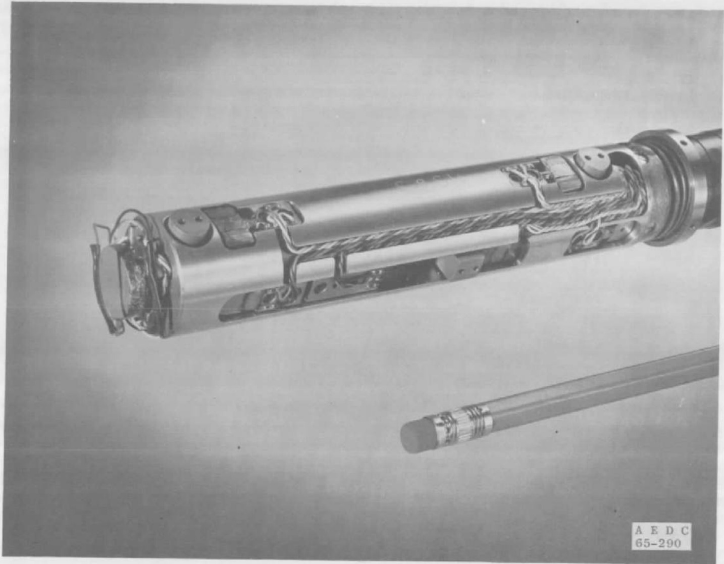
Fig. 10 Six-Component Balance Assembly
