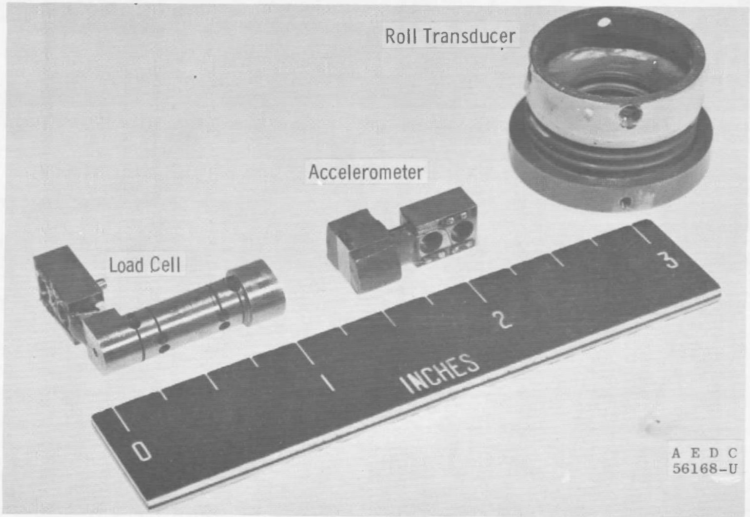
Fig. 11 Balance Components
