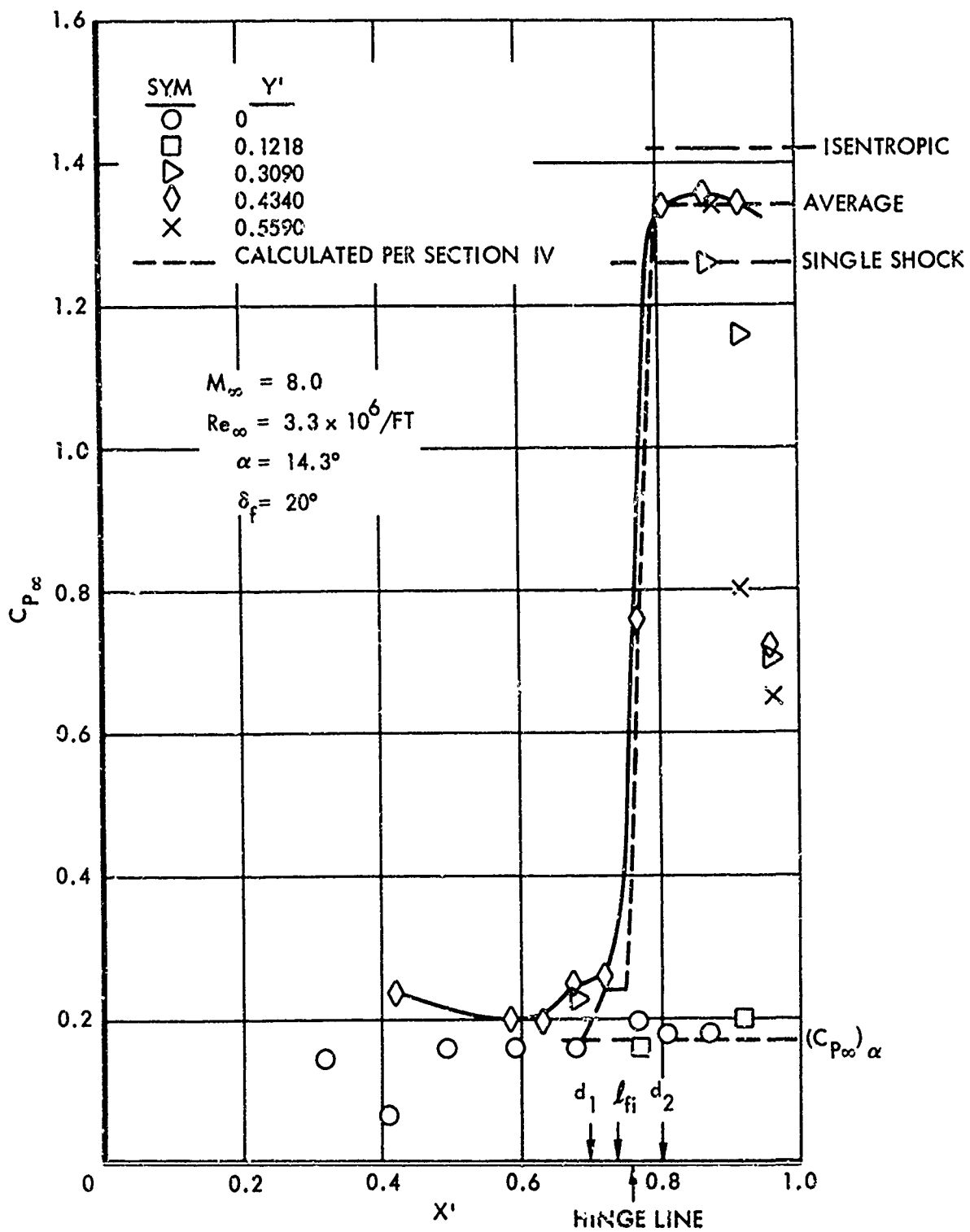
Figure 89. Pressure Distribution Over Pyramidal Configuration (Flat Bottom Surface), Re_\infty = 3.3 \times 10^6/ft
