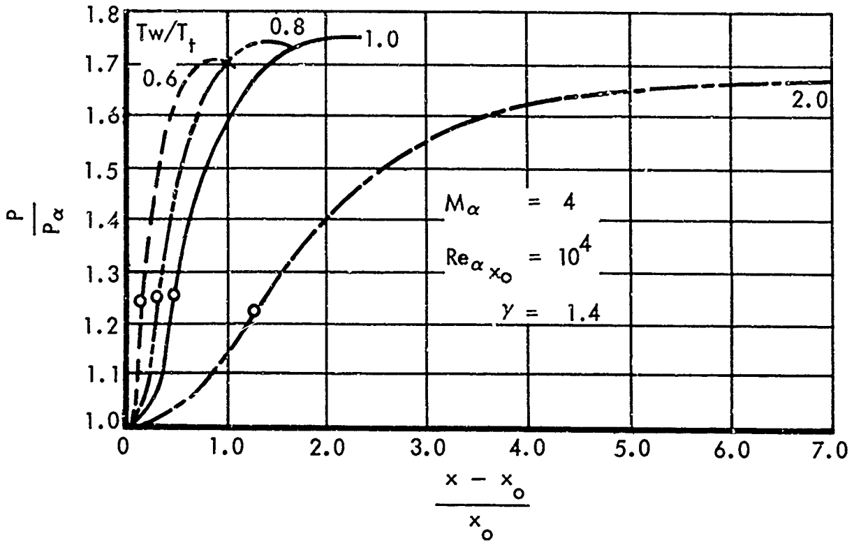
Figure 9. Wall Temperature Effect on Pressure Distribution in Separated Flow over a Curved Surface (Reference 28)
