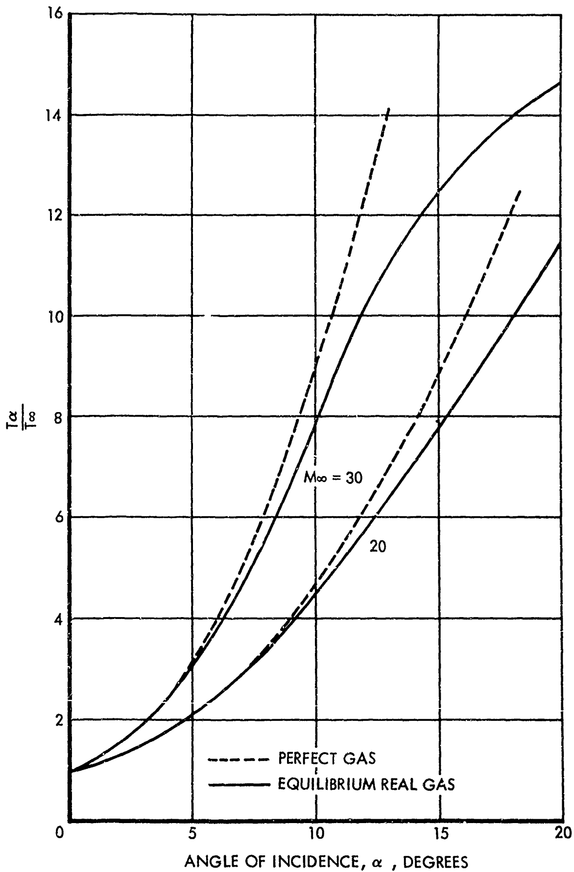
Figure 97. Oblique Shock Temperature Ratio Including Real Gas Effects (Concluded)
