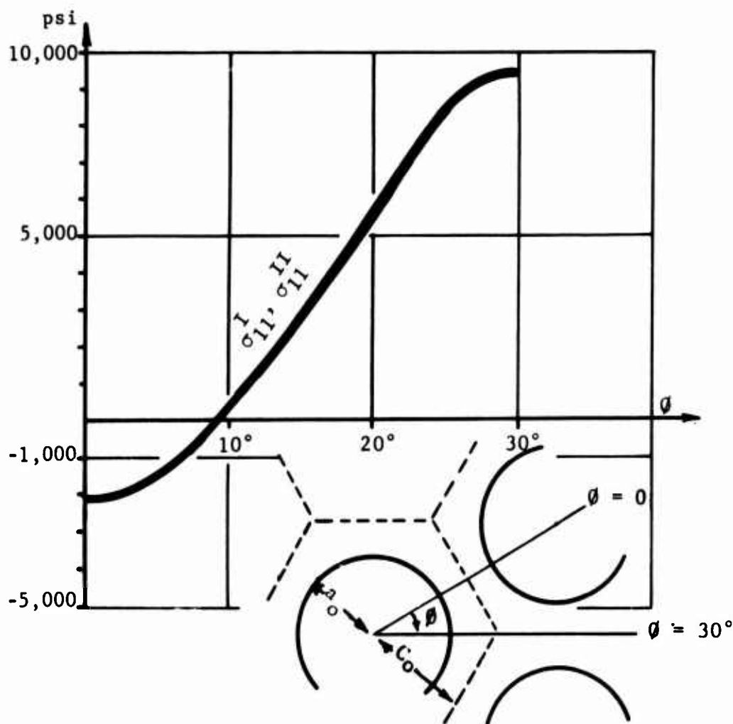
Figure 11. Radial Shrinkage Stresses at Interface in a Multifiber Composite Model a_0 = 0.14 inch; C_0 = 0.2 inch (Components: glass and epoxy)
