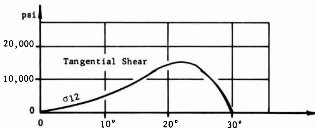
Figure 12. Shear Stress at Interface Due to Shrinkage a_0 = 0.14 inch; C_0 = 0.2 inch (Components: glass and epoxy)
