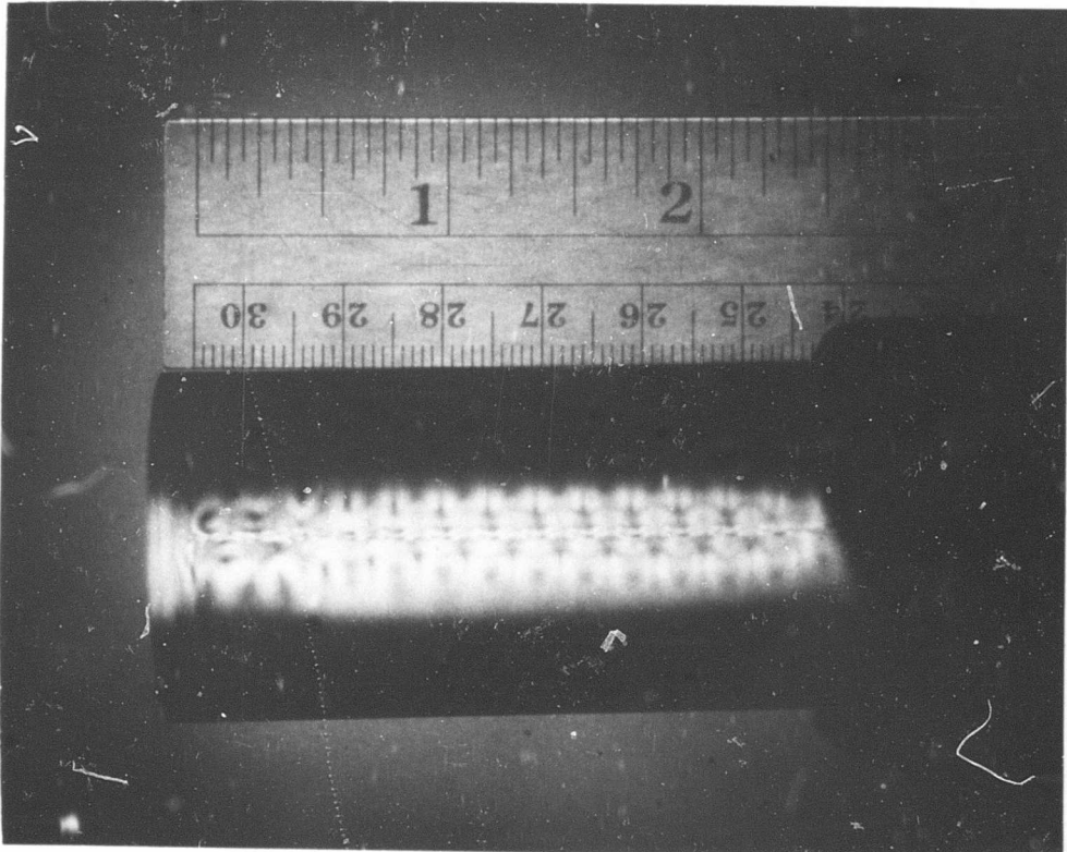
Figure 17. Glass Fiber (0.005-inch Diameter) in an Epoxy Resin Cylinder Viewed under Polarized Light (Quarter wave plates are in the optic system)
