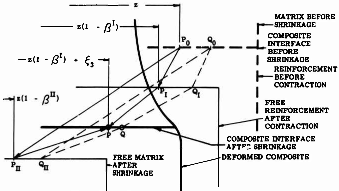
(c) View A (Enlarged) Showing Combined Shrinkage in Relation to Independent Shrinkage of Both Materials
