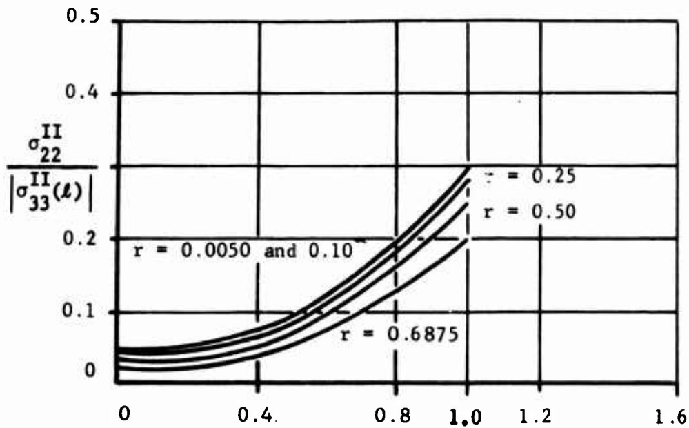
Figure 7. Tangential Stress in the Resin Produced by Load \sigma_{33}^{II}(l) at the Resin End z = 1.5 inches (single-fiber composite)
