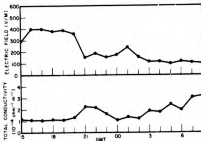
Fig. 8 - Failure in forecasting dissipation, Argentia, Newfoundland; June 24 and 25, 1958
