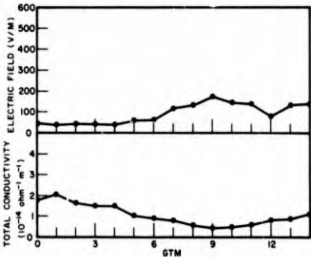
Fig. 3 - Example of successful forecast of onset and dissipation of fog, Lakehurst, New Jersey, May 12, 1962
