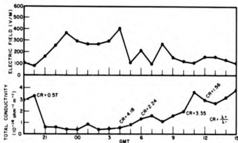
Fig. 11 - Example of low conductivity and high field in fog and rain (drizzle), Argentina, Newfoundland, Mar. 10 and 11, 1958
