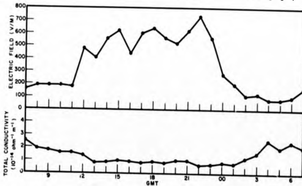
Fig. 4 - Example of successful forecast of onset and dissipation of fog, Argentia, Newfoundland, Aug. 4 and 5, 1958
