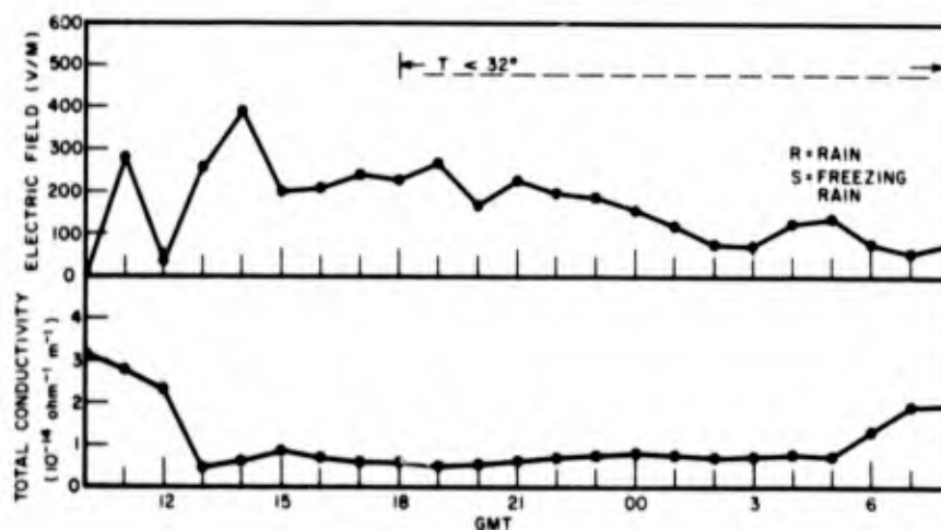
Fig. 10 - Occasion of fog, rain, and freezing rain, Argentina, Newfoundland, Mar. 7 and 8, 1959
