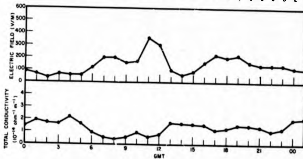
Fig. 5 - Example of successful forecast of onset and dissipation of fog, Pensacola, Florida, Mar. 25, 1959
