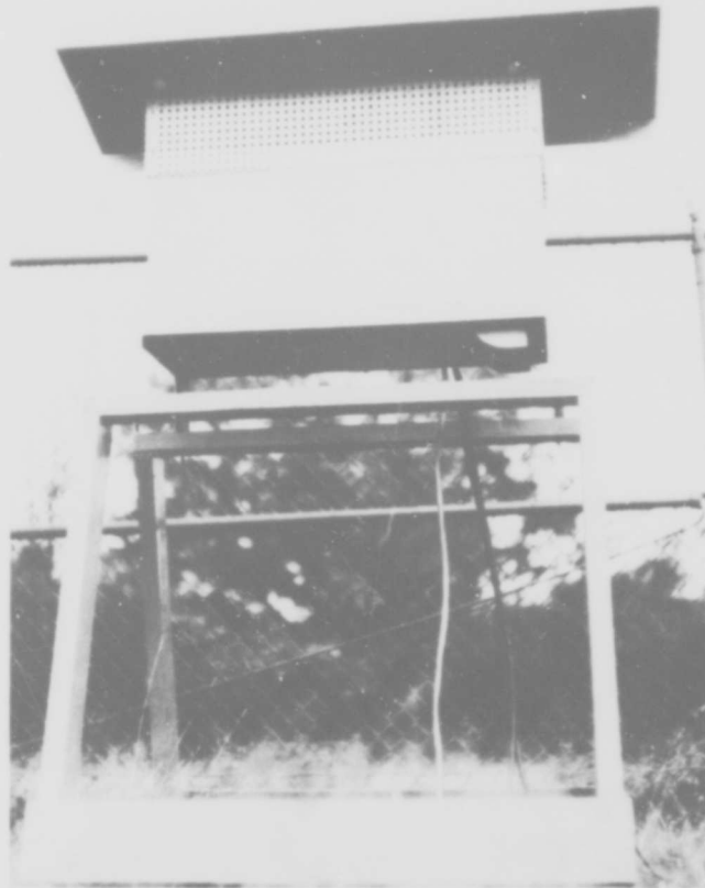
Fig. 14 - Overall view of total-conductivity chamber showing air-inlet scoops and exhaust ports
