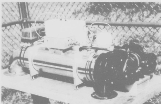
Fig. 15 - Interior view of total-conductivity chamber, with insulation and temperature control
