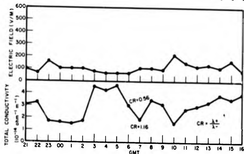
Fig. 12 - Example of high conductivity and low field in fog and rain (drizzle), conductivity unstable, Argentinia, Newfoundland, Mar. 11 and 12, 1958
