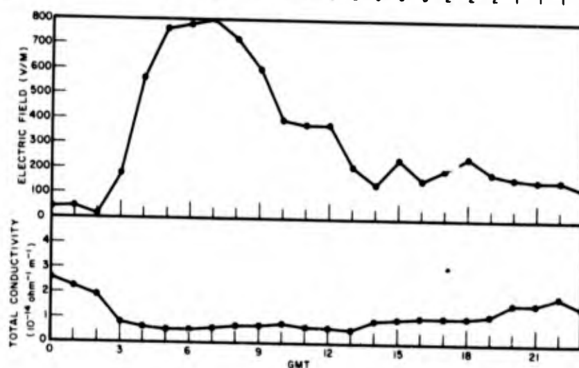
Fig. 13 - Example where fog onset could have been predicted even in rain, Argentinia, Newfoundland, Aug. 26, 1958
