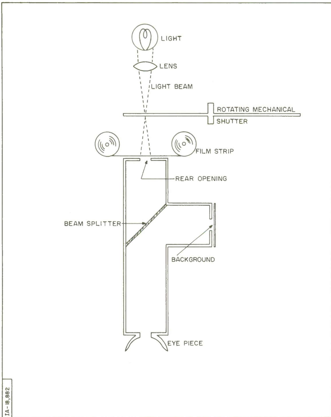
Figure 5. The Tachistoscope
