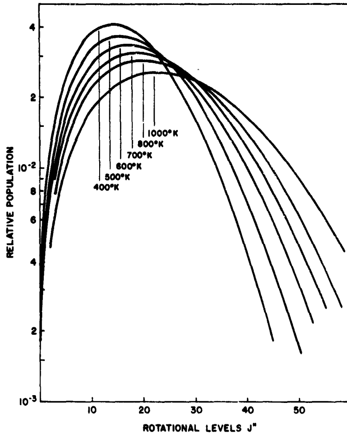
Figure 4. Rotational Population of the Ground Vibrational Level v'' = 0 of AlO
