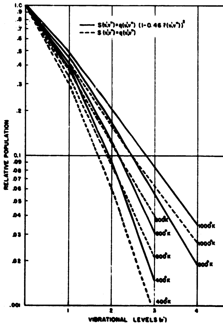
Figure 6. Population of the Upper States for Various Temperatures
