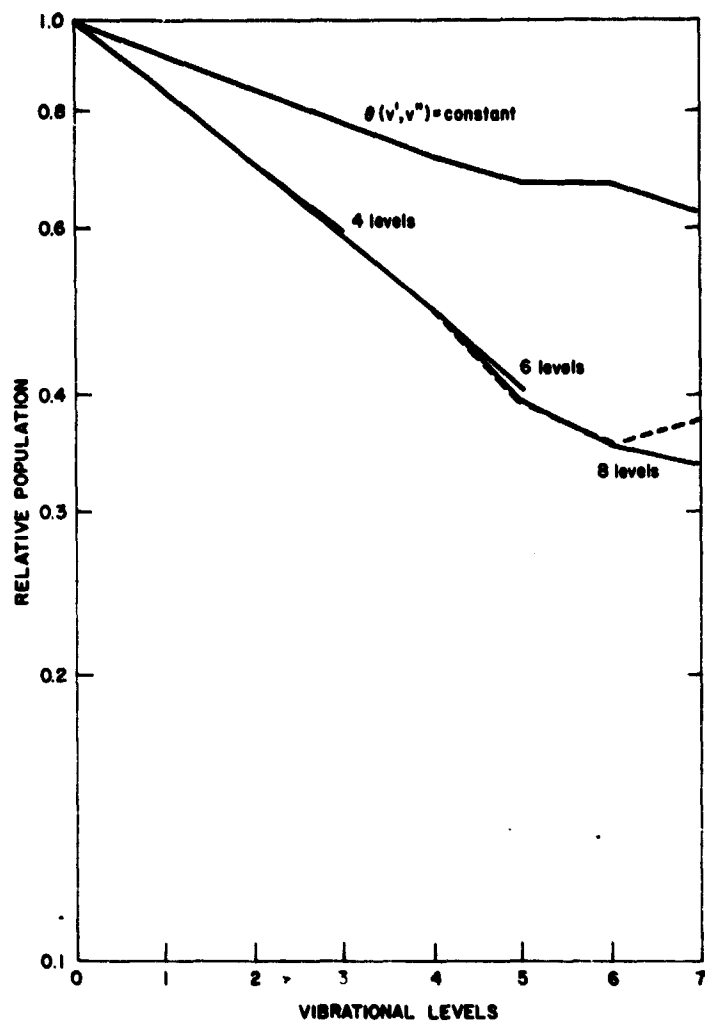
Figure 13. Relative Population for the Case Where Lower Levels are not Thermalized
