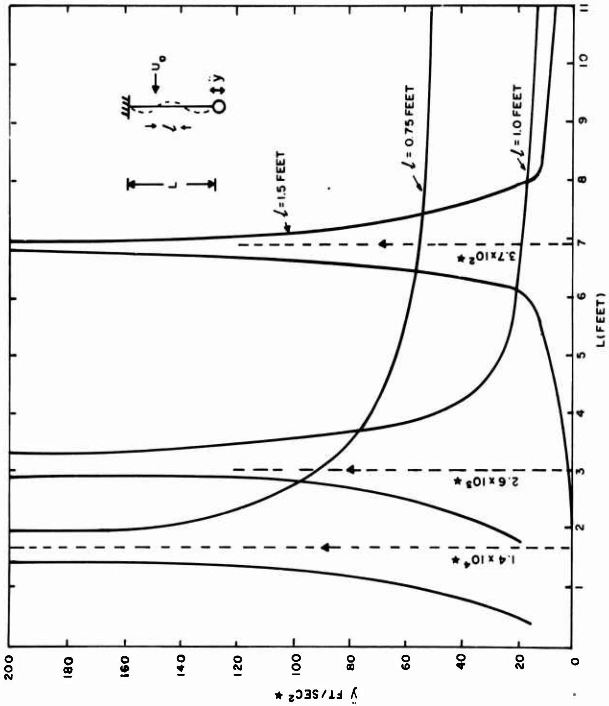
FIGURE 7 - Experimental Motion Response of the Terminal Mass to Cable Strumming Forces
