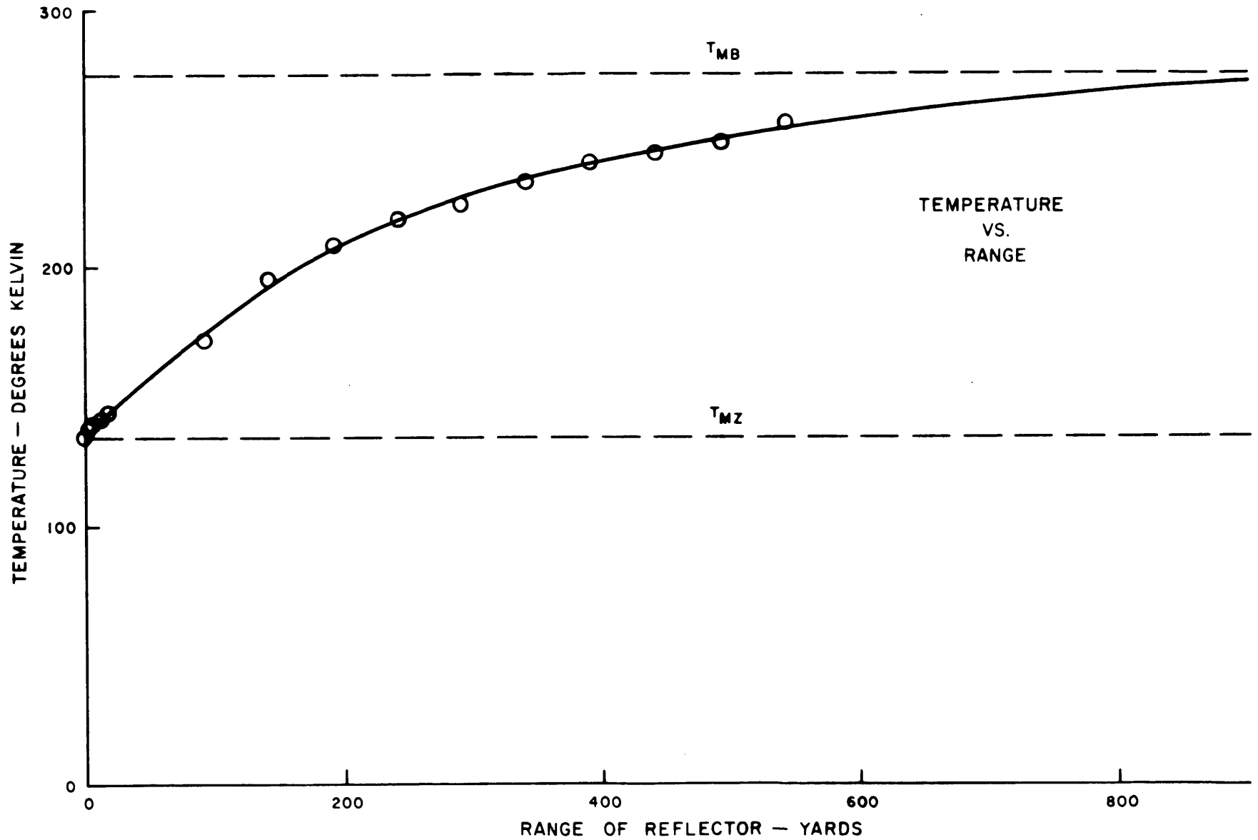
FIGURE 19. MEASURED DATA FOR RUN 8.
