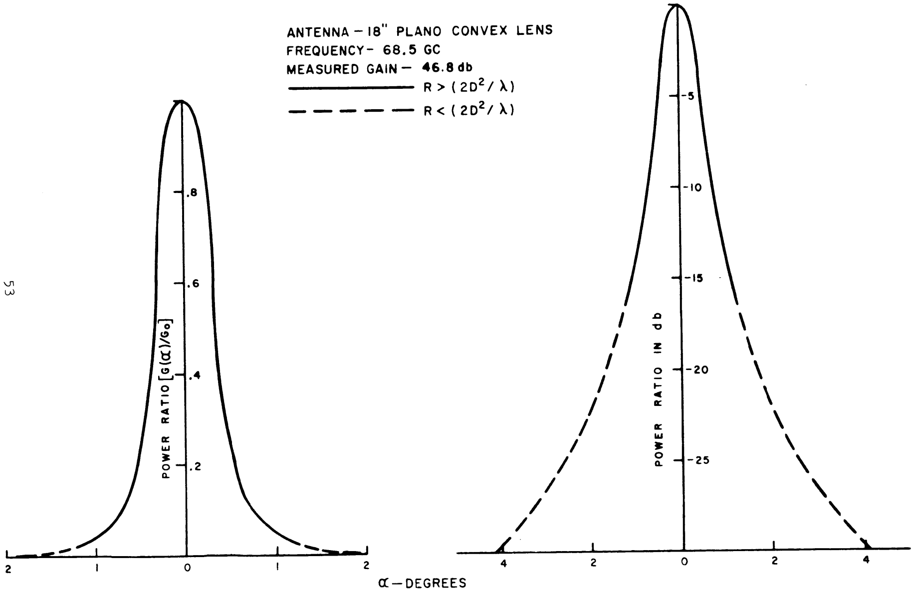
FIGURE 6. NORMALIZED EFFECTIVE POWER PATTERN FOR RUN I.
