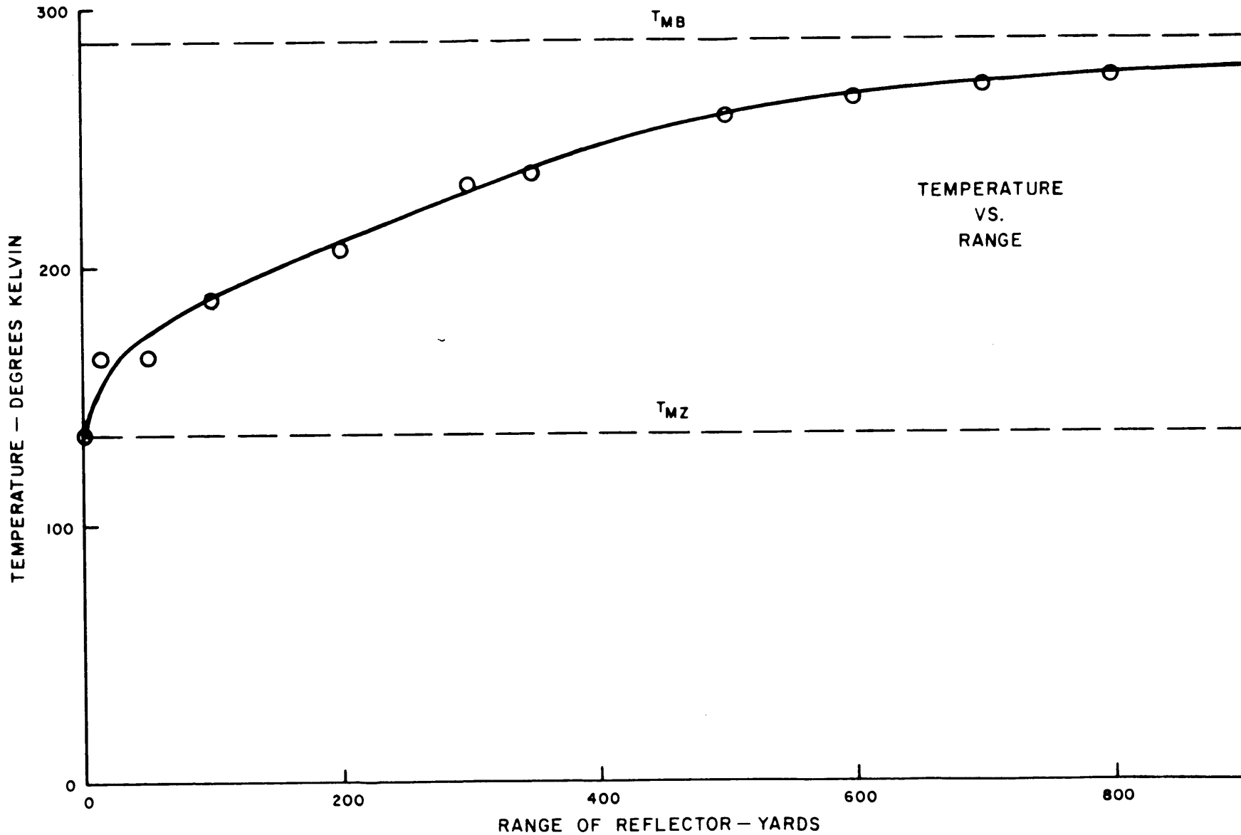
FIGURE II. MEASURED DATA FOR RUN 4.
