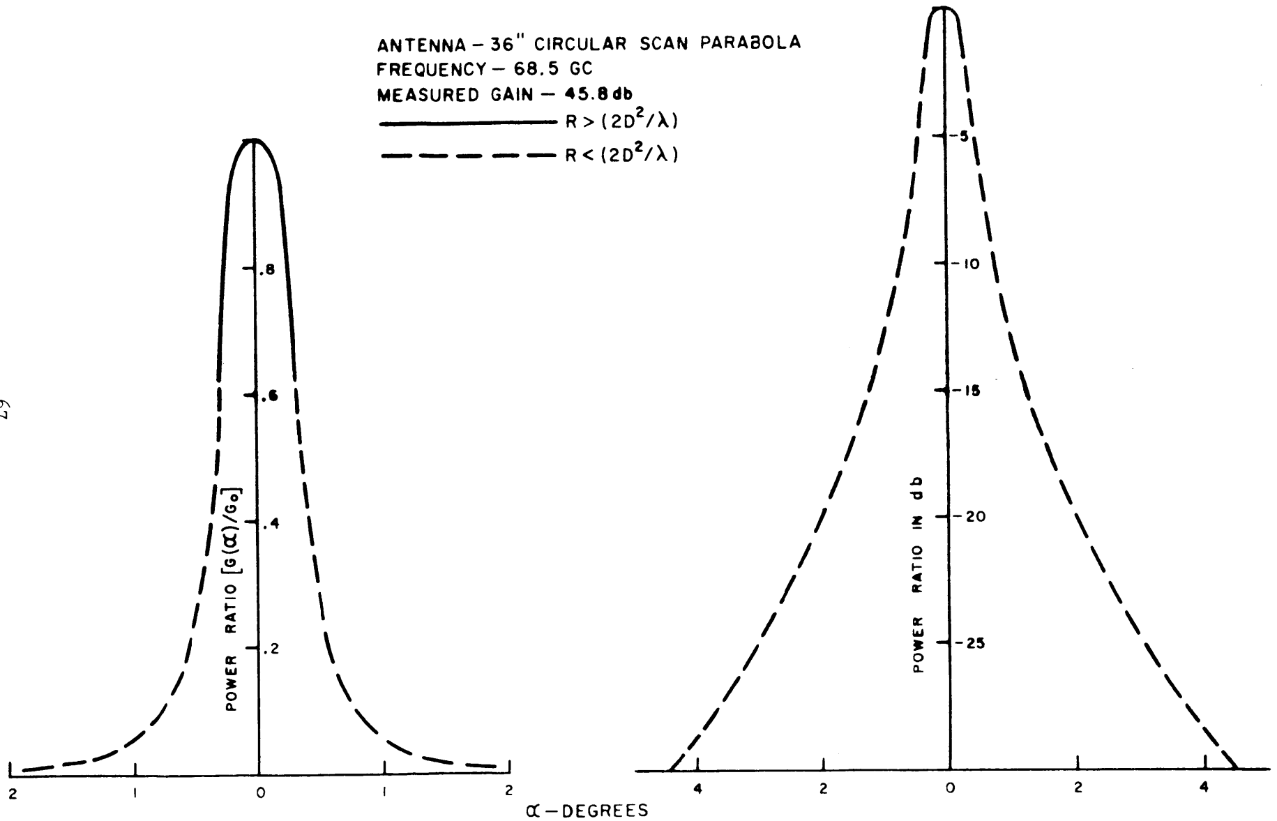
FIGURE 20. NORMALIZED EFFECTIVE POWER PATTERN FOR RUN 8.
