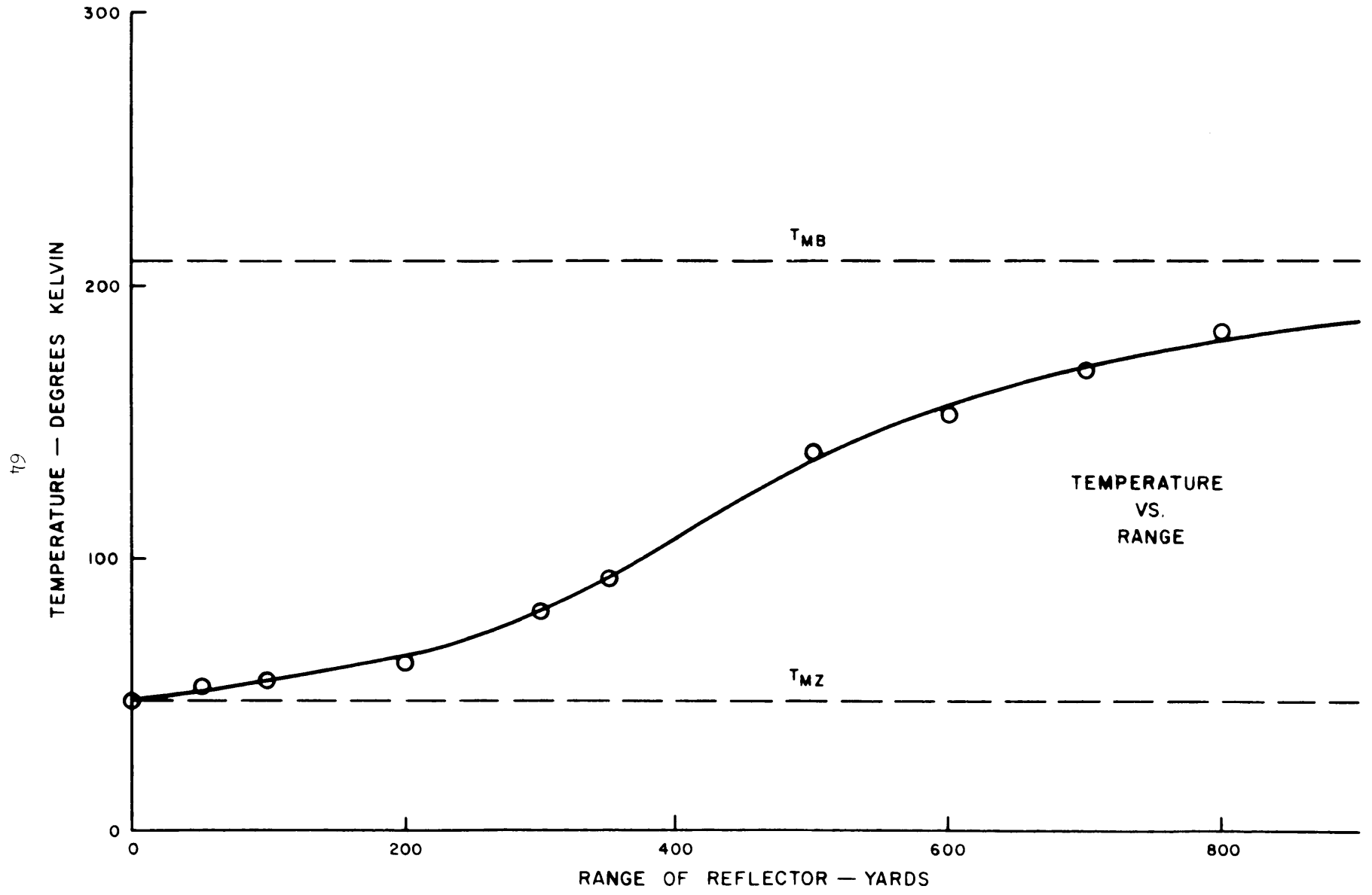
FIGURE 17. MEASURED DATA FOR RUN 7.
