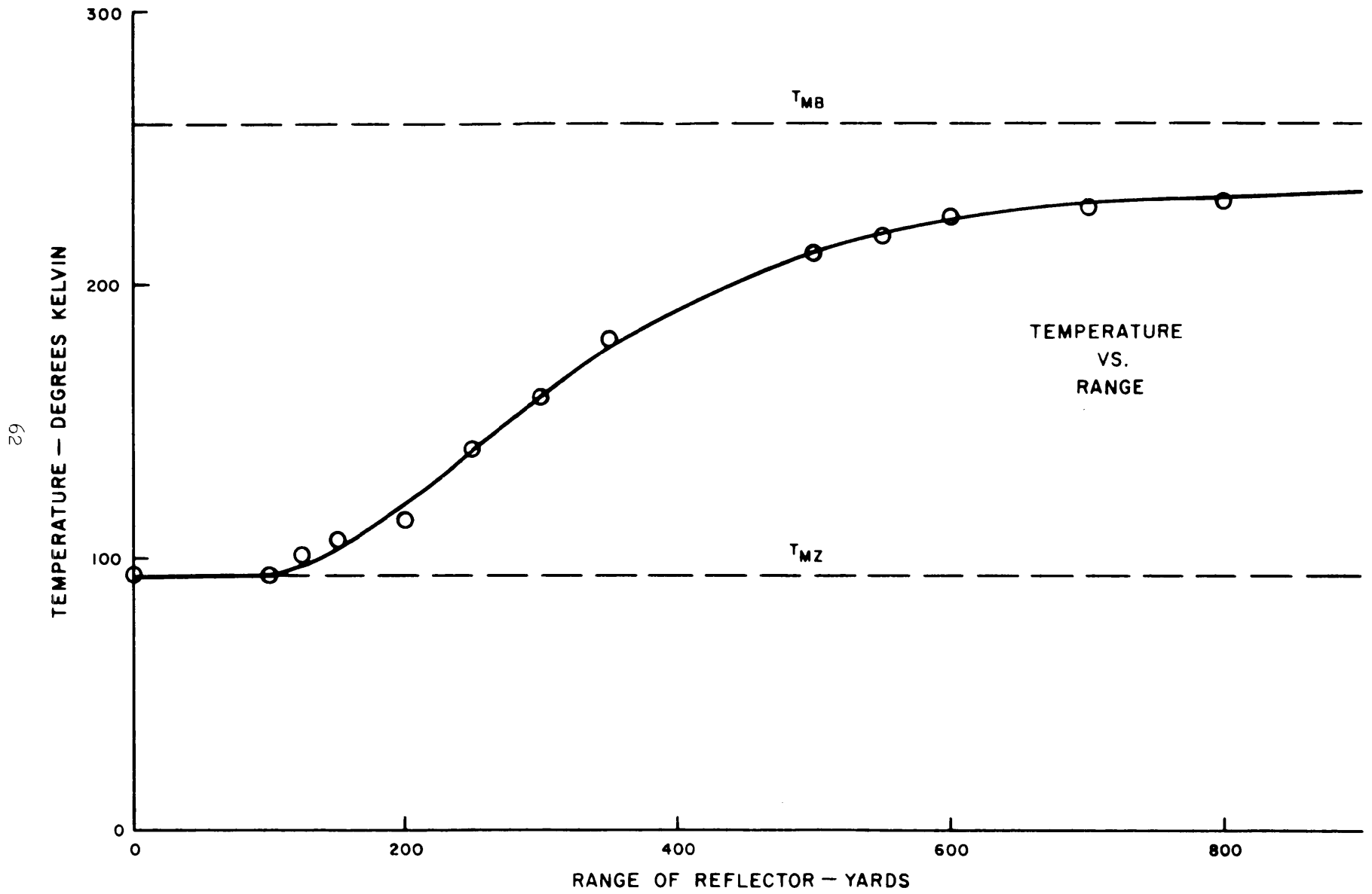
FIGURE 15. MEASURED DATA FOR RUN 6.
