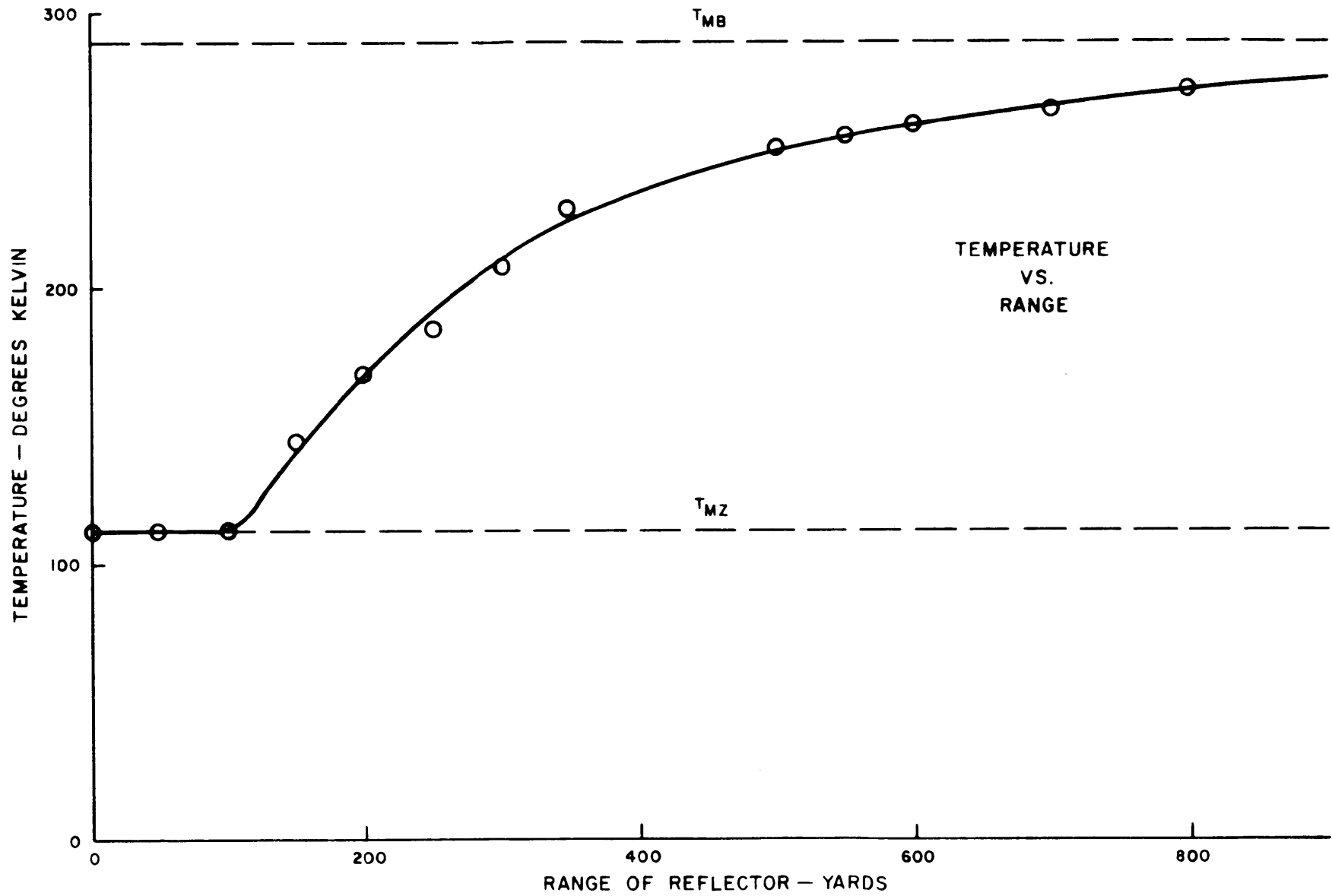
FIGURE 9. MEASURED DATA FOR RUN 3.
