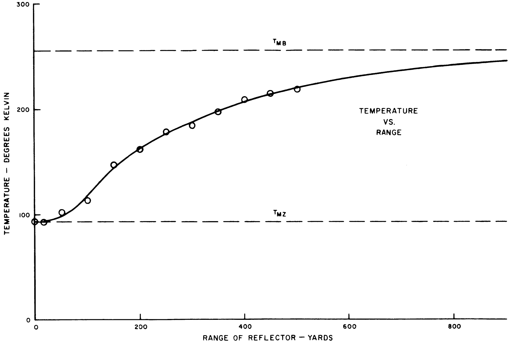
FIGURE 5. MEASURED DATA FOR RUN I.
