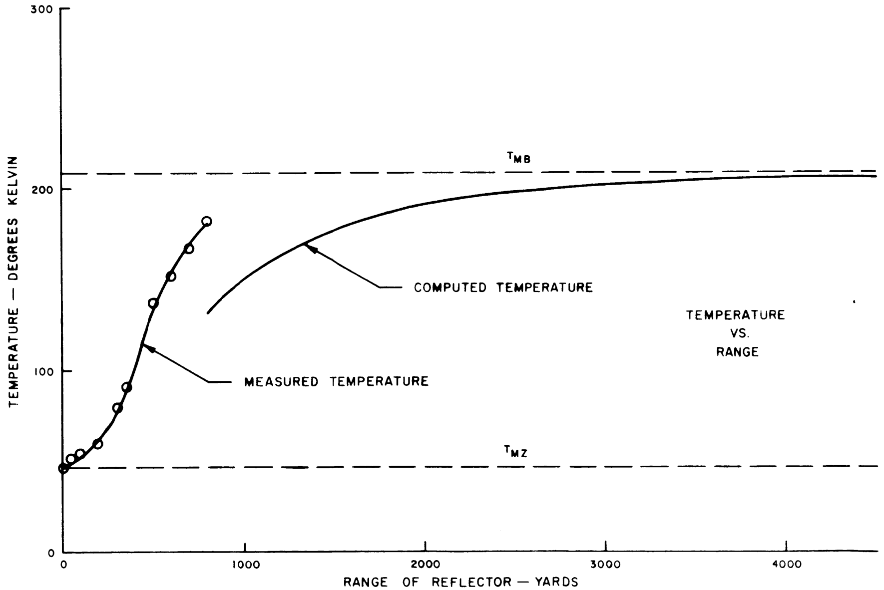
FIGURE 21. COMPARISON OF MEASURED DATA WITH TEMPERATURES COMPUTED FOR ANTENNA WITH 54.2 db GAIN AND 0.24° B.W.
