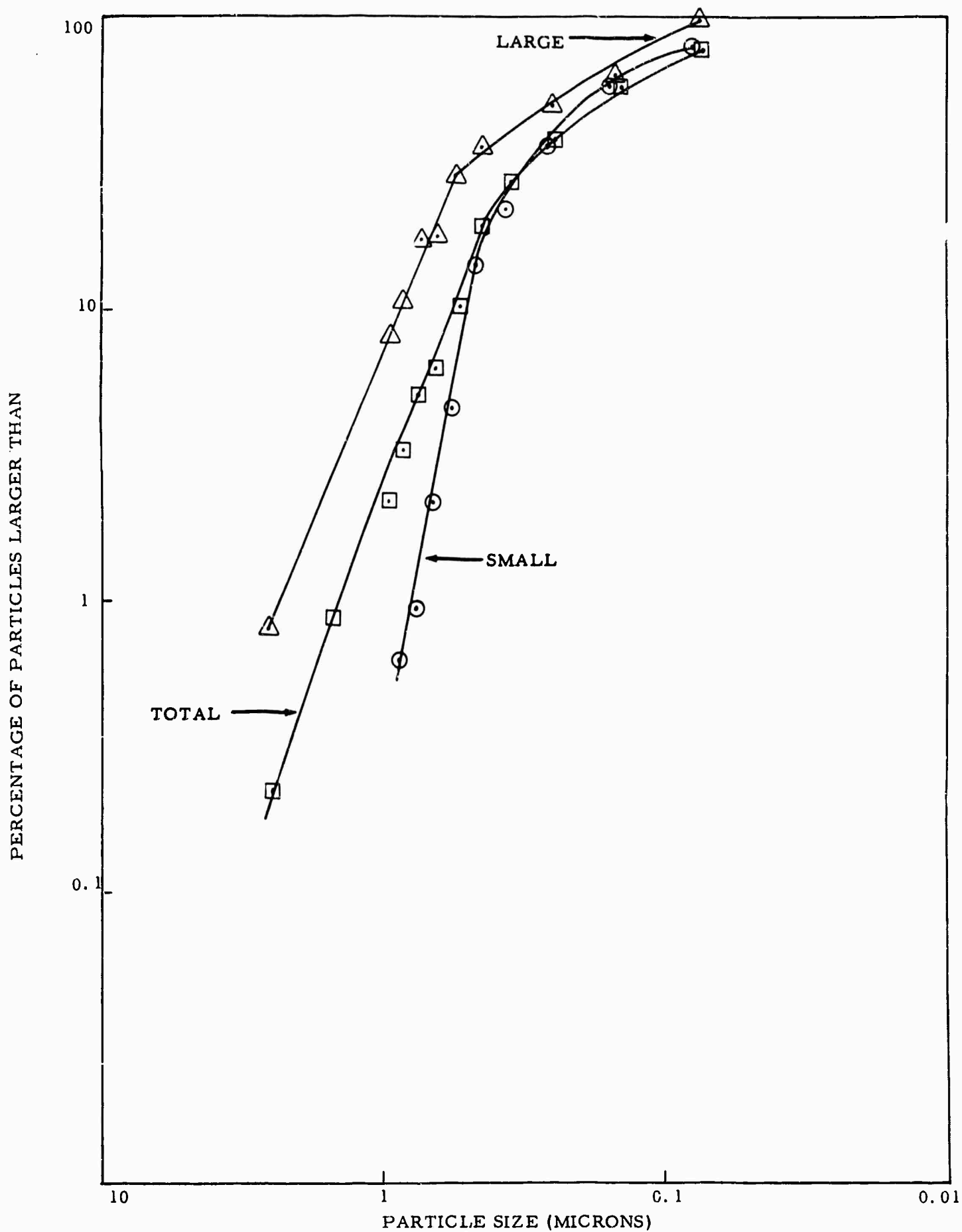
Fig. 8 Particle size analysis for phenolic graphite. This intergal distribution curve for material shown in Figure 5 is obtained from the data plotted in Figure 7.
