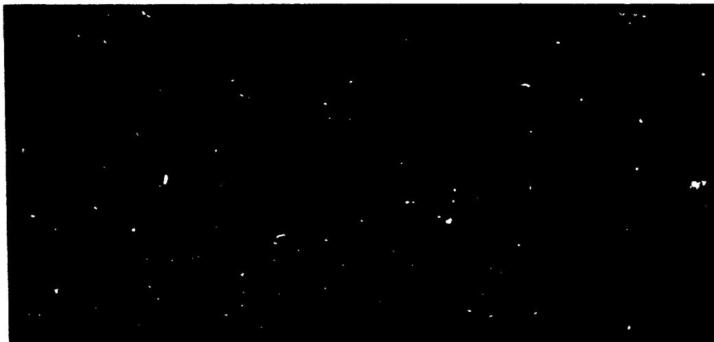
FIG. 3. The effect of various reagents on the activity of PI and Pli tested on NZA.1. A, No addition; B, 0.1 \text{ M Ca}^{++} (top layer) plus 750 \text{ } \mu\text{M Fe}^{+++} (top layer) and 0.8 \text{ M citrate} (top layer); C, 0.028 \text{ M PO}_4^{=} (basal layer); D, 0.028 \text{ M PO}_4^{=} (basal layer) and 0.8 \text{ M citrate} (top layer); E, 0.1 \text{ M Ca}^{++} (top layer) and 750 \text{ } \mu\text{M Fe}^{+++} (top layer); F, 750 \text{ } \mu\text{M Fe}^{+++} (top layer).
