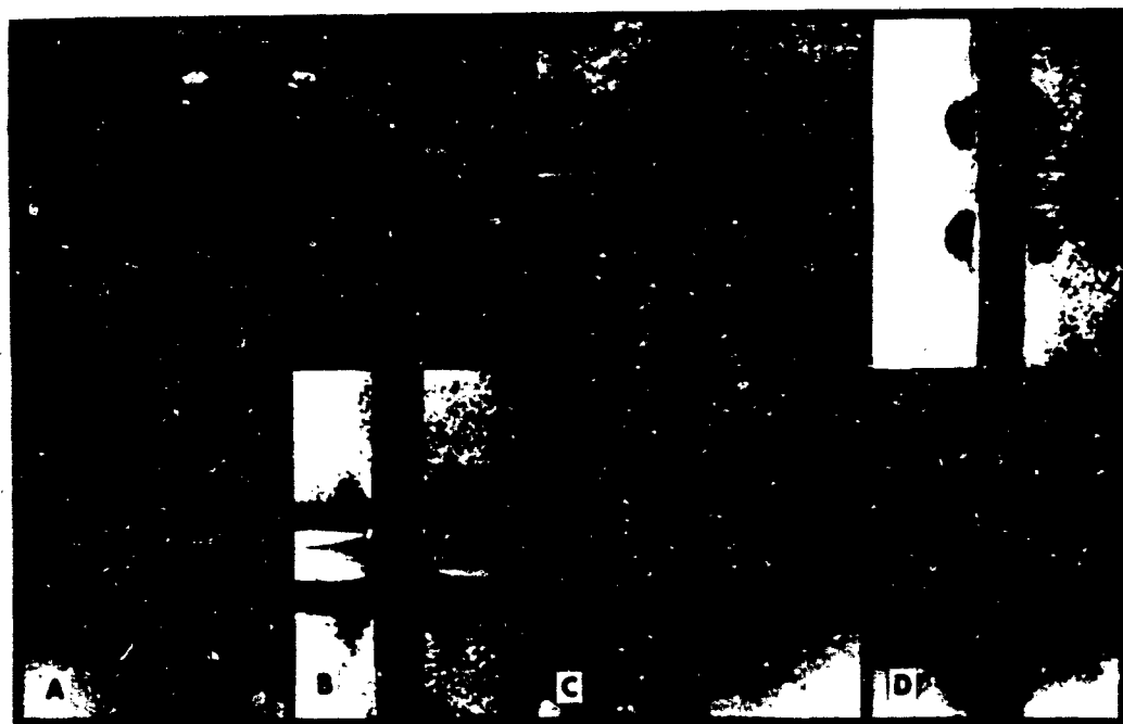
FIG. 1. The effect of various reagents on the activity of PI (top row) and PII (bottom row) tested by the modified cross-streak method. A, Trypsin (1.0%); B, Antiserum (PBI/+); C, \text{FeCl}_3 (0.01 M) all assayed on BAB plus 0.01 M \text{Ca}^{++} ; D, \text{CaCl}_2 (1.0 M) assayed on BAB containing 0.001 M \text{Fe}^{+++} in the top agar layer.
