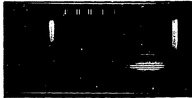
Figure 15. Flame Spectrum of Solid Rocket Showing Wide Bands of Polyatomic Species.
