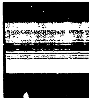
Figure 9. Spectrum of CROW Solid Ramjet Flame.
