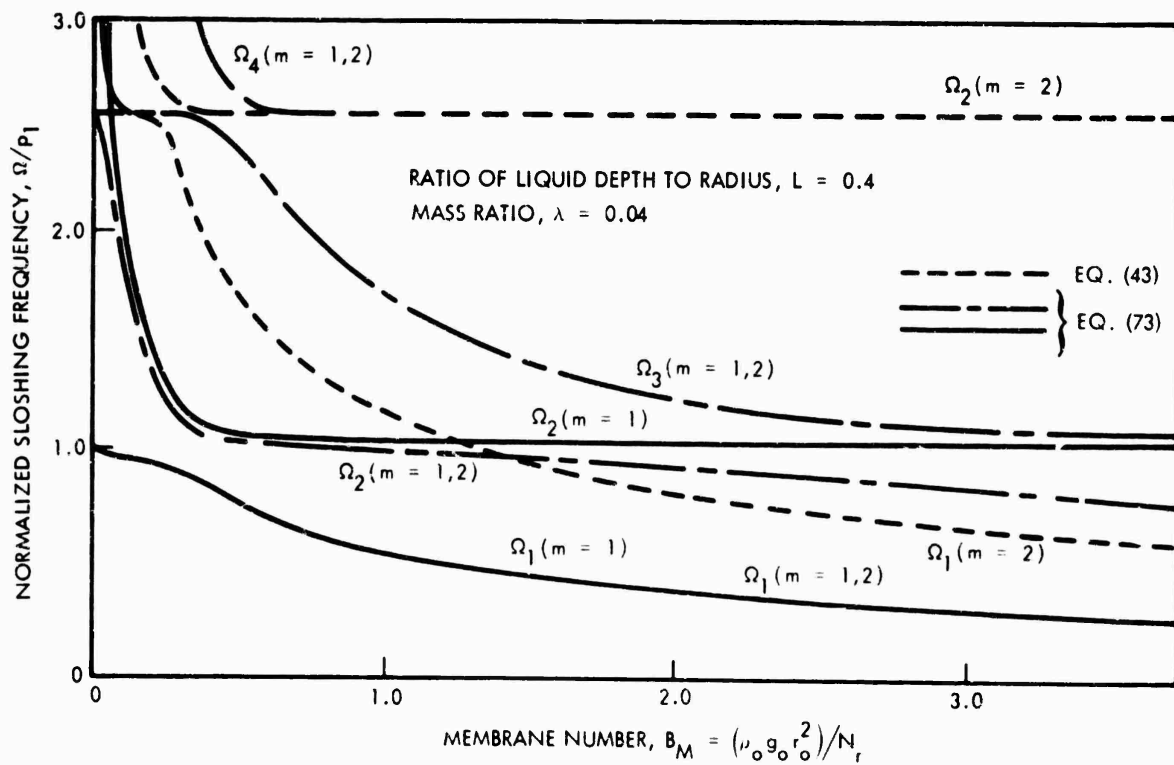
Fig. 3 Frequencies Computed From Eqs. (73) and (43), With Bond Number 1.0
