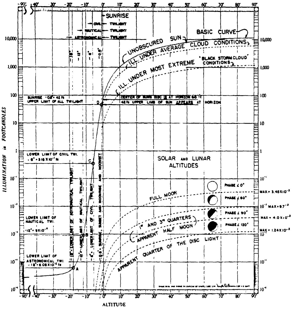
Figure 4. Total light of celestial bodies.
