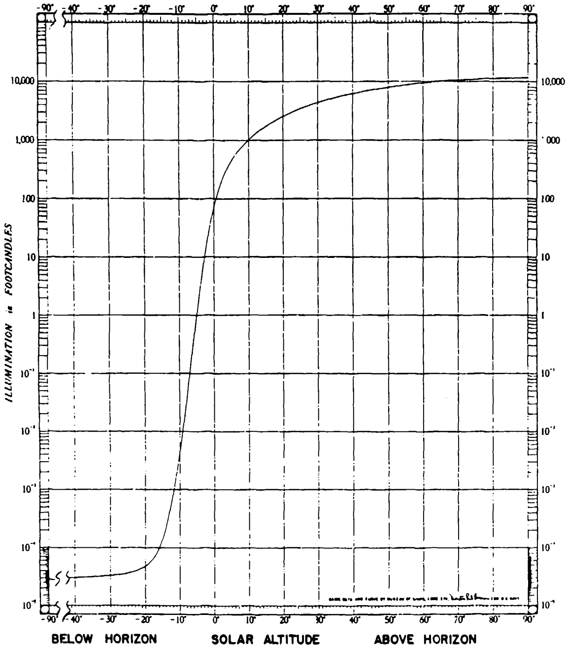
Figure 1. Basic Curve - Illumination in Footcandles Corresponding to Sun's Altitude
