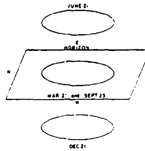
Figure 10. Observer in the North Pole.
