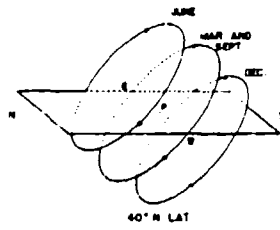
Figure 8. Observer in 40° N latitude.
