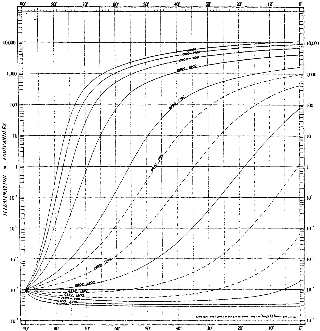
Each curve is for a given hour of LOCAL APPARENT TIME as shown
