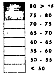
SOUTHEAST ASIA MEAN DAILY MIN. TEMPERATURE MARCH
