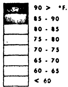
SOUTHEAST ASIA MEAN MONTHLY TEMPERATURE FEBRUARY
