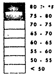
SOUTHEAST ASIA MEAN DAILY MIN. TEMPERATURE DECEMBER
