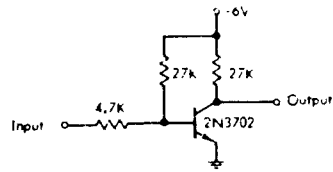
a) Level Converter
