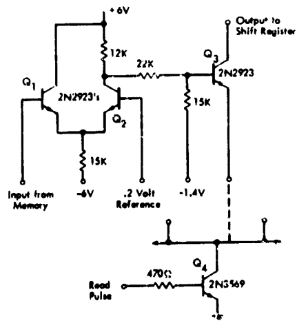
Fig. 6. High Gain Sense Amplifier
