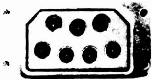
Figure 16. Connector corrosion and contamination
