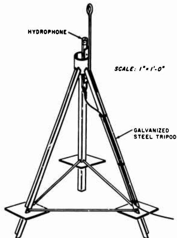
Figure 3. Hydrophone tripod
