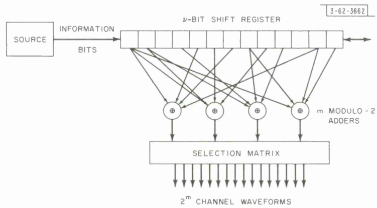
Fig. 2. Convolutional encoder.
