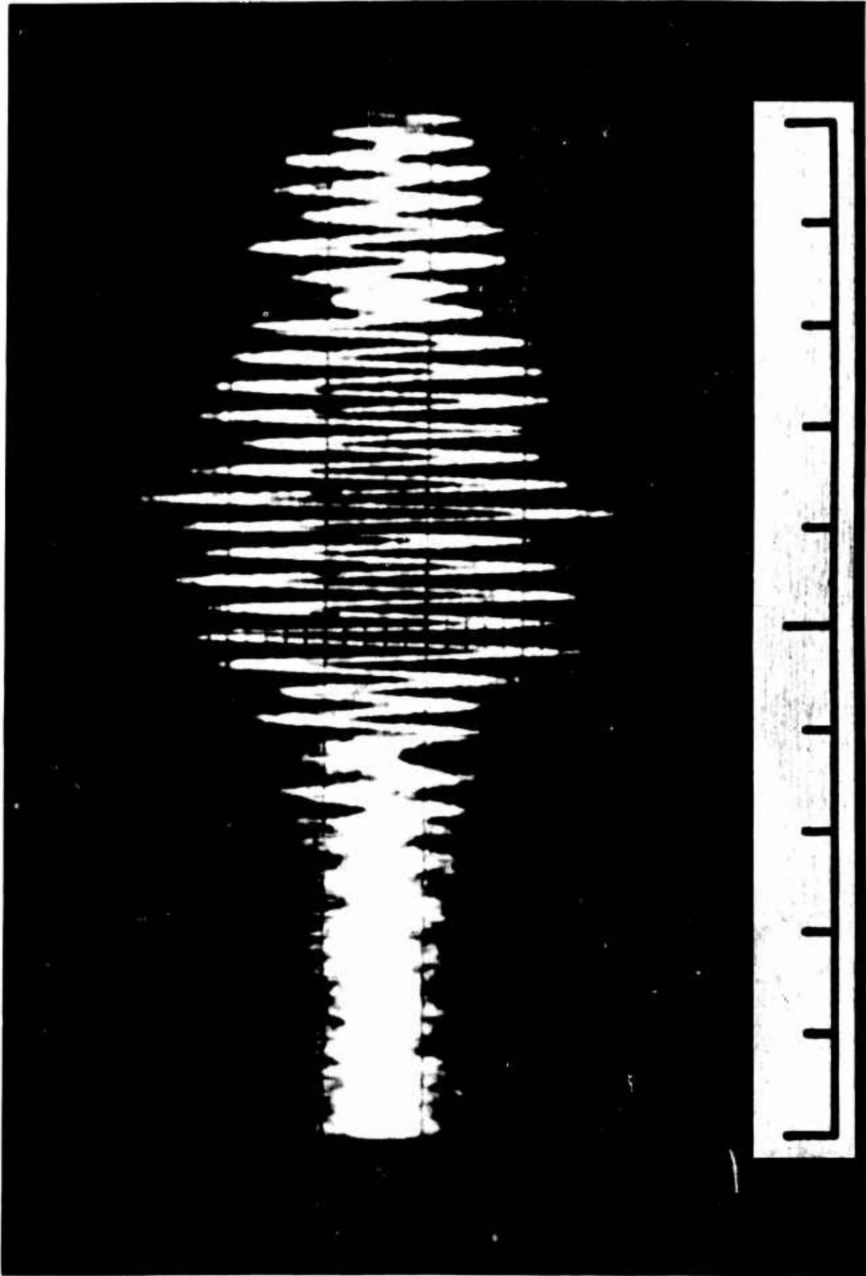
Figure 38. Oscilloscope: San Manual Mine, F-III Units, Transmitter at 10-2-b, Receiver at 10-2-e. Units Parallel, Offset, Towards Each Other. Horizontal scale: 3.17 msec/division. Vertical scale: 0.2 v/division.
