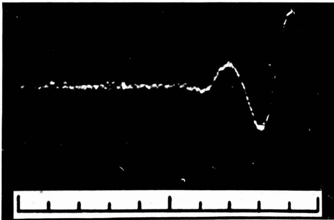
b. Expanded Arrival; Central Graticule Line is 5 Milliseconds. Spurious Sound in Figure "a" is Longer in Existence. Horizontal scale: 0.2 msec/division Vertical scale: 0.1 v/division
