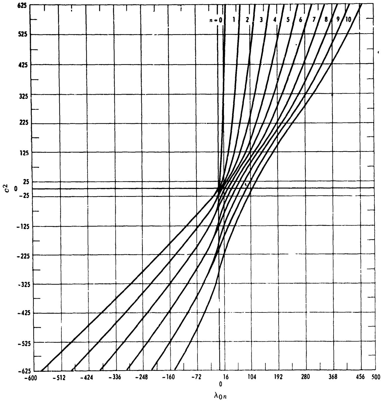
Figure - The Eigenvalues \lambda_{0n} for n = 0 (1) 10 and -625 \leq c^2 < 625
